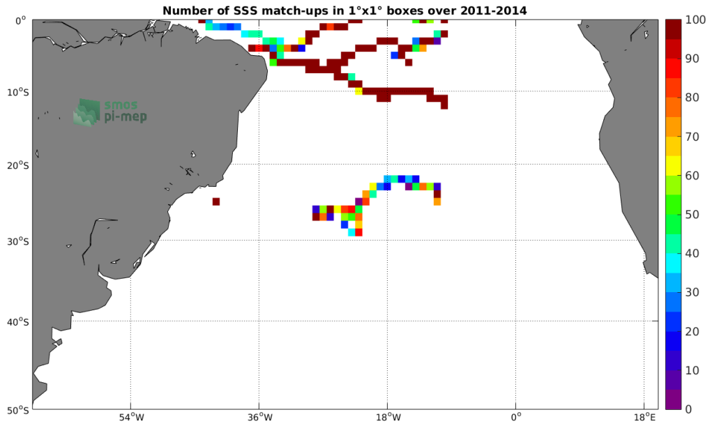
Figure 3: Number of SSS match-ups between Surface drifters SSS and the Aquarius-L4-IPRC-V5-MONTHLY SSS product for the South Atlantic Ocean Pi-MEP region over 1^\circ \times 1^\circ boxes and for the full satellite product period.
