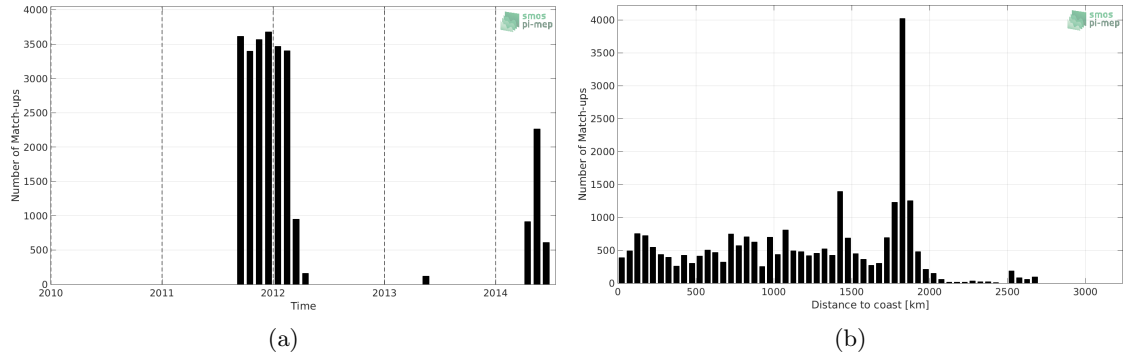
Figure 1: Number of match-ups between Surface drifters and Aquarius-L4-IPRC-V5-MONTHLY SSS as a function of time (a) and as function of the distance to coast (b) over the South Atlantic Ocean Pi-MEP region and for the full satellite product period.
