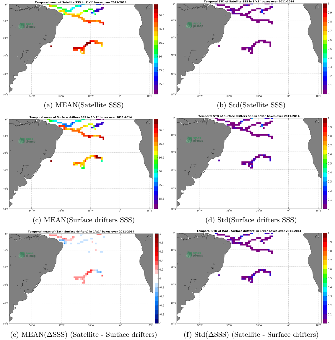
Figure 5: Temporal mean (left) and Std (right) of SSS from Aquarius-L4-IPRC-V5-MONTHLY (top), Surface drifters (middle), and of \Delta SSS (Satellite - Surface drifters). Only match-up pairs are used to generate these maps.
