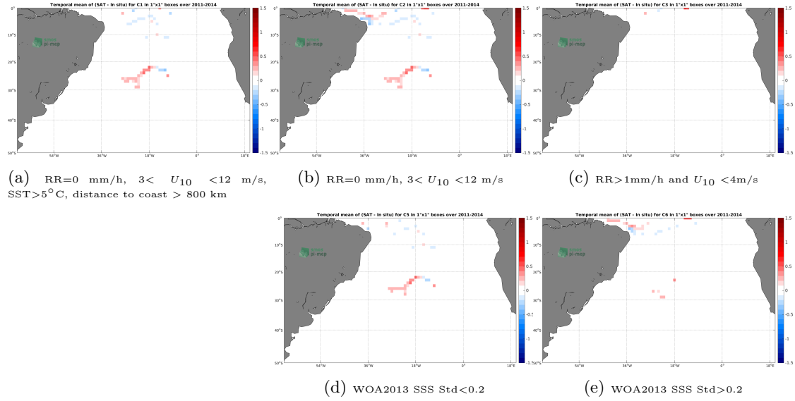
Figure 11: Temporal mean gridded over spatial boxes of size 1^\circ \times 1^\circ of \Delta SSS (Aquarius-L4-IPRC-V5-MONTHLY - Surface drifters) for 5 different subdatasets corresponding to: RR=0 mm/h, 3 < U_{10} < 12 m/s, SST > 5^\circ\text{C} , distance to coast > 800 km (a), RR=0 mm/h, 3 < U_{10} < 12 m/s (b), RR > 1 mm/h and U_{10} < 4 m/s (c), WOA2013 SSS Std < 0.2 (d), WOA2013 SSS Std > 0.2 (e).
