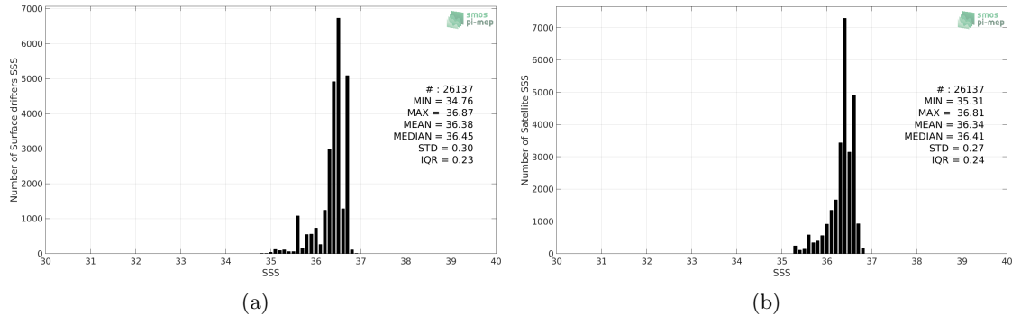
Figure 2: Histograms of SSS from Surface drifters (a) and Aquarius-L4-IPRC-V5-MONTHLY (b) considering all match-up pairs per bins of 0.1 over the South Atlantic Ocean Pi-MEP region and for the full satellite product period.
