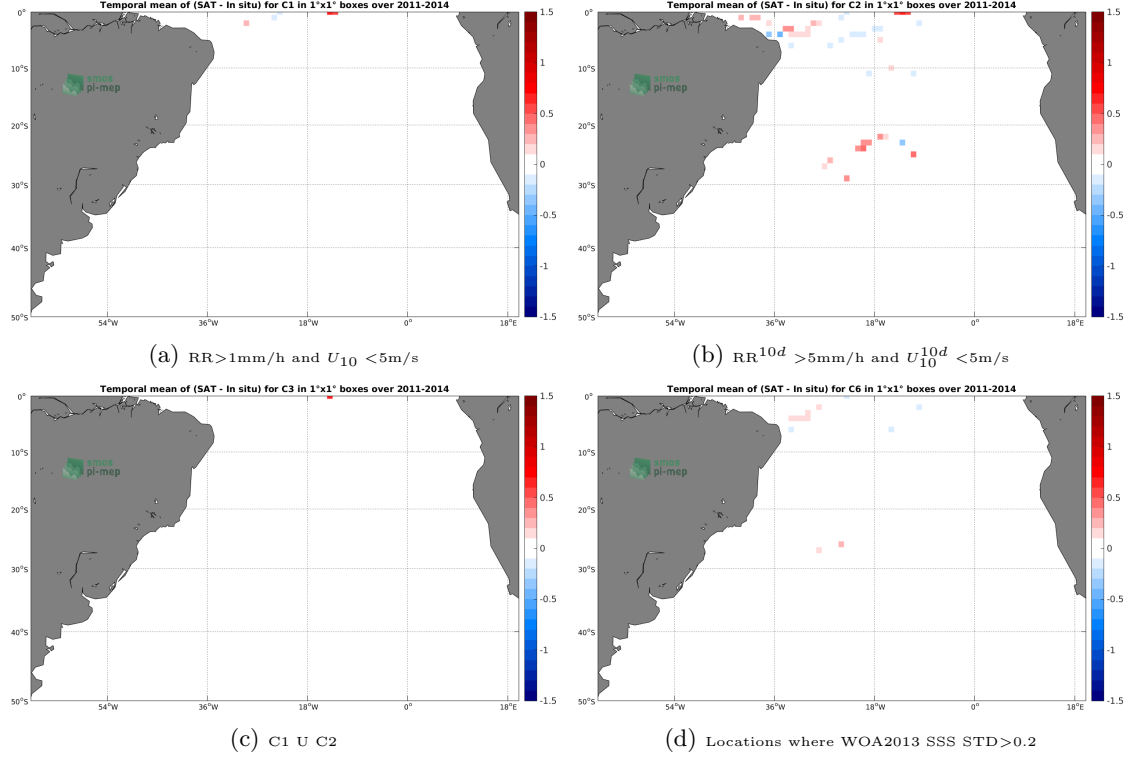
Figure 11: Temporal mean gridded over spatial boxes of size 1^\circ \times 1^\circ of \Delta SSS (Aquarius-L4-IPRC-V5-MONTHLY - Surface drifters) for 4 different subdatasets corresponding to: RR > 1mm/h and U_{10} < 5\text{m/s} (a), RR^{10d} > 5\text{mm/h} and U_{10}^{10d} < 5\text{m/s} (b), C1 U C2 (c), Locations where WOA2013 SSS STD > 0.2 (d).
