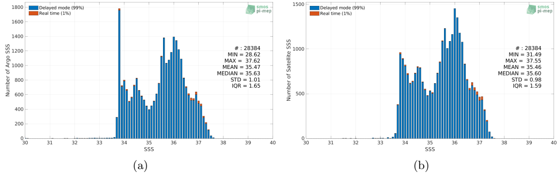
Figure 2: Histograms of SSS from Argo (a) and Aquarius SSS L4 OI v5 - Monthly (IPRC) (b) considering all match-up pairs per bins of 0.1 over the South Atlantic Ocean Pi-MEP region and for the full satellite product period.
