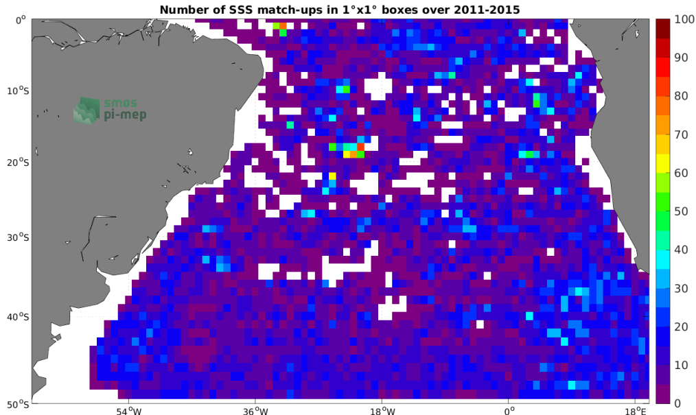
Figure 4: Number of SSS match-ups between Argo SSS and the Aquarius SSS L4 OI v5 - Monthly (IPRC) SSS product for the South Atlantic Ocean Pi-MEP region over 1^\circ \times 1^\circ boxes and for the full satellite product period.
