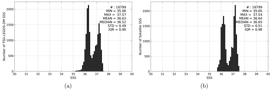
Figure 2: Histograms of SSS from TSG-LEGOS-DM (a) and Aquarius-L4-IPRC-V4-MONTHLY (b) considering all match-up pairs per bins of 0.1 over the South Atlantic Ocean Pi-MEP region and for the full satellite product period.
