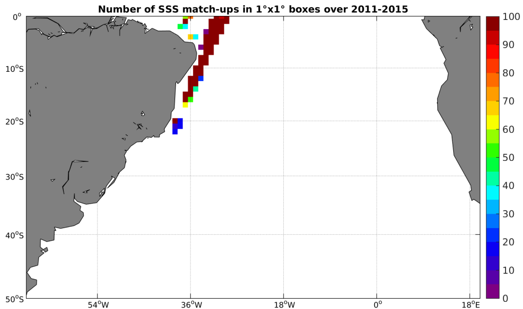
Figure 4: Number of SSS match-ups between TSG-LEGOS-DM SSS and the Aquarius-L4-IPRC-V4-MONTHLY SSS product for the South Atlantic Ocean Pi-MEP region over 1^\circ \times 1^\circ boxes and for the full satellite product period.
