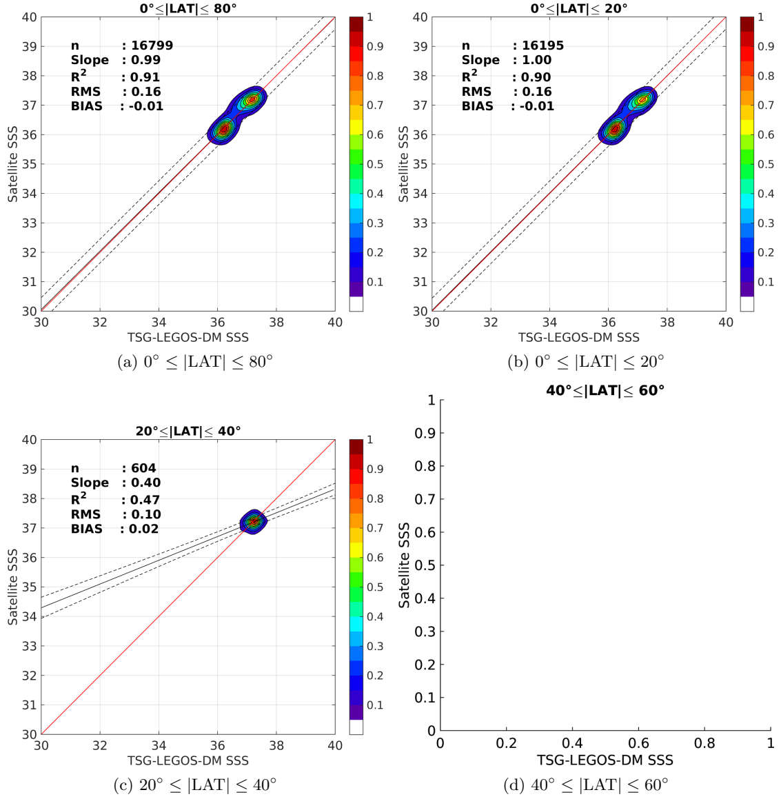
Figure 9: Contour maps of the concentration of Aquarius-L4-IPRC-V4-MONTHLY SSS (y-axis) versus TSG-LEGOS-DM SSS (x-axis) at match-up pairs for different latitude bands. For each plot, the red line shows x=y . The black thin and dashed lines indicate a linear fit through the data cloud and the \pm 95\% confidence levels, respectively. The number match-up pairs n , the slope and R^2 coefficient of the linear fit, the root mean square (RMS) and the mean bias between satellite and in situ data are indicated for each latitude band in each plots.
