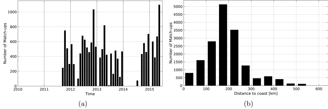
Figure 1: Number of match-ups between TSG-LEGOS-DM and Aquarius-L4-IPRC-V4-MONTHLY SSS as a function of time (a) and as function of the distance to coast (b) over the South Atlantic Ocean Pi-MEP region and for the full satellite product period.
