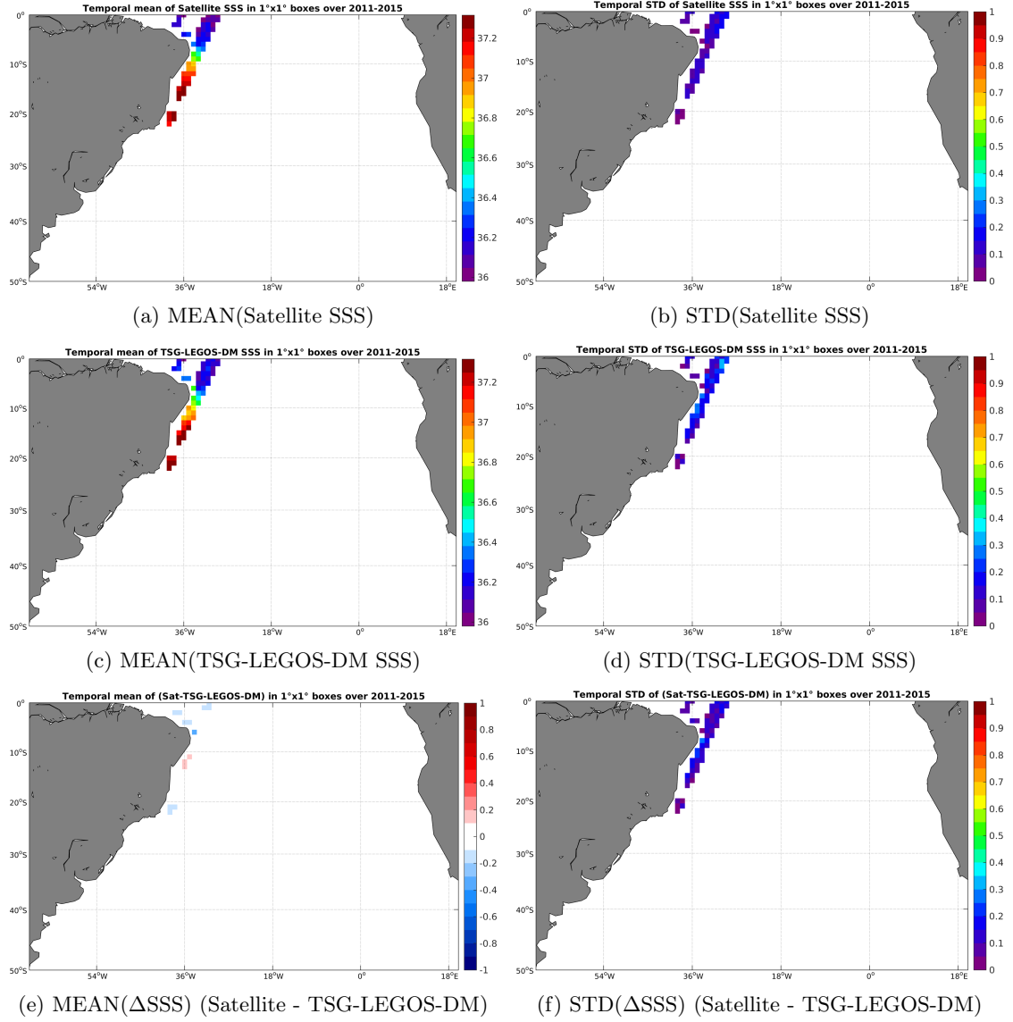
Figure 6: Temporal mean (left) and STD (right) of SSS from Aquarius-L4-IPRC-V4-MONTHLY (top), TSG-LEGOS-DM (middle), and of \Delta SSS (Satellite - TSG-LEGOS-DM). Only match-up pairs are used to generate these maps.
