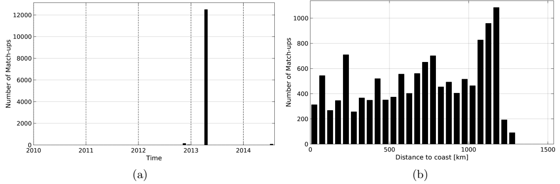
Figure 1: Number of match-ups between TSG-GOSUD-Sailing-ship and Aquarius-L4-IPRC-V4-MONTHLY SSS as a function of time (a) and as function of the distance to coast (b) over the South Atlantic Ocean Pi-MEP region and for the full satellite product period.
