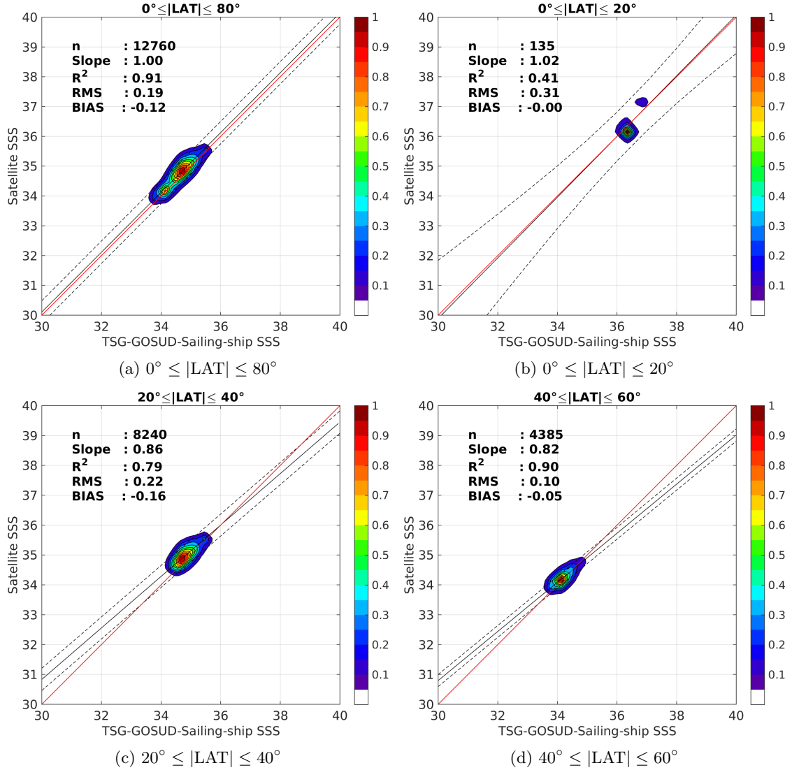
Figure 9: Contour maps of the concentration of Aquarius-L4-IPRC-V4-MONTHLY SSS (y-axis) versus TSG-GOSUD-Sailing-ship SSS (x-axis) at match-up pairs for different latitude bands. For each plot, the red line shows x=y . The black thin and dashed lines indicate a linear fit through the data cloud and the \pm 95\% confidence levels, respectively. The number match-up pairs n , the slope and R^2 coefficient of the linear fit, the root mean square (RMS) and the mean bias between satellite and in situ data are indicated for each latitude band in each plots.
