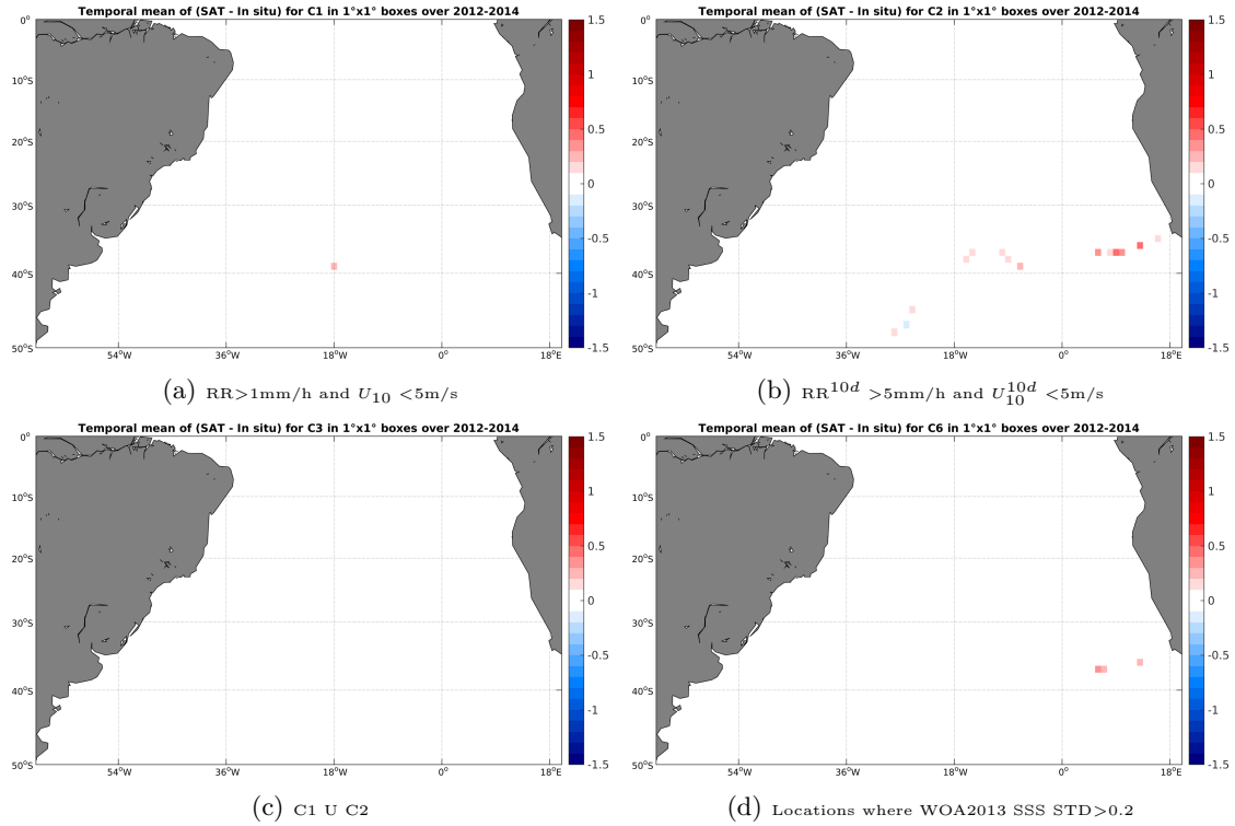
Figure 12: Temporal mean gridded over spatial boxes of size 1^\circ \times 1^\circ of \Delta SSS (Aquarius-L4-IPRC-V4-MONTHLY - TSG-GOSUD-Sailing-ship) for 4 different subdatasets corresponding to: RR > 1\text{mm/h} and U_{10} < 5\text{m/s} (a), RR^{10d} > 5\text{mm/h} and U_{10}^{10d} < 5\text{m/s} (b), C1 U C2 (c), Locations where WOA2013 SSS STD > 0.2 (d).
