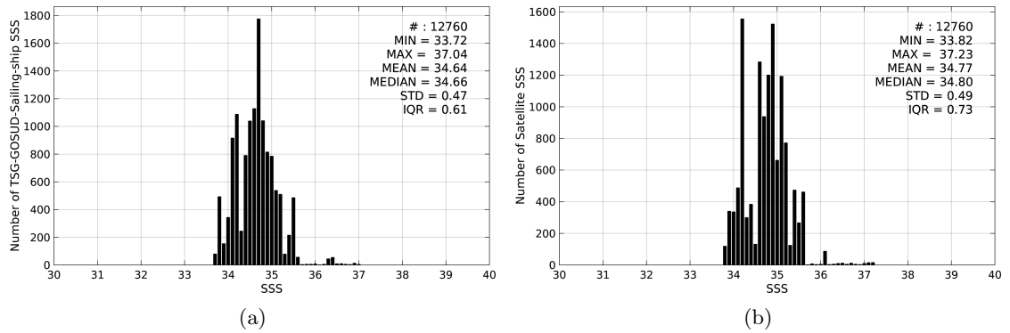
Figure 2: Histograms of SSS from TSG-GOSUD-Sailing-ship (a) and Aquarius-L4-IPRC-V4-MONTHLY (b) considering all match-up pairs per bins of 0.1 over the South Atlantic Ocean Pi-MEP region and for the full satellite product period.
