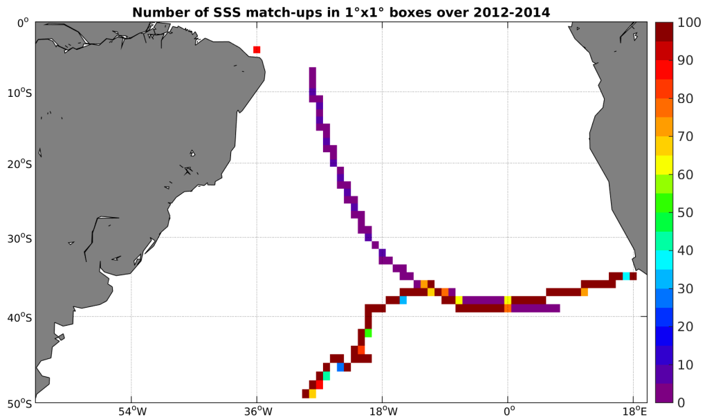
Figure 4: Number of SSS match-ups between TSG-GOSUD-Sailing-ship SSS and the Aquarius-L4-IPRC-V4-MONTHLY SSS product for the South Atlantic Ocean Pi-MEP region over 1^\circ \times 1^\circ boxes and for the full satellite product period.
