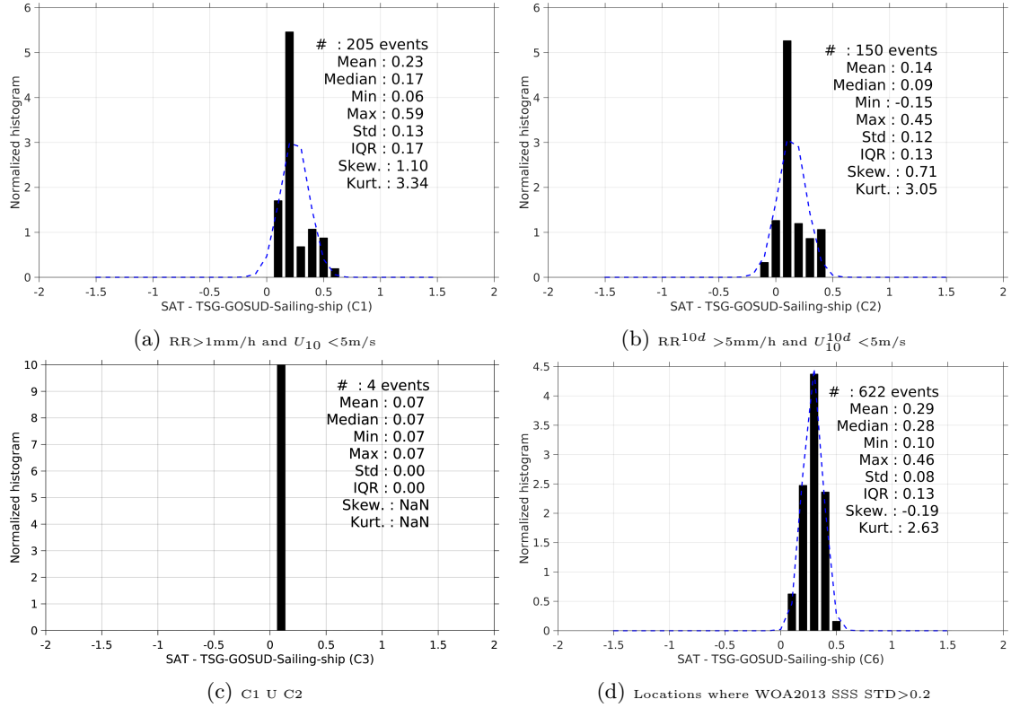
Figure 13: Normalized histogram of \Delta SSS (Aquarius-L4-IPRC-V4-MONTHLY - TSG-GOSUD-Sailing-ship) for 6 different subdatasets corresponding to: RR > 1\text{mm/h} and U_{10} < 5\text{m/s} (a), RR^{10d} > 5\text{mm/h} and U_{10}^{10d} < 5\text{m/s} (b), C1 U C2 (c), Locations where WOA2013 SSS STD > 0.2 (d).
