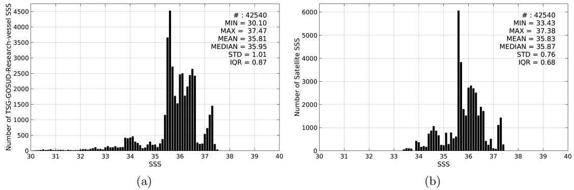
Figure 2: Histograms of SSS from TSG-GOSUD-Research-vessel (a) and Aquarius-L4-IPRC-V4-MONTHLY (b) considering all match-up pairs per bins of 0.1 over the South Atlantic Ocean Pi-MEP region and for the full satellite product period.
