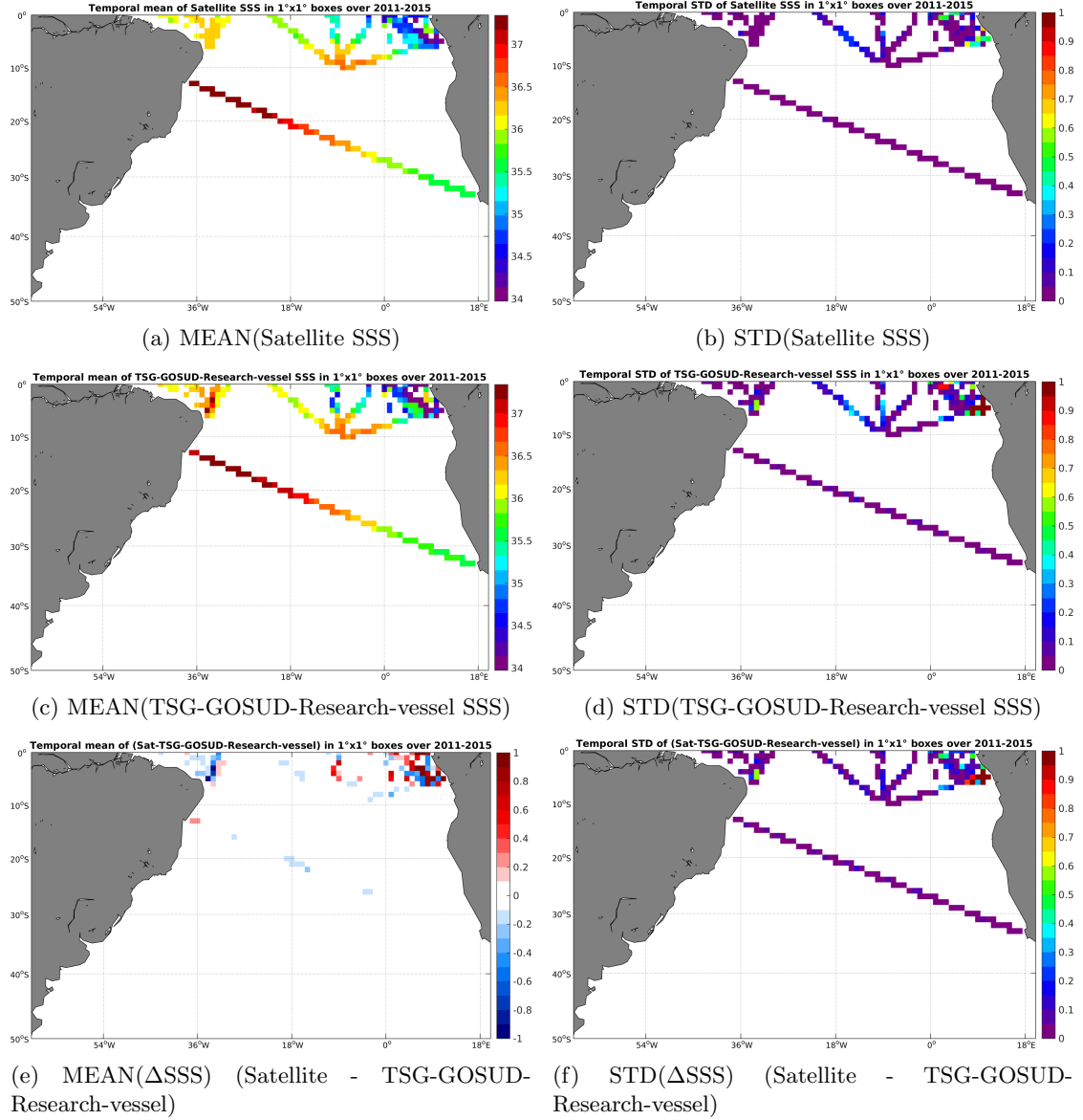
Figure 6: Temporal mean (left) and STD (right) of SSS from Aquarius-L4-IPRC-V4-MONTHLY (top), TSG-GOSUD-Research-vessel (middle), and of \Delta SSS (Satellite - TSG-GOSUD-Research-vessel). Only match-up pairs are used to generate these maps.
