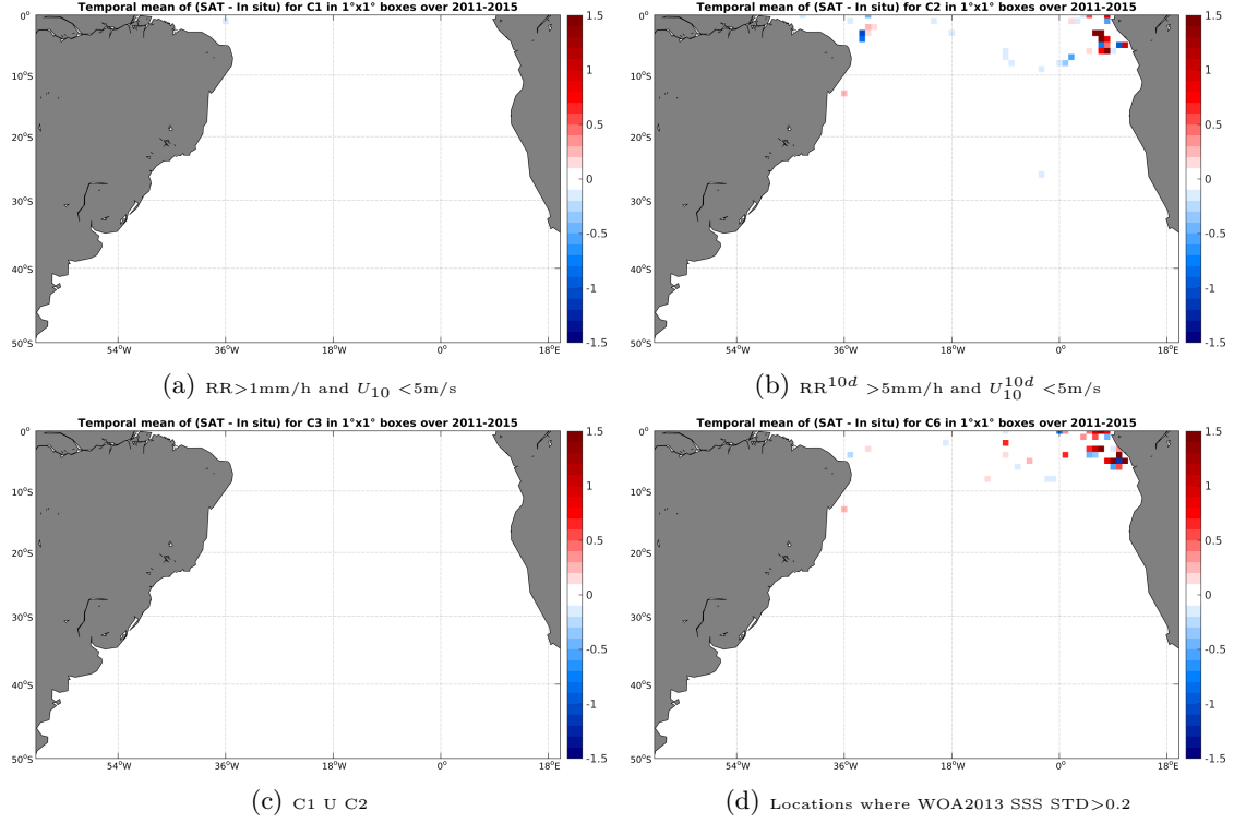
Figure 12: Temporal mean gridded over spatial boxes of size 1^\circ \times 1^\circ of \Delta SSS (Aquarius-L4-IPRC-V4-MONTHLY - TSG-GOSUD-Research-vessel) for 4 different subdatasets corresponding to: RR > 1\text{mm/h} and U_{10} < 5\text{m/s} (a), RR^{10d} > 5\text{mm/h} and U_{10}^{10d} < 5\text{m/s} (b), C1 U C2 (c), Locations where WOA2013 SSS STD > 0.2 (d).
