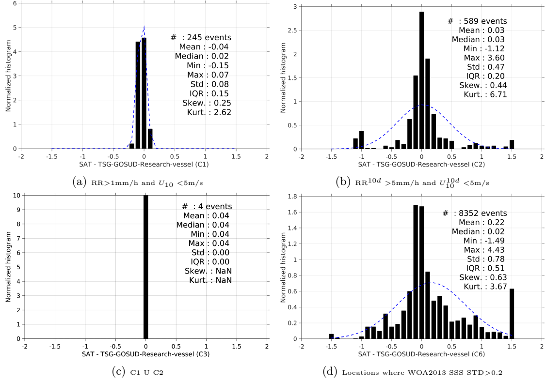
Figure 13: Normalized histogram of \Delta SSS (Aquarius-L4-IPRC-V4-MONTHLY - TSG-GOSUD-Research-vessel) for 6 different subdatasets corresponding to: RR > 1mm/h and U_{10} < 5\text{m/s} (a), RR^{10d} > 5\text{mm/h} and U_{10}^{10d} < 5\text{m/s} (b), C1 U C2 (c), Locations where WOA2013 SSS STD > 0.2 (d).
