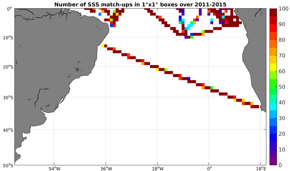
Figure 4: Number of SSS match-ups between TSG-GOSUD-Research-vessel SSS and the Aquarius-L4-IPRC-V4-MONTHLY SSS product for the South Atlantic Ocean Pi-MEP region over 1^\circ \times 1^\circ boxes and for the full satellite product period.
