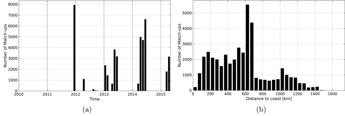
Figure 1: Number of match-ups between TSG-GOSUD-Research-vessel and Aquarius-L4-IPRC-V4-MONTHLY SSS as a function of time (a) and as function of the distance to coast (b) over the South Atlantic Ocean Pi-MEP region and for the full satellite product period.
