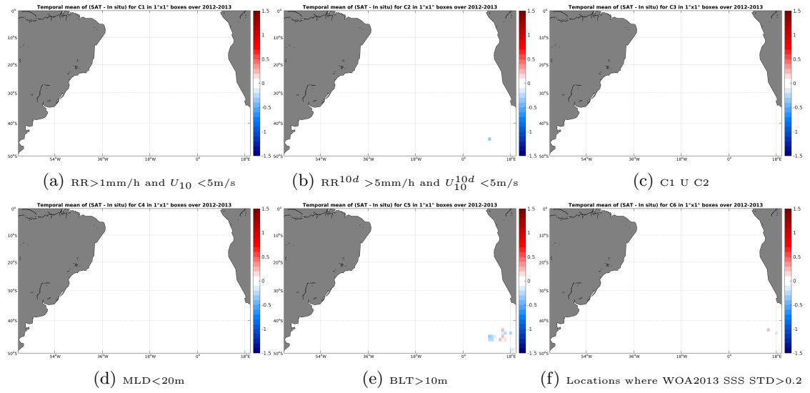
Figure 12: Temporal mean gridded over spatial boxes of size 1^\circ \times 1^\circ of \Delta SSS (Aquarius-L4-IPRC-V4-MONTHLY - Sea mammals) for 6 different subdatasets corresponding to: RR > 1\text{mm/h} and U_{10} < 5\text{m/s} (a), RR^{10d} > 5\text{mm/h} and U_{10}^{10d} < 5\text{m/s} (b), C1 U C2 (c), MLD < 20\text{m} (d), BLT > 10\text{m} (e), Locations where WOA2013 SSS STD > 0.2 (f).
