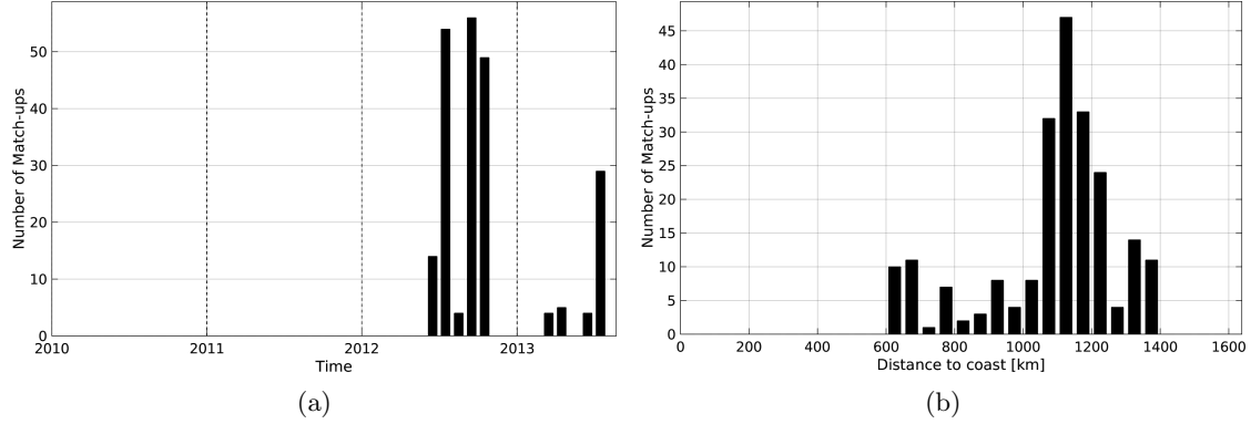
Figure 1: Number of match-ups between Sea mammals and Aquarius-L4-IPRC-V4-MONTHLY SSS as a function of time (a) and as function of the distance to coast (b) over the South Atlantic Ocean Pi-MEP region and for the full satellite product period.
