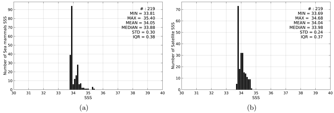
Figure 2: Histograms of SSS from Sea mammals (a) and Aquarius-L4-IPRC-V4-MONTHLY (b) considering all match-up pairs per bins of 0.1 over the South Atlantic Ocean Pi-MEP region and for the full satellite product period.
