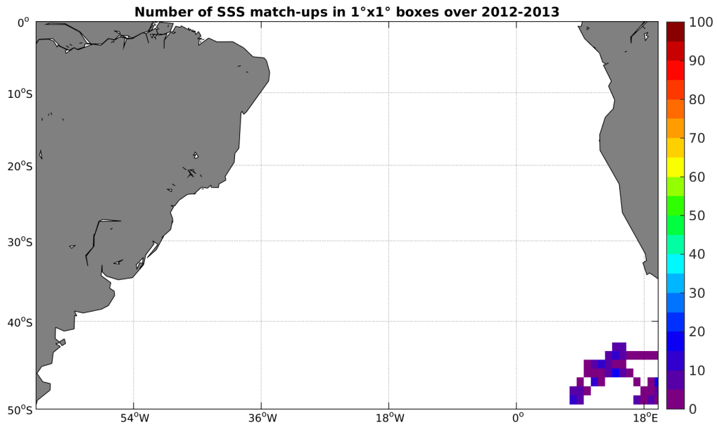
Figure 4: Number of SSS match-ups between Sea mammals SSS and the Aquarius-L4-IPRC-V4-MONTHLY SSS product for the South Atlantic Ocean Pi-MEP region over 1^\circ \times 1^\circ boxes and for the full satellite product period.
