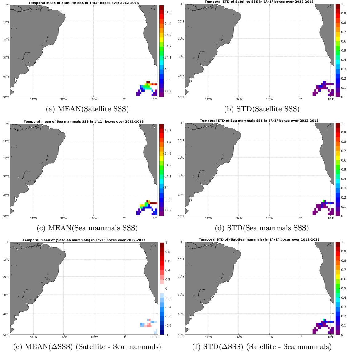
Figure 6: Temporal mean (left) and STD (right) of SSS from Aquarius-L4-IPRC-V4-MONTHLY (top), Sea mammals (middle), and of \Delta SSS (Satellite - Sea mammals). Only match-up pairs are used to generate these maps.
