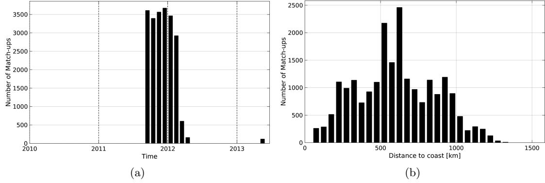
Figure 1: Number of match-ups between Surface drifters and Aquarius-L4-IPRC-V4-MONTHLY SSS as a function of time (a) and as function of the distance to coast (b) over the South Atlantic Ocean Pi-MEP region and for the full satellite product period.
