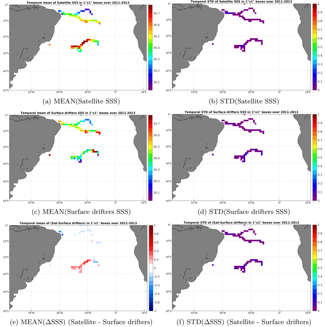
Figure 5: Temporal mean (left) and STD (right) of SSS from Aquarius-L4-IPRC-V4-MONTHLY (top), Surface drifters (middle), and of \Delta SSS (Satellite - Surface drifters). Only match-up pairs are used to generate these maps.
