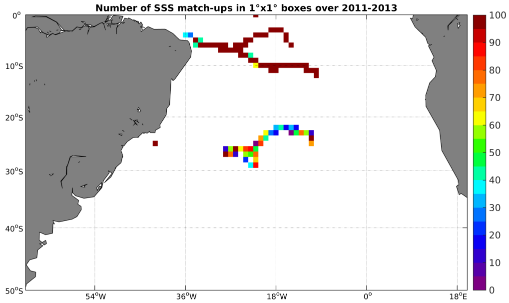
Figure 3: Number of SSS match-ups between Surface drifters SSS and the Aquarius-L4-IPRC-V4-MONTHLY SSS product for the South Atlantic Ocean Pi-MEP region over 1^\circ \times 1^\circ boxes and for the full satellite product period.
