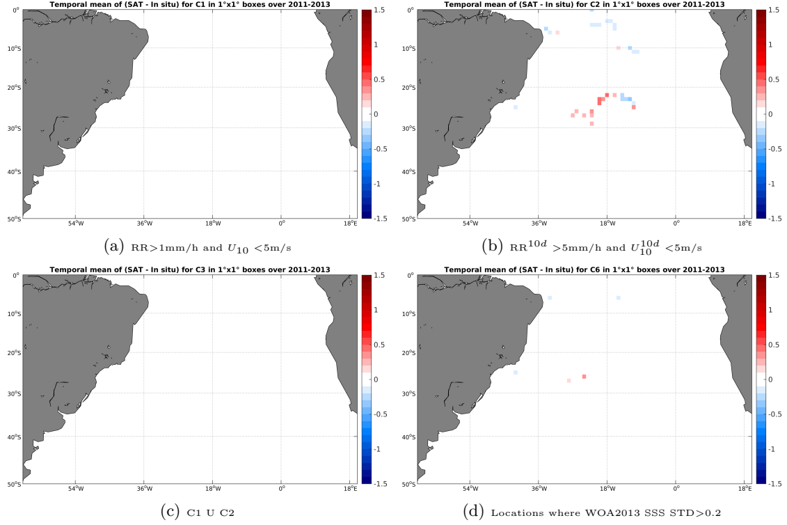
Figure 11: Temporal mean gridded over spatial boxes of size 1^\circ \times 1^\circ of \Delta SSS (Aquarius-L4-IPRC-V4-MONTHLY - Surface drifters) for 4 different subdatasets corresponding to: RR > 1 mm/h and U_{10} < 5 m/s (a), RR 10d > 5 mm/h and U_{10}^{10d} < 5 m/s (b), C1 U C2 (c), Locations where WOA2013 SSS STD > 0.2 (d).
