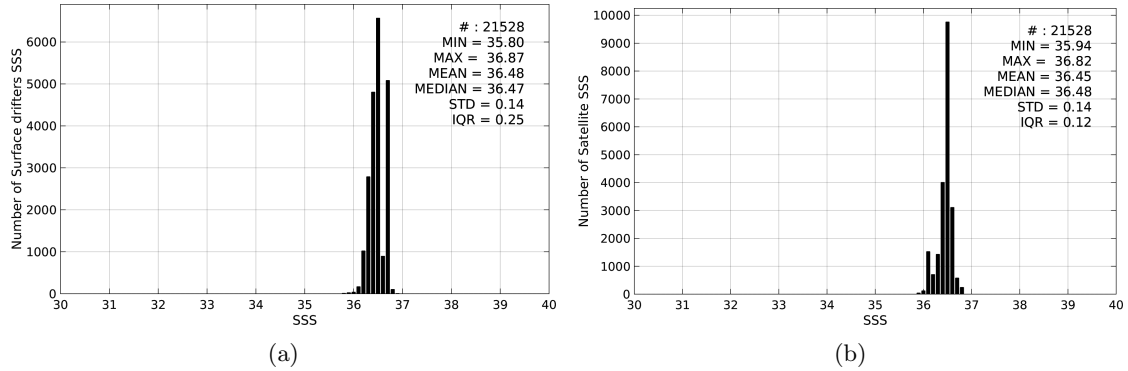
Figure 2: Histograms of SSS from Surface drifters (a) and Aquarius-L4-IPRC-V4-MONTHLY (b) considering all match-up pairs per bins of 0.1 over the South Atlantic Ocean Pi-MEP region and for the full satellite product period.
