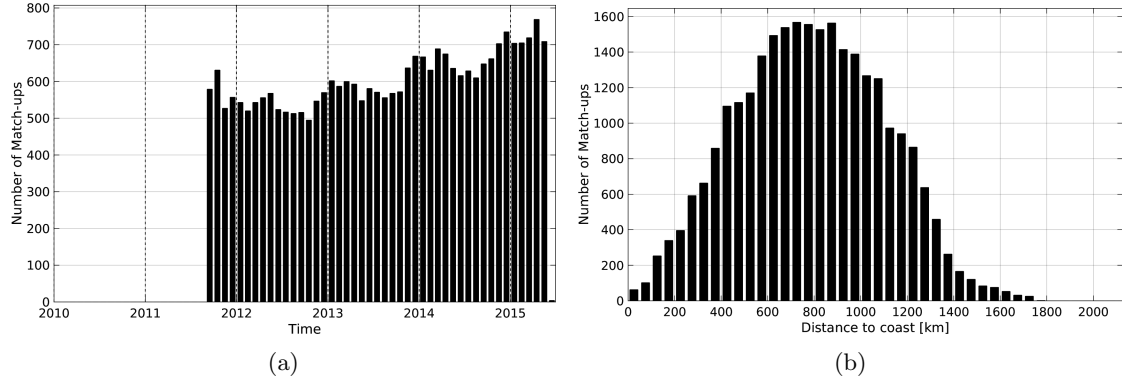
Figure 1: Number of match-ups between Argo and Aquarius-L4-IPRC-V4-MONTHLY SSS as a function of time (a) and as function of the distance to coast (b) over the South Atlantic Ocean Pi-MEP region and for the full satellite product period.
