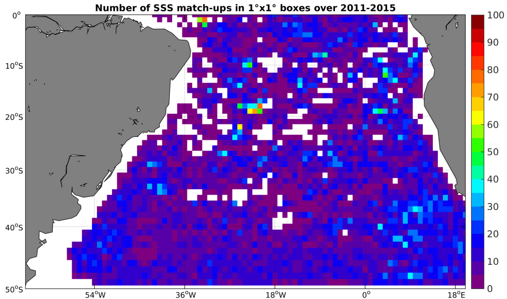
Figure 4: Number of SSS match-ups between Argo SSS and the Aquarius-L4-IPRC-V4-MONTHLY SSS product for the South Atlantic Ocean Pi-MEP region over 1^\circ \times 1^\circ boxes and for the full satellite product period.
