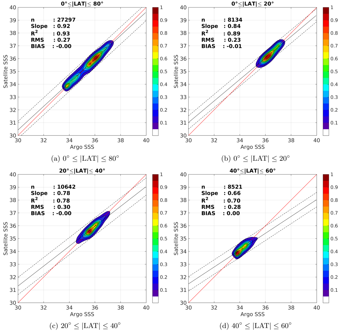
Figure 9: Contour maps of the concentration of Aquarius-L4-IPRC-V4-MONTHLY SSS (y-axis) versus Argo SSS (x-axis) at match-up pairs for different latitude bands. For each plot, the red line shows x=y . The black thin and dashed lines indicate a linear fit through the data cloud and the \pm 95\% confidence levels, respectively. The number match-up pairs n , the slope and R^2 coefficient of the linear fit, the root mean square (RMS) and the mean bias between satellite and in situ data are indicated for each latitude band in each plots.
