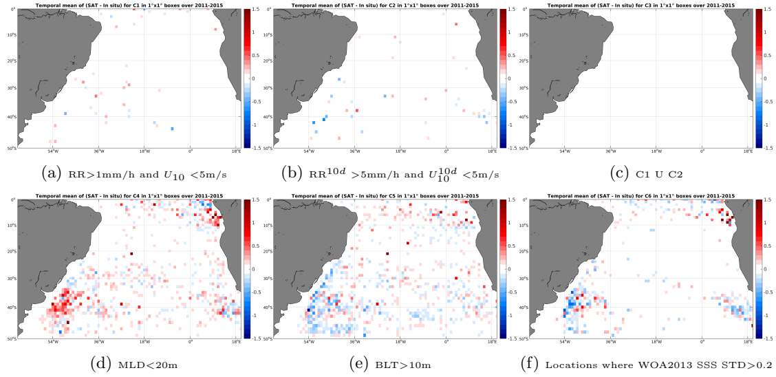
Figure 12: Temporal mean gridded over spatial boxes of size 1^\circ \times 1^\circ of \Delta SSS (Aquarius-L4-IPRC-V4-MONTHLY - Argo) for 6 different subdatasets corresponding to: RR > 1\text{mm/h} and U_{10} < 5\text{m/s} (a), RR^{10d} > 5\text{mm/h} and U_{10}^{10d} < 5\text{m/s} (b), C1 U C2 (c), MLD < 20\text{m} (d), BLT > 10\text{m} (e), Locations where WOA2013 SSS STD > 0.2 (f).
