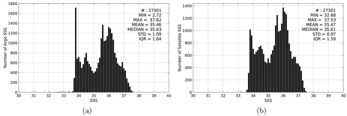
Figure 2: Histograms of SSS from Argo (a) and Aquarius-L4-IPRC-V4-MONTHLY (b) considering all match-up pairs per bins of 0.1 over the South Atlantic Ocean Pi-MEP region and for the full satellite product period.
