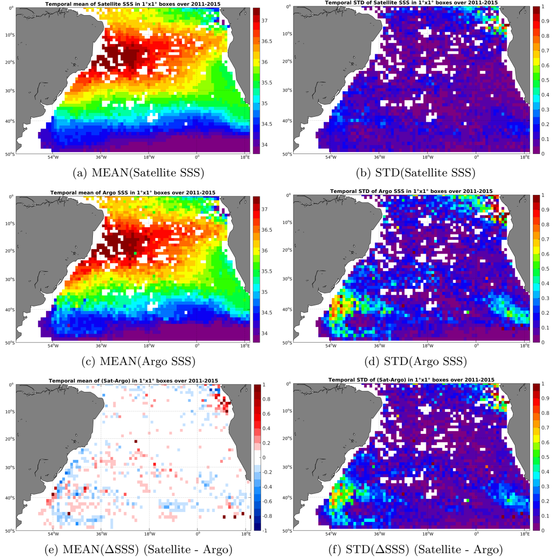
Figure 6: Temporal mean (left) and STD (right) of SSS from Aquarius-L4-IPRC-V4-MONTHLY (top), Argo (middle), and of \Delta SSS (Satellite - Argo). Only match-up pairs are used to generate these maps.
