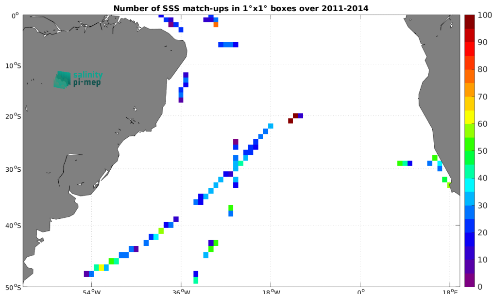
Figure 5: Number of SSS match-ups between TSG (SAMOS) SSS and the Aquarius SSS L3 OR v5 - 7-Day running (NASA-GSFC) SSS product for the South Atlantic Ocean Pi-MEP region over 1^\circ \times 1^\circ boxes and for the full satellite product period.
