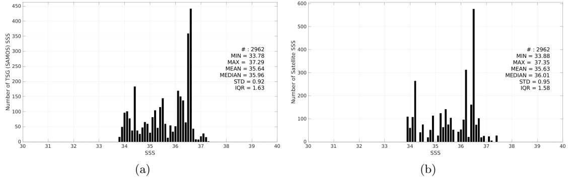
Figure 3: Histograms of SSS from TSG (SAMOS) (a) and Aquarius SSS L3 OR v5 - 7-Day running (NASA-GSFC) (b) considering all match-up pairs per bins of 0.1 over the South Atlantic Ocean Pi-MEP region and for the full satellite product period.
