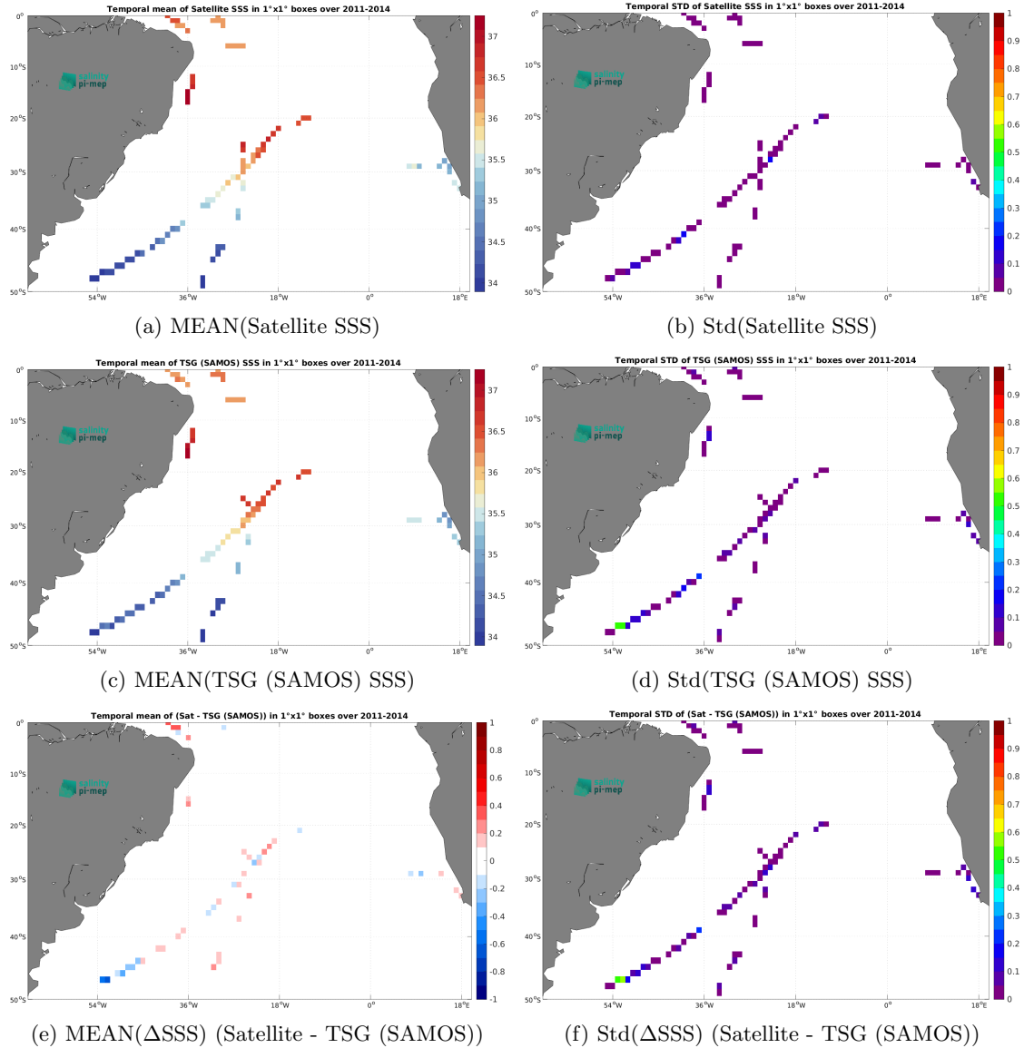
Figure 7: Temporal mean (left) and Std (right) of SSS from Aquarius SSS L3 OR v5 - 7-Day running (NASA-GSFC) (top), TSG (SAMOS) (middle), and of \Delta SSS (Satellite - TSG (SAMOS)). Only match-up pairs are used to generate these maps.
