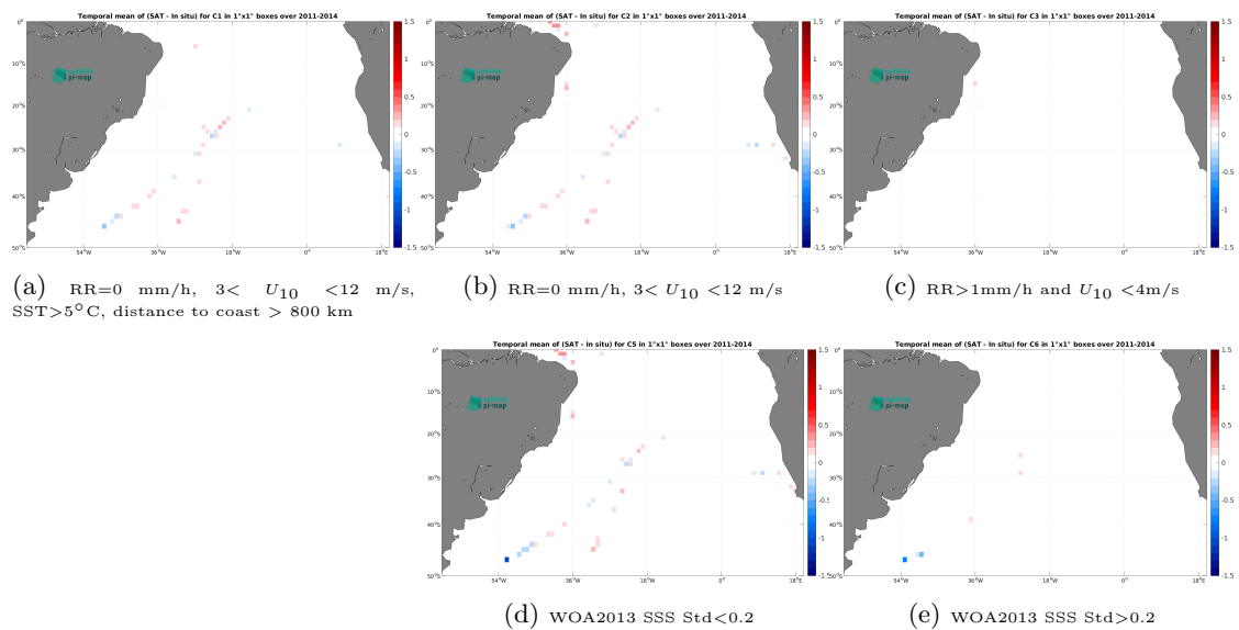
Figure 14: Temporal mean gridded over spatial boxes of size 1^\circ \times 1^\circ of \Delta\text{SSS} (Aquarius SSS L3 OR v5 - 7-Day running (NASA-GSFC) - TSG (SAMOS)) for 5 different subdatasets corresponding to:RR=0 mm/h, 3 < U_{10} < 12 m/s, SST >5^\circ\text{C} , distance to coast > 800 km (a), RR=0 mm/h, 3 < U_{10} < 12 m/s (b), RR >1 mm/h and U_{10} < 4 m/s (c), WOA2013 SSS Std <0.2 (d), WOA2013 SSS Std >0.2 (e).
