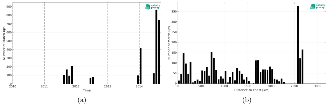
Figure 2: Number of match-ups between TSG (SAMOS) and Aquarius SSS L3 OR v5 - 7-Day running (NASA-GSFC) SSS as a function of time (a) and as function of the distance to coast (b) over the South Atlantic Ocean Pi-MEP region and for the full satellite product period.
