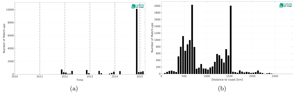
Figure 2: Number of match-ups between TSG (Polarstern) and Aquarius SSS L3 OR v5 - 7-Day running (NASA-GSFC) SSS as a function of time (a) and as function of the distance to coast (b) over the South Atlantic Ocean Pi-MEP region and for the full satellite product period.
