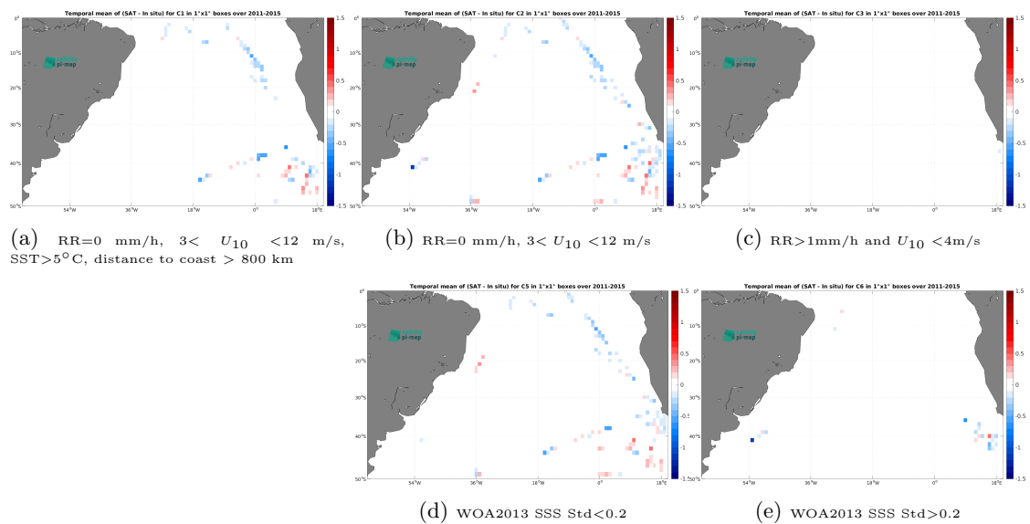
Figure 14: Temporal mean gridded over spatial boxes of size 1^\circ \times 1^\circ of \Delta SSS (Aquarius SSS L3 OR v5 - 7-Day running (NASA-GSFC) - TSG (Polarstern)) for 5 different subdatasets corresponding to:RR=0 mm/h, 3 < U_{10} < 12 m/s, SST >5^\circ\text{C} , distance to coast > 800 km (a), RR=0 mm/h, 3 < U_{10} < 12 m/s (b), RR >1 mm/h and U_{10} < 4 m/s (c), WOA2013 SSS Std <0.2 (d), WOA2013 SSS Std >0.2 (e).
