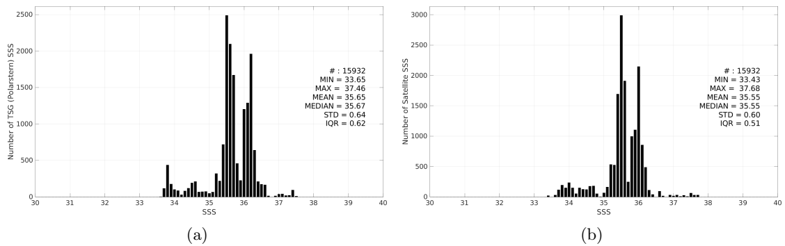
Figure 3: Histograms of SSS from TSG (Polarstern) (a) and Aquarius SSS L3 OR v5 - 7-Day running (NASA-GSFC) (b) considering all match-up pairs per bins of 0.1 over the South Atlantic Ocean Pi-MEP region and for the full satellite product period.
