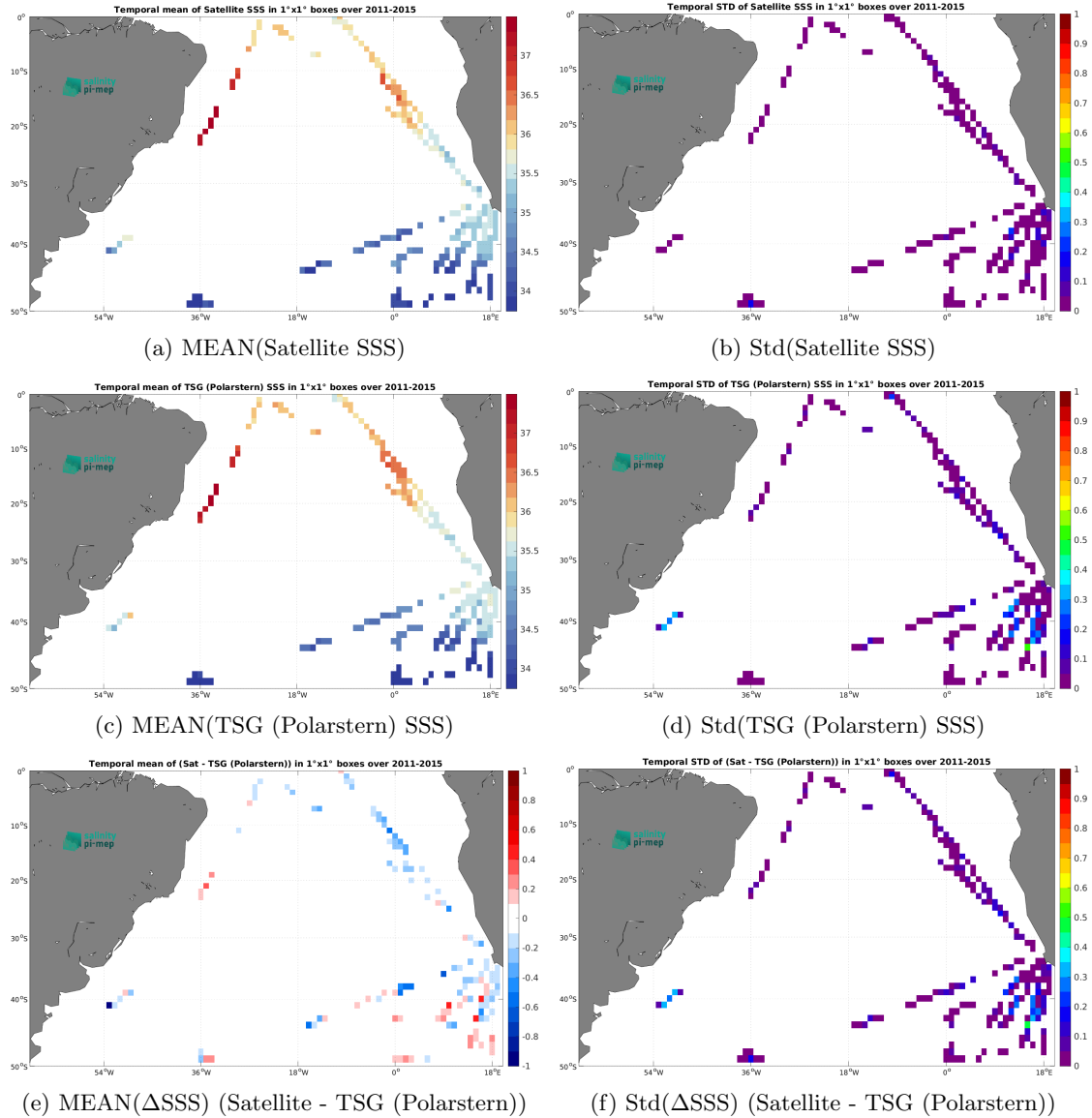
Figure 7: Temporal mean (left) and Std (right) of SSS from Aquarius SSS L3 OR v5 - 7-Day running (NASA-GSFC) (top), TSG (Polarstern) (middle), and of \Delta SSS (Satellite - TSG (Polarstern)). Only match-up pairs are used to generate these maps.
