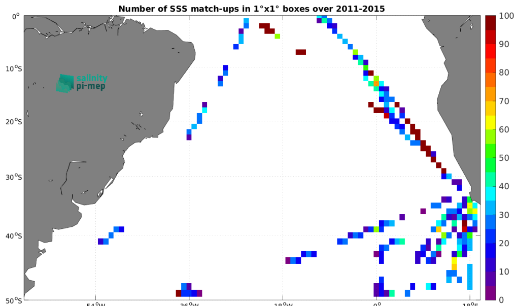
Figure 5: Number of SSS match-ups between TSG (Polarstern) SSS and the Aquarius SSS L3 OR v5 - 7-Day running (NASA-GSFC) SSS product for the South Atlantic Ocean Pi-MEP region over 1^\circ \times 1^\circ boxes and for the full satellite product period.
