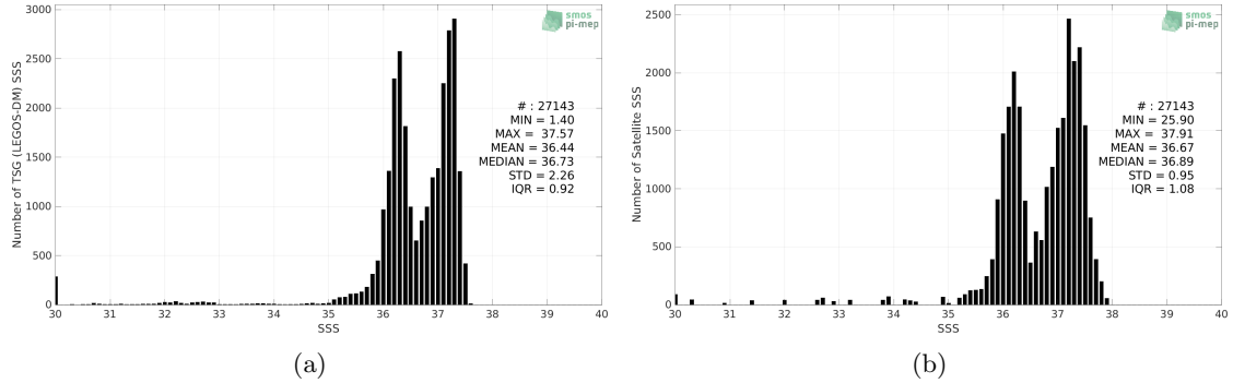
Figure 2: Histograms of SSS from TSG (LEGOS-DM) (a) and Aquarius SSS L3 OR v5 - 7-Day running (NASA-GSFC) (b) considering all match-up pairs per bins of 0.1 over the South Atlantic Ocean Pi-MEP region and for the full satellite product period.
