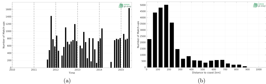
Figure 1: Number of match-ups between TSG (LEGOS-DM) and Aquarius SSS L3 OR v5 - 7-Day running (NASA-GSFC) SSS as a function of time (a) and as function of the distance to coast (b) over the South Atlantic Ocean Pi-MEP region and for the full satellite product period.
