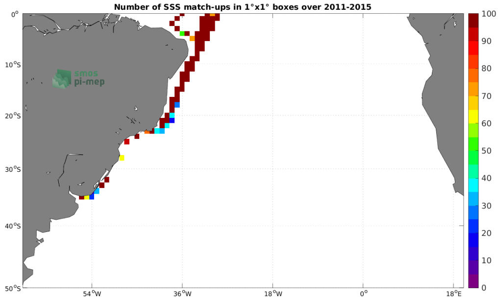
Figure 4: Number of SSS match-ups between TSG (LEGOS-DM) SSS and the Aquarius SSS L3 OR v5 - 7-Day running (NASA-GSFC) SSS product for the South Atlantic Ocean Pi-MEP region over 1^\circ \times 1^\circ boxes and for the full satellite product period.
