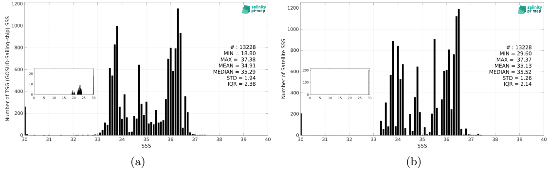
Figure 3: Histograms of SSS from TSG (GOSUD-Sailing-ship) (a) and Aquarius SSS L3 OR v5 - 7-Day running (NASA-GSFC) (b) considering all match-up pairs per bins of 0.1 over the South Atlantic Ocean Pi-MEP region and for the full satellite product period.
