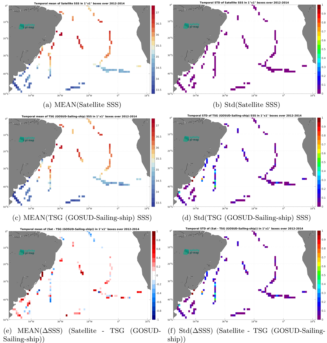
Figure 7: Temporal mean (left) and Std (right) of SSS from Aquarius SSS L3 OR v5 - 7-Day running (NASA-GSFC) (top), TSG (GOSUD-Sailing-ship) (middle), and of \Delta SSS (Satellite - TSG (GOSUD-Sailing-ship)). Only match-up pairs are used to generate these maps.
