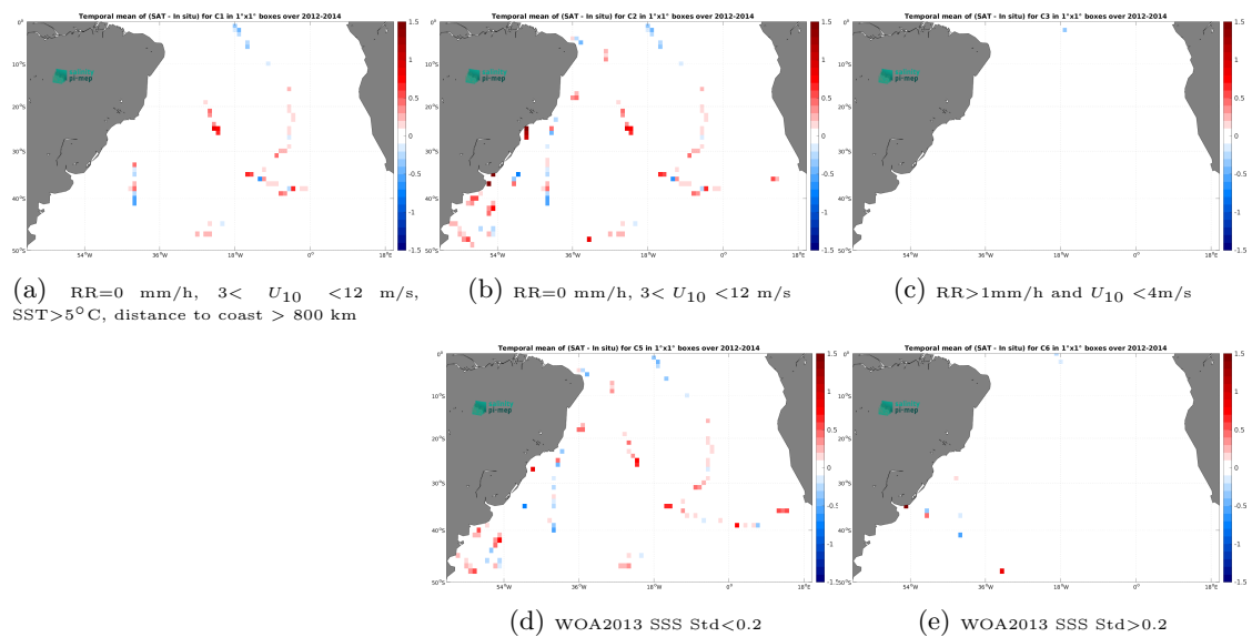
Figure 14: Temporal mean gridded over spatial boxes of size 1^\circ \times 1^\circ of \Delta\text{SSS} (Aquarius SSS L3 OR v5 - 7-Day running (NASA-GSFC) - TSG (GOSUD-Sailing-ship)) for 5 different subdatasets corresponding to:RR=0 mm/h, 3 < U_{10} < 12 m/s, SST >5^\circ\text{C} , distance to coast > 800 km (a), RR=0 mm/h, 3 < U_{10} < 12 m/s (b), RR >1 mm/h and U_{10} < 4 m/s (c), WOA2013 SSS Std <0.2 (d), WOA2013 SSS Std >0.2 (e).
