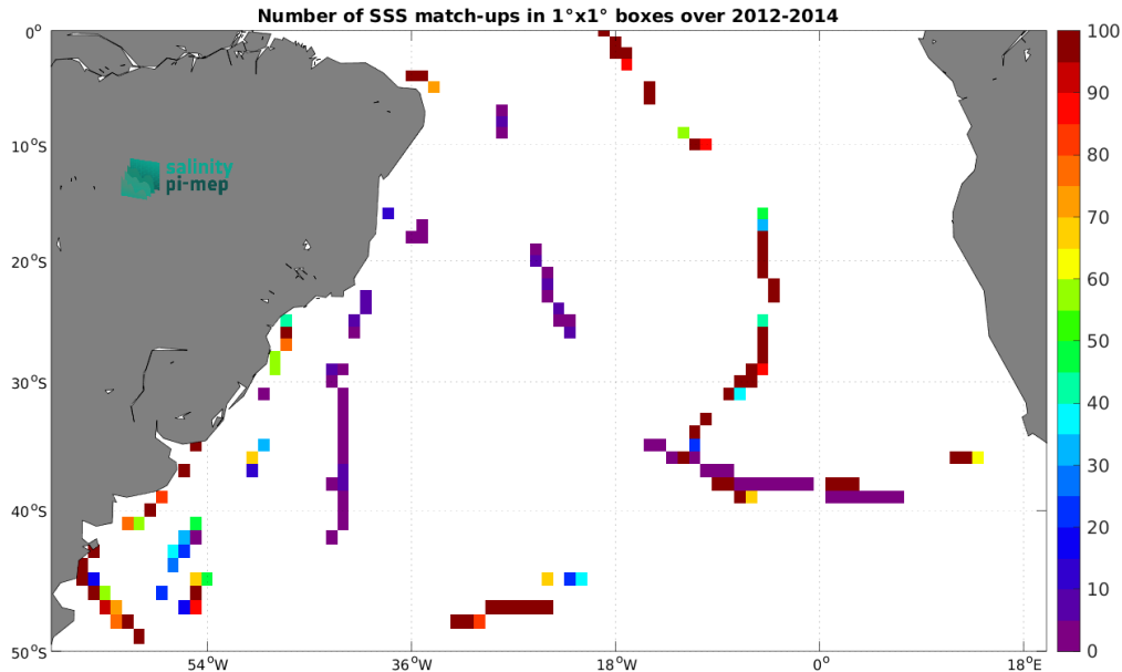
Figure 5: Number of SSS match-ups between TSG (GOSUD-Sailing-ship) SSS and the Aquarius SSS L3 OR v5 - 7-Day running (NASA-GSFC) SSS product for the South Atlantic Ocean Pi-MEP region over 1^\circ \times 1^\circ boxes and for the full satellite product period.
