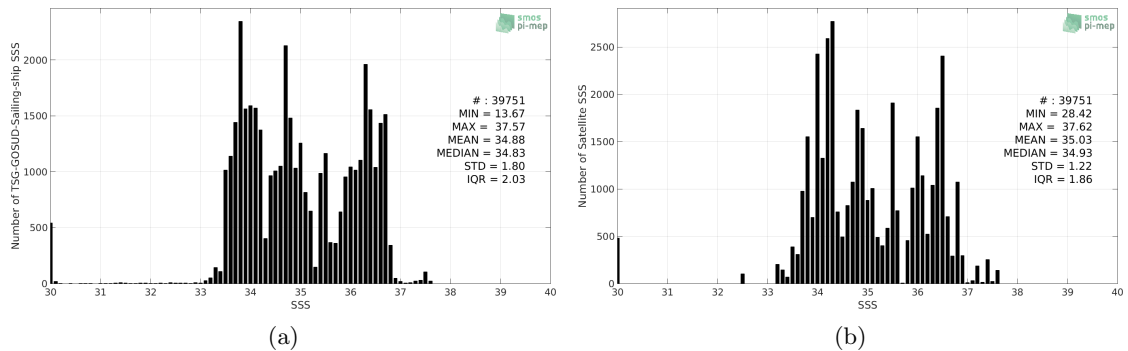
Figure 2: Histograms of SSS from TSG-GOSUD-Sailing-ship (a) and Aquarius-L3-OR-V5-7DAY-RUNNING-1DEG (b) considering all match-up pairs per bins of 0.1 over the South Atlantic Ocean Pi-MEP region and for the full satellite product period.
