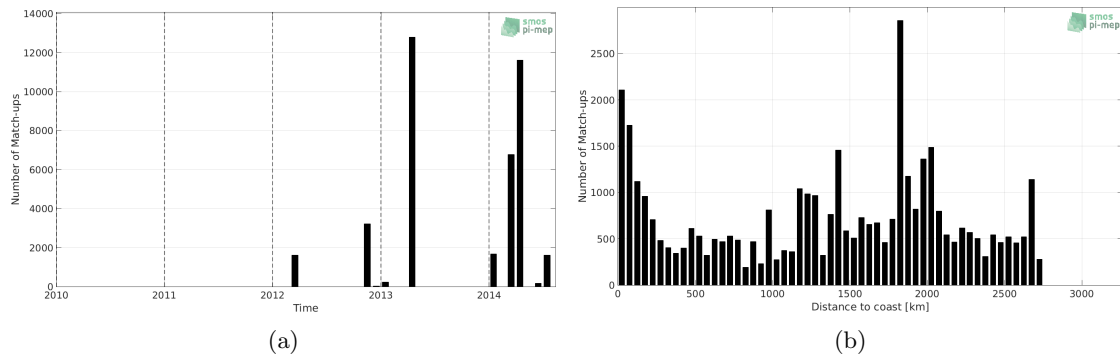
Figure 1: Number of match-ups between TSG-GOSUD-Sailing-ship and Aquarius-L3-OR-V5-7DAY-RUNNING-1DEG SSS as a function of time (a) and as function of the distance to coast (b) over the South Atlantic Ocean Pi-MEP region and for the full satellite product period.
