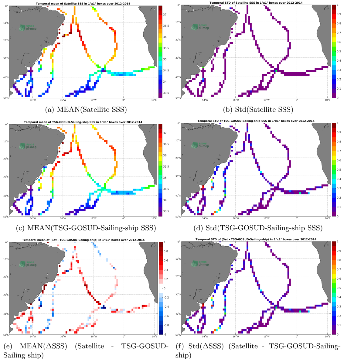
Figure 6: Temporal mean (left) and Std (right) of SSS from Aquarius-L3-OR-V5-7DAY-RUNNING-1DEG (top), TSG-GOSUD-Sailing-ship (middle), and of \Delta SSS (Satellite - TSG-GOSUD-Sailing-ship). Only match-up pairs are used to generate these maps.
