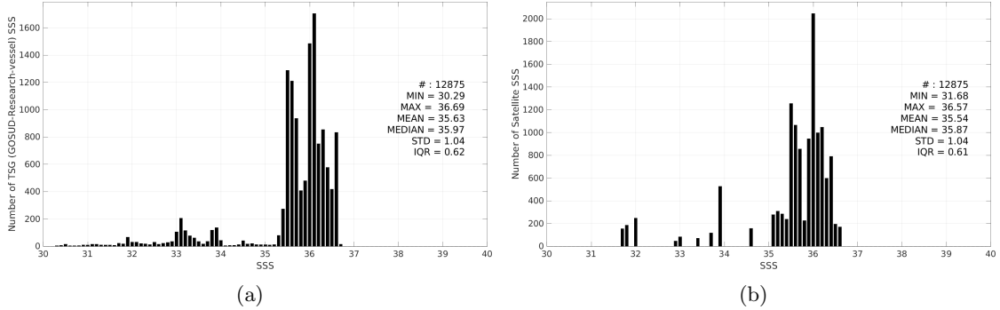
Figure 3: Histograms of SSS from TSG (GOSUD-Research-vessel) (a) and Aquarius SSS L3 OR v5 - 7-Day running (NASA-GSFC) (b) considering all match-up pairs per bins of 0.1 over the South Atlantic Ocean Pi-MEP region and for the full satellite product period.
