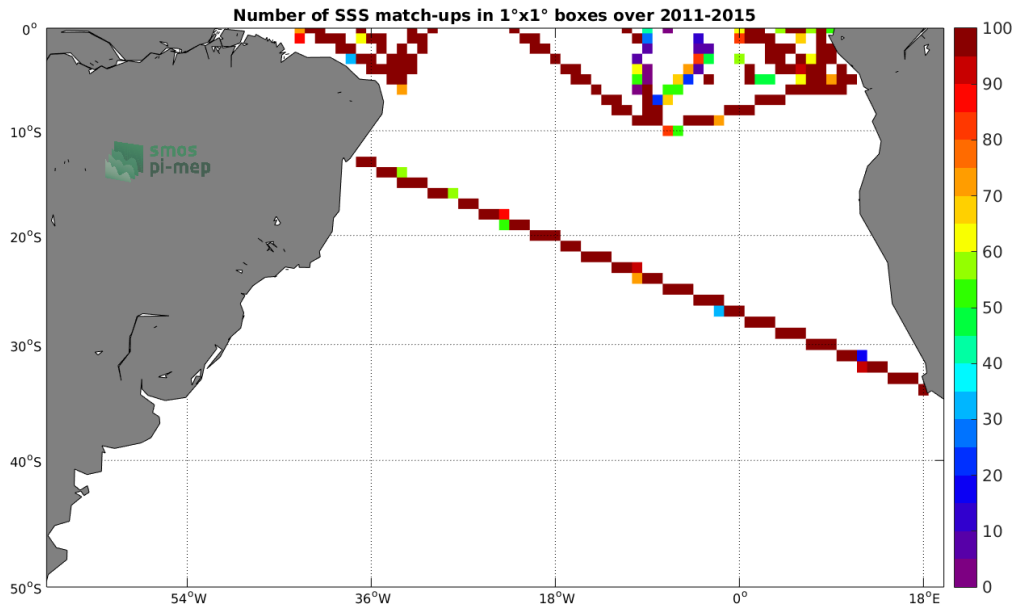
Figure 4: Number of SSS match-ups between TSG-GOSUD-Research-vessel SSS and the Aquarius-L3-OR-V5-7DAY-RUNNING-1DEG SSS product for the South Atlantic Ocean Pi-MEP region over 1^\circ \times 1^\circ boxes and for the full satellite product period.
