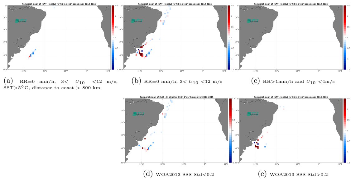
Figure 14: Temporal mean gridded over spatial boxes of size 1^\circ \times 1^\circ of \Delta\text{SSS} (Aquarius SSS L3 OR v5 - 7-Day running (NASA-GSFC) - TSG (CSIC-UTM)) for 5 different subdatasets corresponding to:RR=0 mm/h, 3 < U_{10} < 12 m/s, SST >5^\circ\text{C} , distance to coast > 800 km (a), RR=0 mm/h, 3 < U_{10} < 12 m/s (b), RR >1 mm/h and U_{10} < 4 m/s (c), WOA2013 SSS Std <0.2 (d), WOA2013 SSS Std >0.2 (e).
