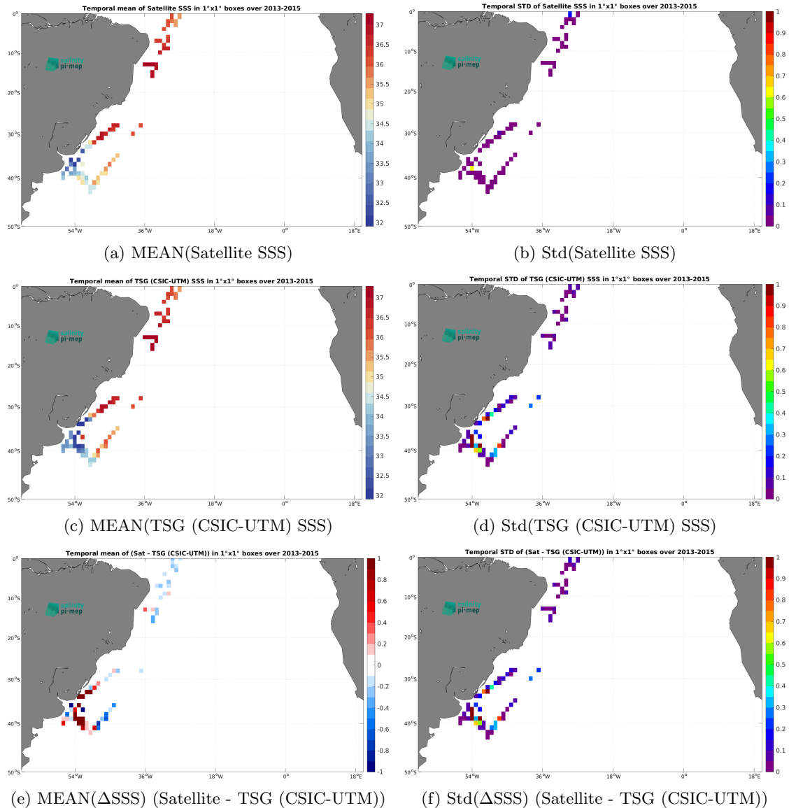
Figure 7: Temporal mean (left) and Std (right) of SSS from Aquarius SSS L3 OR v5 - 7-Day running (NASA-GSFC) (top), TSG (CSIC-UTM) ( in situ ) dataset (middle), and of \Delta SSS (Satellite - TSG (CSIC-UTM)). Only match-up pairs are used to generate these maps.
