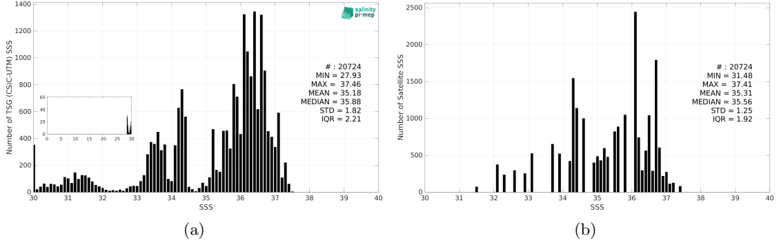
Figure 3: Histograms of SSS from TSG (CSIC-UTM) (a) and Aquarius SSS L3 OR v5 - 7-Day running (NASA-GSFC) (b) considering all match-up pairs per bins of 0.1 over the South Atlantic Ocean Pi-MEP region and for the full satellite product period.
