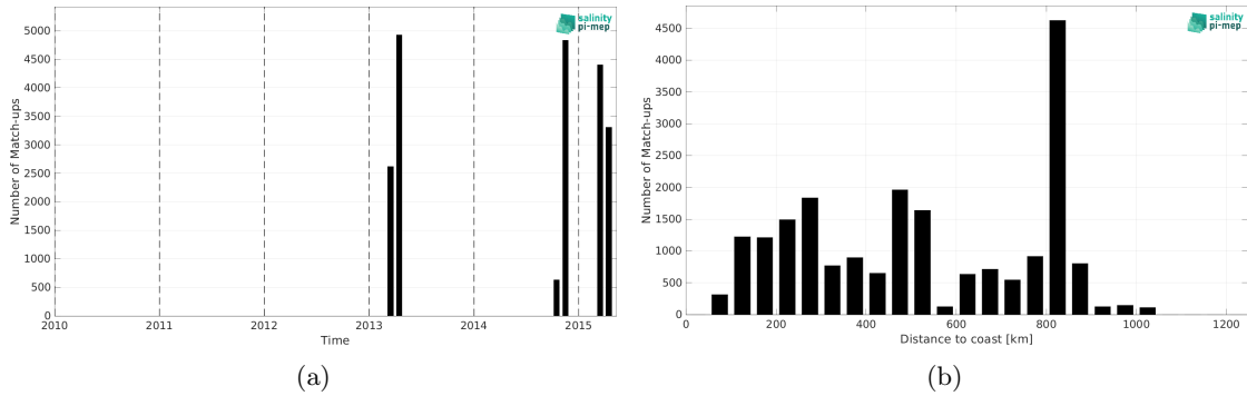
Figure 2: Number of match-ups between TSG (CSIC-UTM) and Aquarius SSS L3 OR v5 - 7-Day running (NASA-GSFC) SSS as a function of time (a) and as function of the distance to coast (b) over the South Atlantic Ocean Pi-MEP region and for the full satellite product period.
