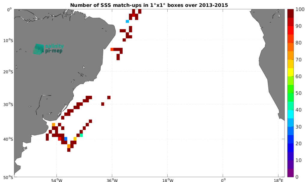
Figure 5: Number of SSS match-ups between TSG (CSIC-UTM) SSS and the Aquarius SSS L3 OR v5 - 7-Day running (NASA-GSFC) SSS product for the South Atlantic Ocean Pi-MEP region over 1^\circ \times 1^\circ boxes and for the full satellite product period.
