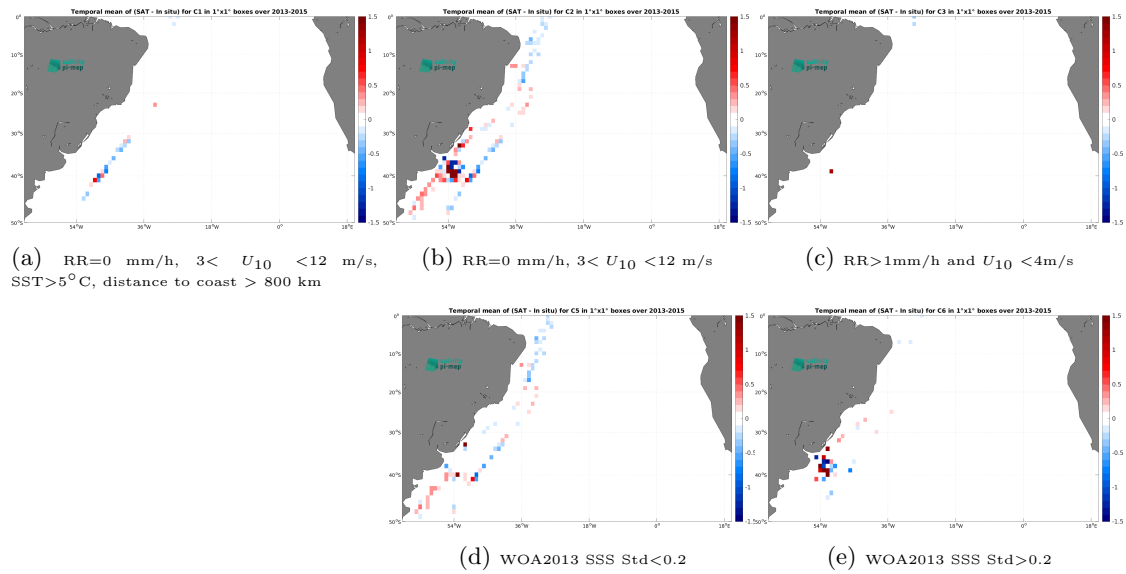
Figure 12: Temporal mean gridded over spatial boxes of size 1^\circ \times 1^\circ of \Delta\text{SSS} (Aquarius SSS L3 OR v5 - 7-Day running (NASA-GSFC) - TSG (CSIC-UTM)) for 5 different subdatasets corresponding to:RR=0 mm/h, 3 < U_{10} < 12 m/s, SST >5^\circ\text{C} , distance to coast > 800 km (a), RR=0 mm/h, 3 < U_{10} < 12 m/s (b), RR >1 mm/h and U_{10} < 4 m/s (c), WOA2013 SSS Std <0.2 (d), WOA2013 SSS Std >0.2 (e).
