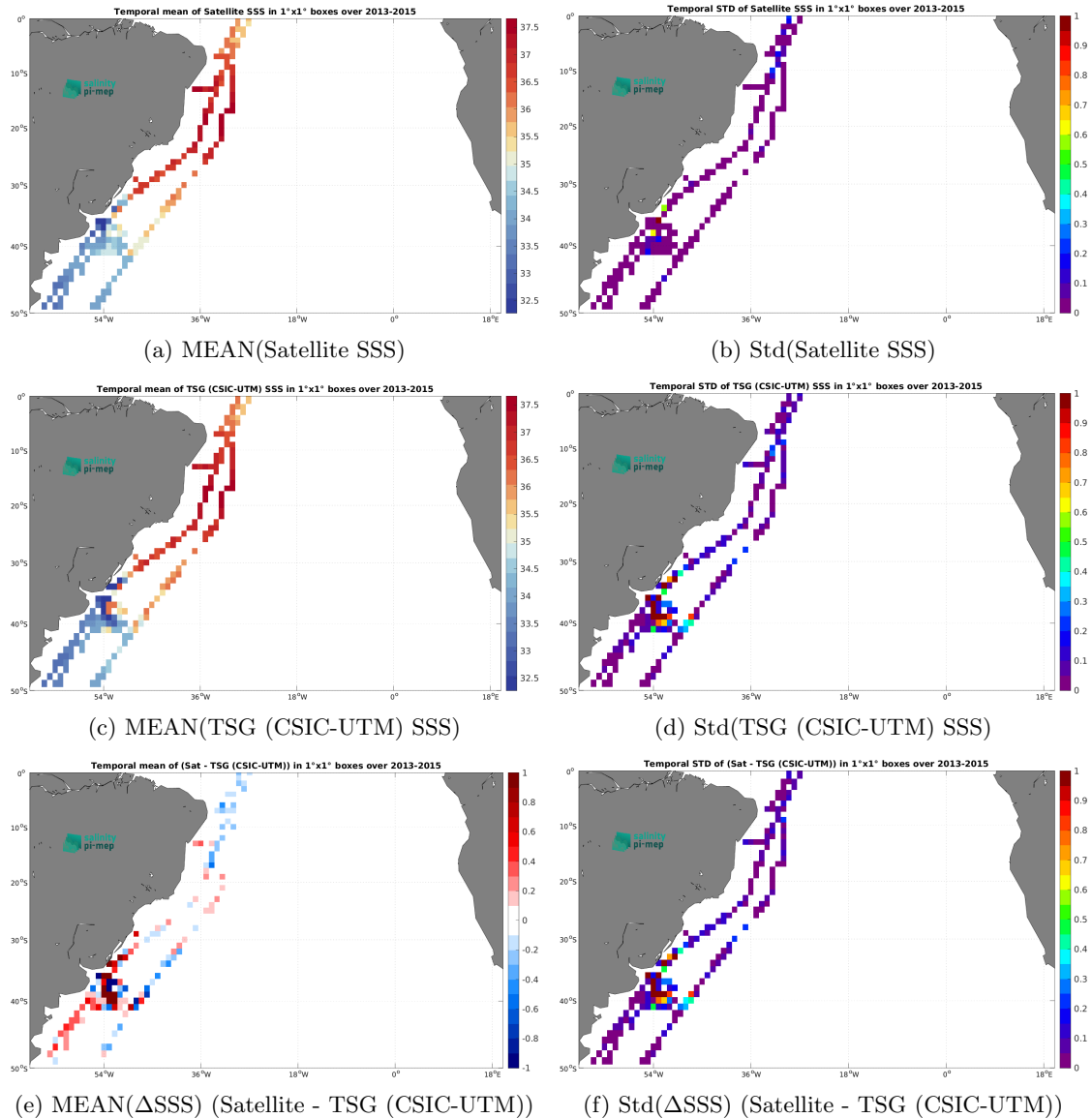
Figure 6: Temporal mean (left) and Std (right) of SSS from Aquarius SSS L3 OR v5 - 7-Day running (NASA-GSFC) (top), TSG (CSIC-UTM) ( in situ ) dataset (middle), and of \Delta SSS (Satellite - TSG (CSIC-UTM)). Only match-up pairs are used to generate these maps.
