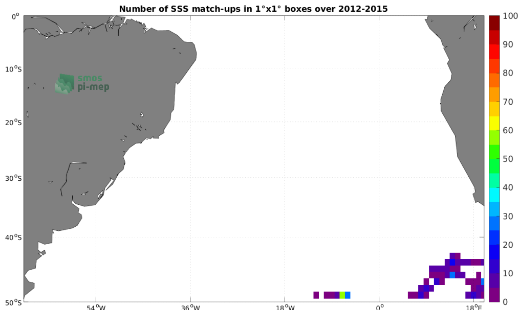
Figure 4: Number of SSS match-ups between Marine mammals SSS and the Aquarius SSS L3 OR v5 - 7-Day running (NASA-GSFC) SSS product for the South Atlantic Ocean Pi-MEP region over 1^\circ \times 1^\circ boxes and for the full satellite product period.
