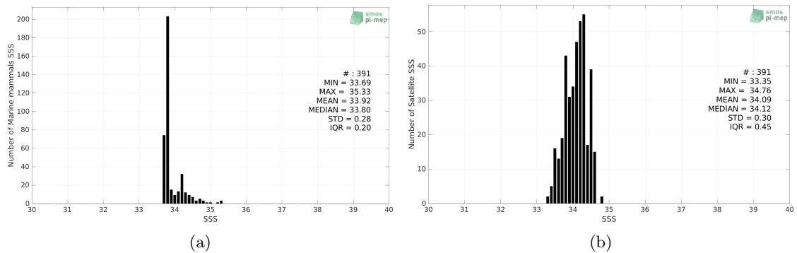
Figure 2: Histograms of SSS from Marine mammals (a) and Aquarius SSS L3 OR v5 - 7-Day running (NASA-GSFC) (b) considering all match-up pairs per bins of 0.1 over the South Atlantic Ocean Pi-MEP region and for the full satellite product period.
