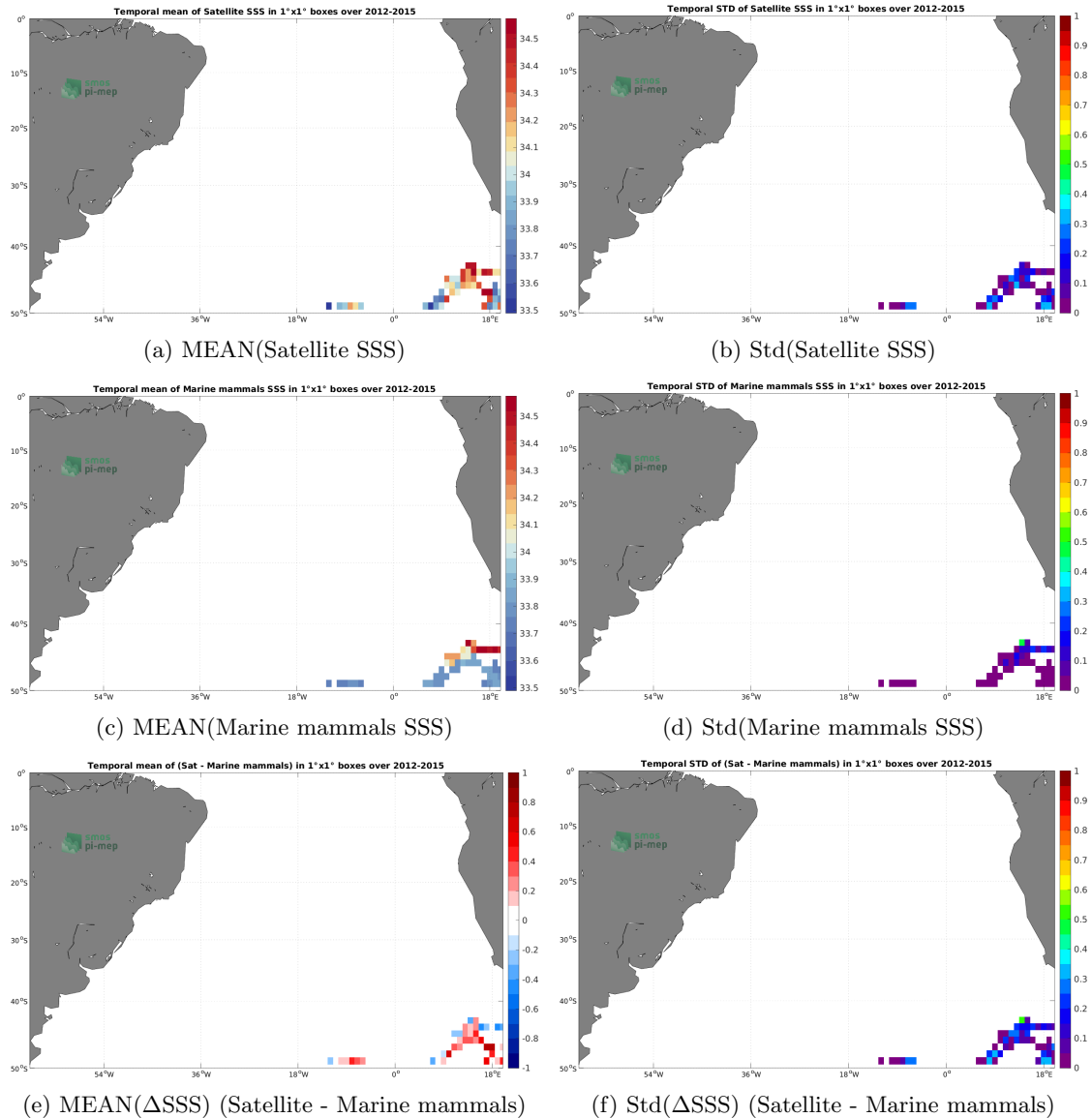
Figure 6: Temporal mean (left) and Std (right) of SSS from Aquarius SSS L3 OR v5 - 7-Day running (NASA-GSFC) (top), Marine mammals (middle), and of \Delta SSS (Satellite - Marine mammals). Only match-up pairs are used to generate these maps.
