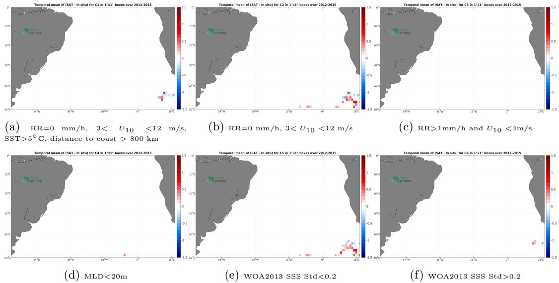
Figure 12: Temporal mean gridded over spatial boxes of size 1^{\circ}\times 1^{\circ} of \Delta\text{SSS} (Aquarius SSS L3 OR v5 - 7-Day running (NASA-GSFC) - Marine mammals) for 6 different subdatasets corresponding to:RR=0 mm/h, 3 < U_{10} < 12 m/s, SST >5^{\circ}\text{C} , distance to coast > 800 km (a), RR=0 mm/h, 3 < U_{10} < 12 m/s (b), RR >1 mm/h and U_{10} < 4 m/s (c),MLD <20 m (d),WOA2013 SSS Std <0.2 (e),WOA2013 SSS Std >0.2 (f).
