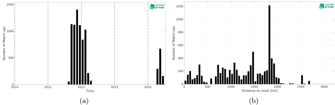
Figure 2: Number of match-ups between Surface drifters and Aquarius SSS L3 OR v5 - 7-Day running (NASA-GSFC) SSS as a function of time (a) and as function of the distance to coast (b) over the South Atlantic Ocean Pi-MEP region and for the full satellite product period.
