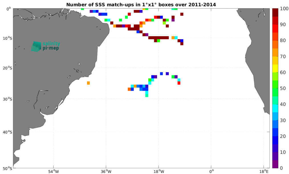
Figure 4: Number of SSS match-ups between Surface drifters SSS and the Aquarius SSS L3 OR v5 - 7-Day running (NASA-GSFC) SSS product for the South Atlantic Ocean Pi-MEP region over 1^\circ \times 1^\circ boxes and for the full satellite product period.
