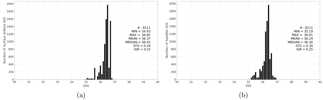
Figure 3: Histograms of SSS from Surface drifters (a) and Aquarius SSS L3 OR v5 - 7-Day running (NASA-GSFC) (b) considering all match-up pairs per bins of 0.1 over the South Atlantic Ocean Pi-MEP region and for the full satellite product period.
