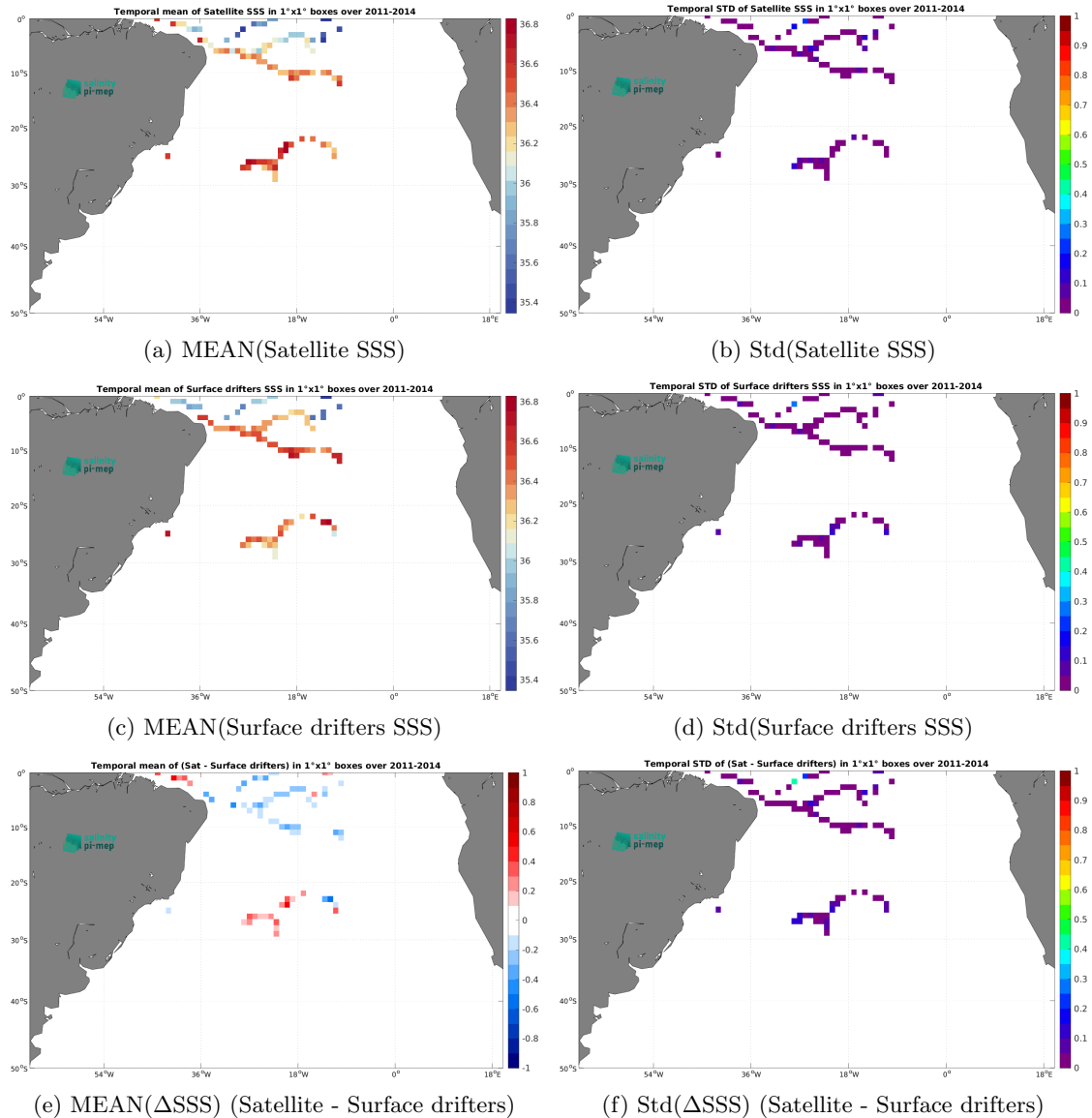
Figure 6: Temporal mean (left) and Std (right) of SSS from Aquarius SSS L3 OR v5 - 7-Day running (NASA-GSFC) (top), Surface drifters (middle), and of \Delta SSS (Satellite - Surface drifters). Only match-up pairs are used to generate these maps.
