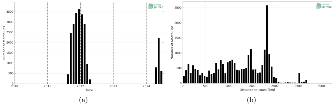
Figure 1: Number of match-ups between Surface drifters and Aquarius SSS L3 OR v5 - 7-Day running (NASA-GSFC) SSS as a function of time (a) and as function of the distance to coast (b) over the South Atlantic Ocean Pi-MEP region and for the full satellite product period.
