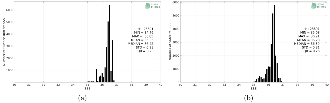
Figure 2: Histograms of SSS from Surface drifters (a) and Aquarius SSS L3 OR v5 - 7-Day running (NASA-GSFC) (b) considering all match-up pairs per bins of 0.1 over the South Atlantic Ocean Pi-MEP region and for the full satellite product period.
