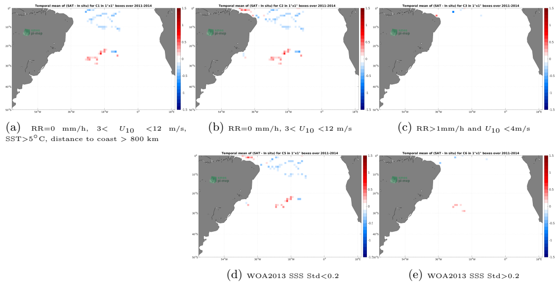
Figure 11: Temporal mean gridded over spatial boxes of size 1^\circ \times 1^\circ of \Delta\text{SSS} (Aquarius SSS L3 OR v5 - 7-Day running (NASA-GSFC) - Surface drifters) for 5 different subdatasets corresponding to:RR=0 mm/h, 3 < U_{10} < 12 m/s, SST >5^\circ\text{C} , distance to coast > 800 km (a), RR=0 mm/h, 3 < U_{10} < 12 m/s (b), RR >1 mm/h and U_{10} < 4 m/s (c), WOA2013 SSS Std <0.2 (d), WOA2013 SSS Std >0.2 (e).
