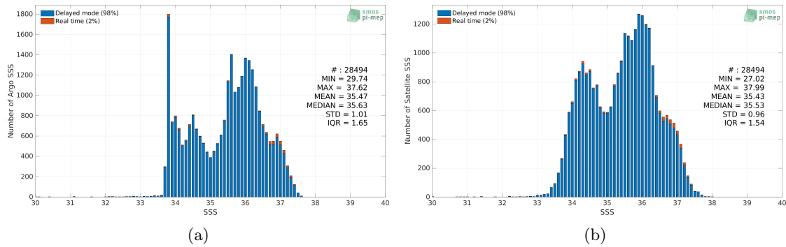
Figure 2: Histograms of SSS from Argo (a) and Aquarius SSS L3 OR v5 - 7-Day running (NASA-GSFC) (b) considering all match-up pairs per bins of 0.1 over the South Atlantic Ocean Pi-MEP region and for the full satellite product period.
