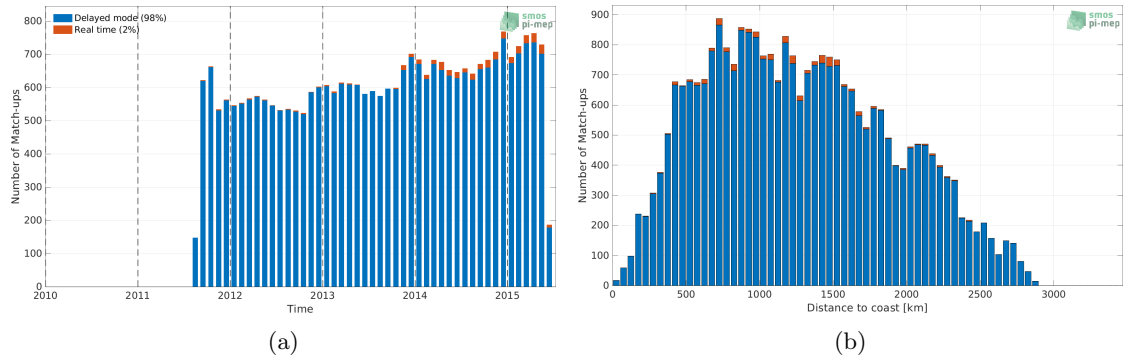
Figure 1: Number of match-ups between Argo and Aquarius SSS L3 OR v5 - 7-Day running (NASA-GSFC) SSS as a function of time (a) and as function of the distance to coast (b) over the South Atlantic Ocean Pi-MEP region and for the full satellite product period.
