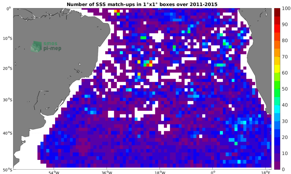
Figure 4: Number of SSS match-ups between Argo SSS and the Aquarius SSS L3 OR v5 - 7-Day running (NASA-GSFC) SSS product for the South Atlantic Ocean Pi-MEP region over 1^\circ \times 1^\circ boxes and for the full satellite product period.
