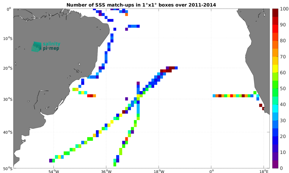
Figure 5: Number of SSS match-ups between TSG (SAMOS) SSS and the Aquarius SSS L3 OR v5 - 7-Day running - Rain mask (NASA-GSFC) SSS product for the South Atlantic Ocean Pi-MEP region over 1^{\circ} \times 1^{\circ} boxes and for the full satellite product period.
