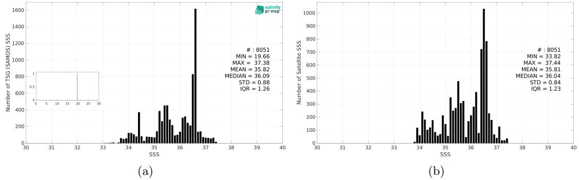
Figure 3: Histograms of SSS from TSG (SAMOS) (a) and Aquarius SSS L3 OR v5 - 7-Day running - Rain mask (NASA-GSFC) (b) considering all match-up pairs per bins of 0.1 over the South Atlantic Ocean Pi-MEP region and for the full satellite product period.
