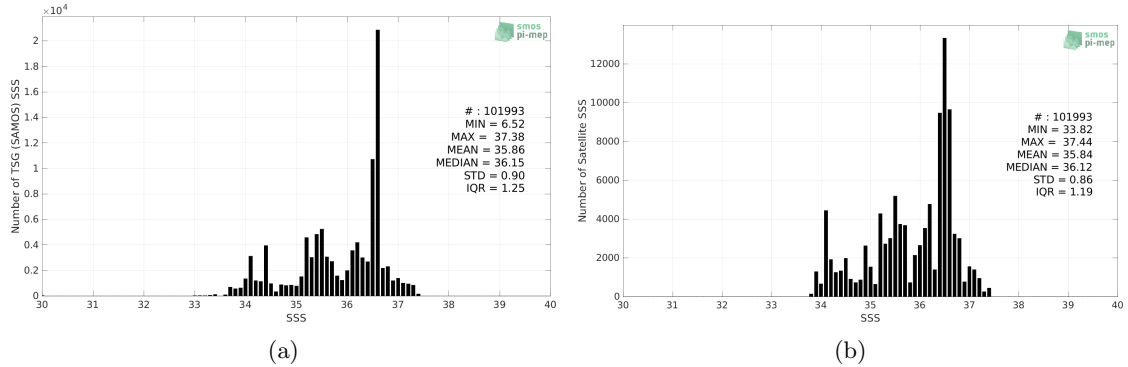
Figure 2: Histograms of SSS from TSG (SAMOS) (a) and Aquarius SSS L3 OR v5 - 7-Day running - Rain mask (NASA-GSFC) (b) considering all match-up pairs per bins of 0.1 over the South Atlantic Ocean Pi-MEP region and for the full satellite product period.
