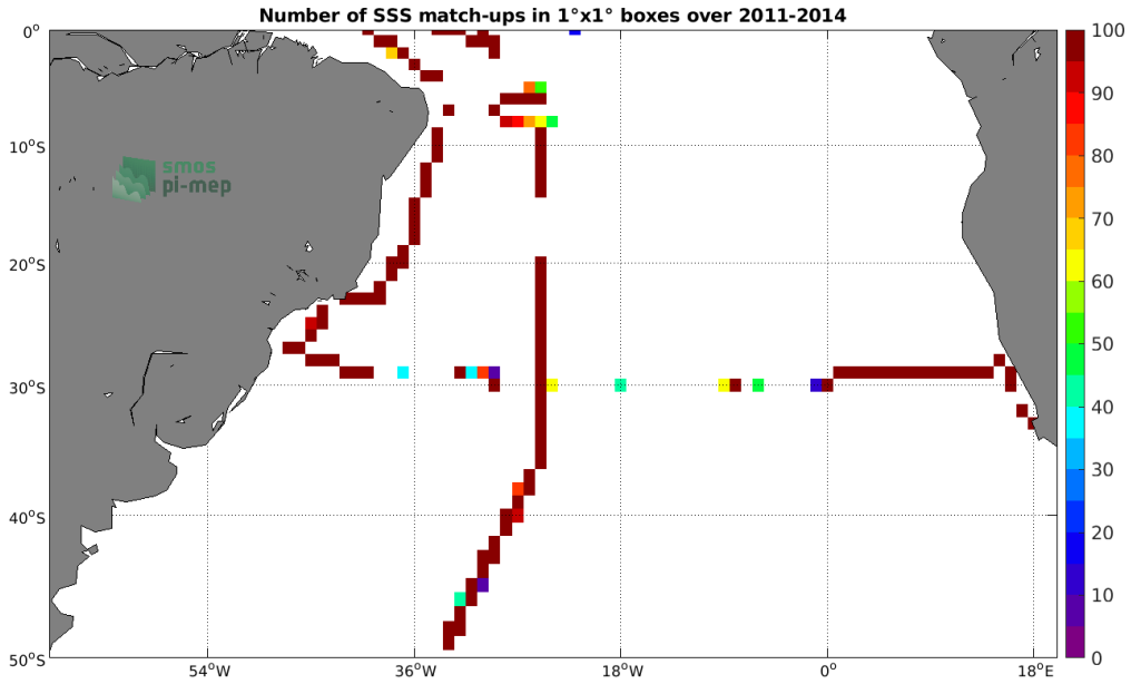
Figure 4: Number of SSS match-ups between TSG (SAMOS) SSS and the Aquarius SSS L3 OR v5 - 7-Day running - Rain mask (NASA-GSFC) SSS product for the South Atlantic Ocean Pi-MEP region over 1^{\circ} \times 1^{\circ} boxes and for the full satellite product period.
