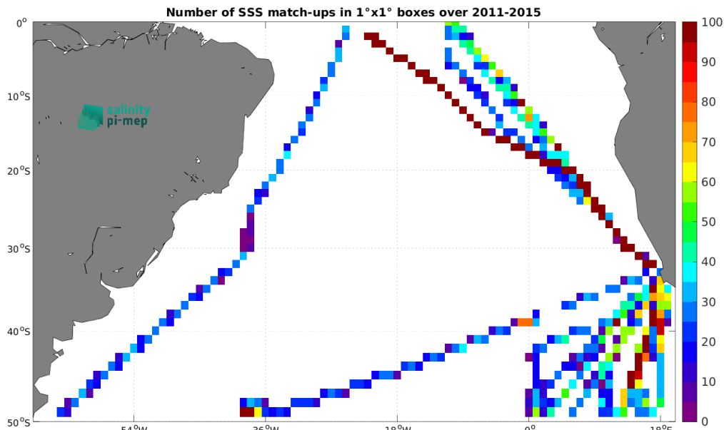
Figure 5: Number of SSS match-ups between TSG (Polarstern) SSS and the Aquarius SSS L3 OR v5 - 7-Day running - Rain mask (NASA-GSFC) SSS product for the South Atlantic Ocean Pi-MEP region over 1^\circ \times 1^\circ boxes and for the full satellite product period.
