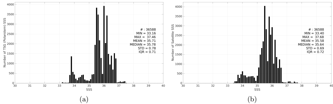
Figure 3: Histograms of SSS from TSG (Polarstern) (a) and Aquarius SSS L3 OR v5 - 7-Day running - Rain mask (NASA-GSFC) (b) considering all match-up pairs per bins of 0.1 over the South Atlantic Ocean Pi-MEP region and for the full satellite product period.
