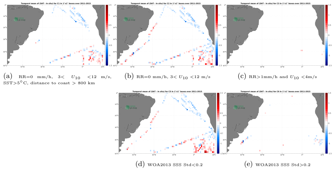
Figure 12: Temporal mean gridded over spatial boxes of size 1^\circ \times 1^\circ of \Delta\text{SSS} (Aquarius SSS L3 OR v5 - 7-Day running - Rain mask (NASA-GSFC) - TSG (Polarstern)) for 5 different subdatasets corresponding to:RR=0 mm/h, 3 < U_{10} < 12 m/s, SST >5^\circ\text{C} , distance to coast > 800 km (a), RR=0 mm/h, 3 < U_{10} < 12 m/s (b), RR >1 mm/h and U_{10} < 4 m/s (c), WOA2013 SSS Std <0.2 (d), WOA2013 SSS Std >0.2 (e).
