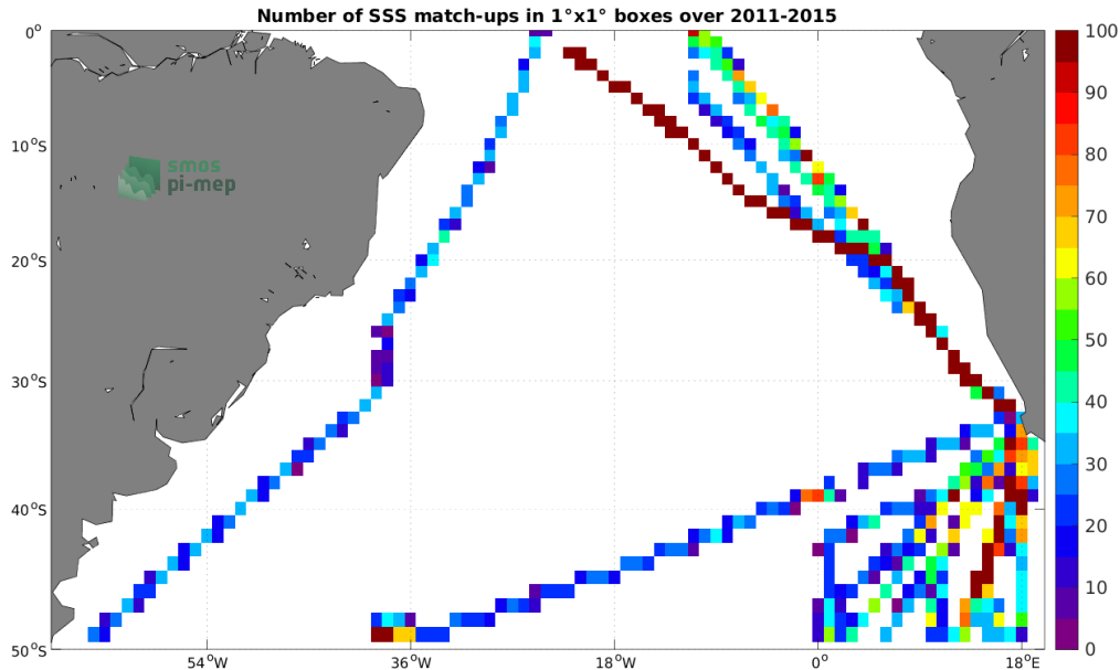
Figure 4: Number of SSS match-ups between TSG (Polarstern) SSS and the Aquarius SSS L3 OR v5 - 7-Day running - Rain mask (NASA-GSFC) SSS product for the South Atlantic Ocean Pi-MEP region over 1^\circ \times 1^\circ boxes and for the full satellite product period.
