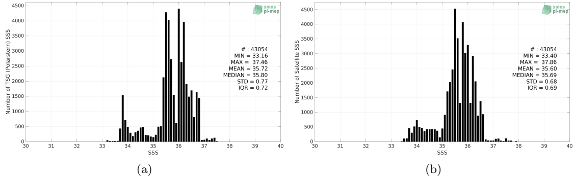
Figure 2: Histograms of SSS from TSG (Polarstern) (a) and Aquarius SSS L3 OR v5 - 7-Day running - Rain mask (NASA-GSFC) (b) considering all match-up pairs per bins of 0.1 over the South Atlantic Ocean Pi-MEP region and for the full satellite product period.
