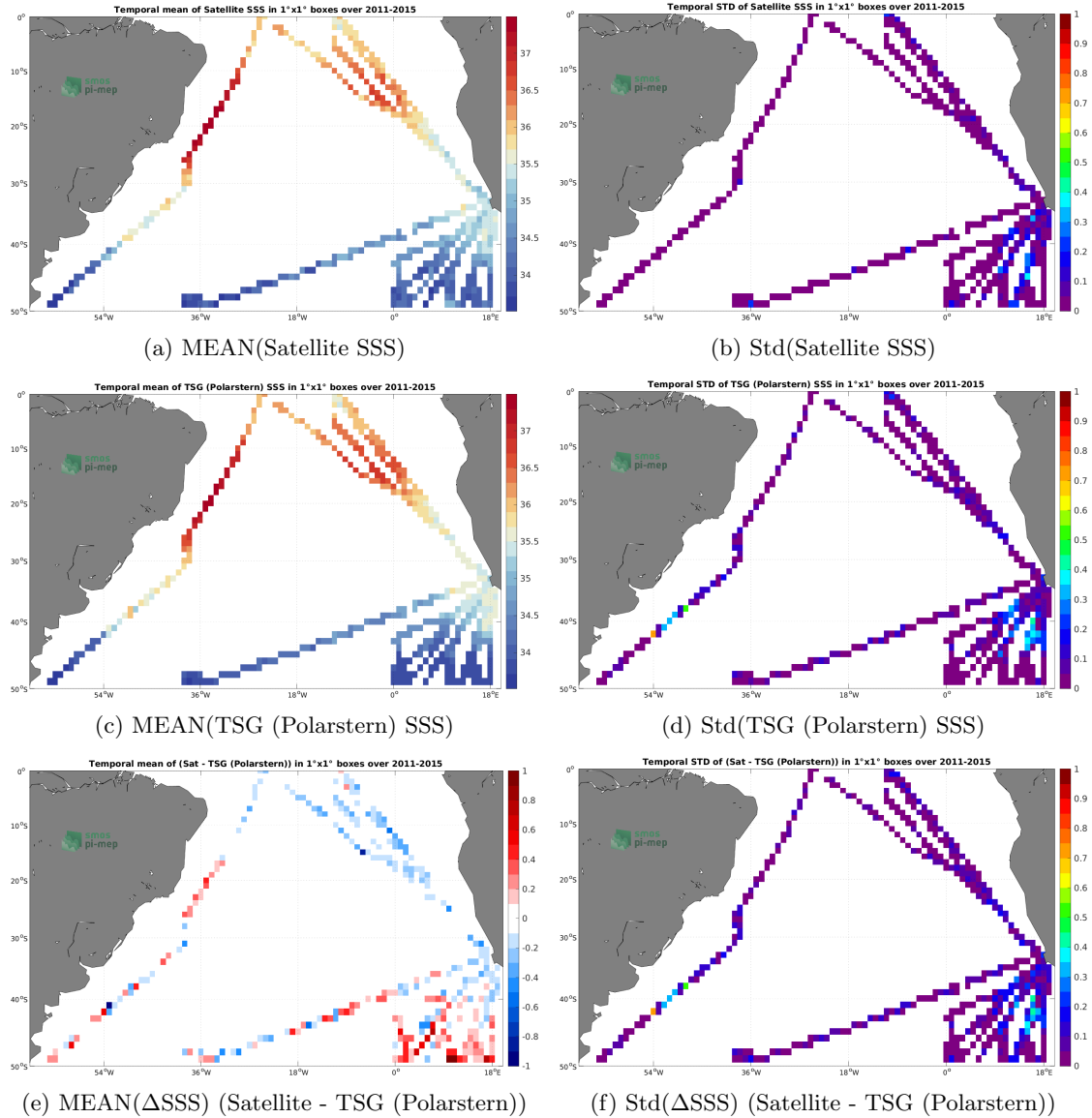
Figure 6: Temporal mean (left) and Std (right) of SSS from Aquarius SSS L3 OR v5 - 7-Day running - Rain mask (NASA-GSFC) (top), TSG (Polarstern) (middle), and of \Delta SSS (Satellite - TSG (Polarstern)). Only match-up pairs are used to generate these maps.
