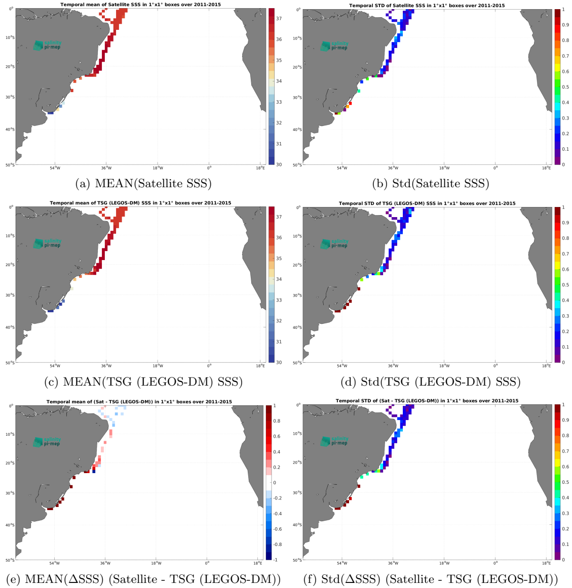
Figure 7: Temporal mean (left) and Std (right) of SSS from Aquarius SSS L3 OR v5 - 7-Day running - Rain mask (NASA-GSFC) (top), TSG (LEGOS-DM) (middle), and of \Delta SSS (Satellite - TSG (LEGOS-DM)). Only match-up pairs are used to generate these maps.
