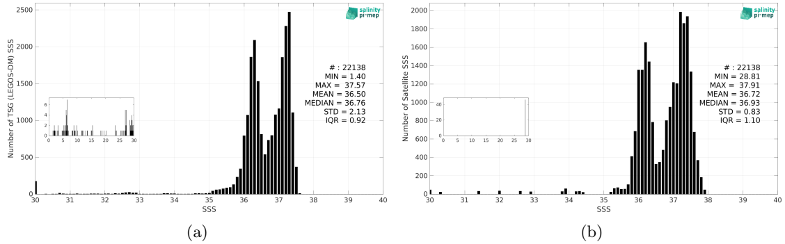
Figure 3: Histograms of SSS from TSG (LEGOS-DM) (a) and Aquarius SSS L3 OR v5 - 7-Day running - Rain mask (NASA-GSFC) (b) considering all match-up pairs per bins of 0.1 over the South Atlantic Ocean Pi-MEP region and for the full satellite product period.
