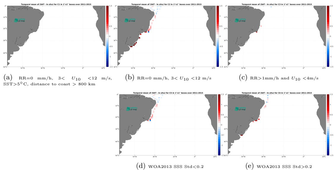
Figure 14: Temporal mean gridded over spatial boxes of size 1^\circ \times 1^\circ of \Delta SSS (Aquarius SSS L3 OR v5 - 7-Day running - Rain mask (NASA-GSFC) - TSG (LEGOS-DM)) for 5 different subdatasets corresponding to:RR=0 mm/h, 3 < U_{10} < 12 m/s, SST >5^\circ\text{C} , distance to coast > 800 km (a), RR=0 mm/h, 3 < U_{10} < 12 m/s (b), RR >1 mm/h and U_{10} < 4 m/s (c), WOA2013 SSS Std <0.2 (d), WOA2013 SSS Std >0.2 (e).
