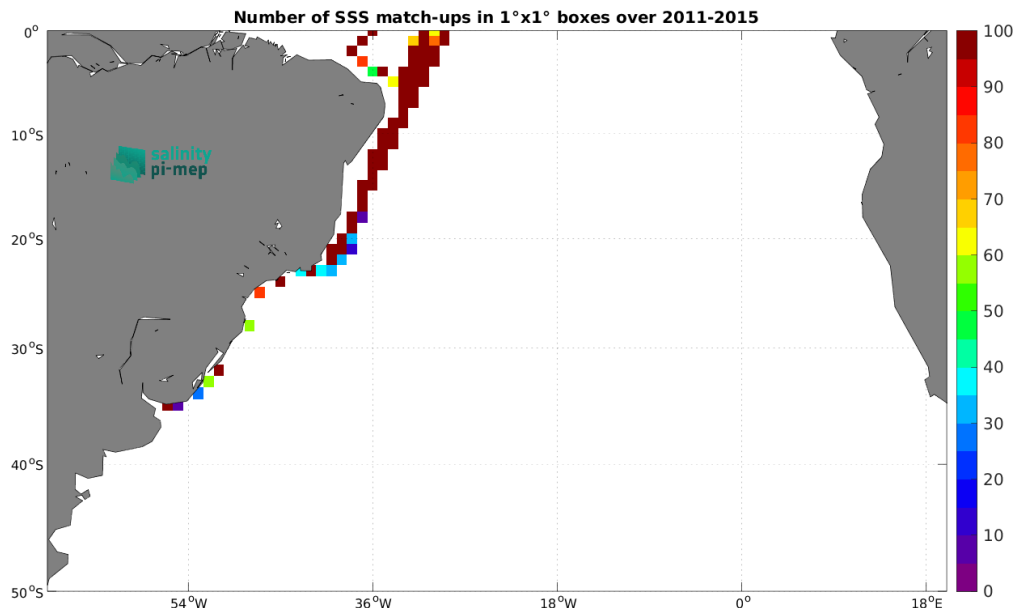
Figure 5: Number of SSS match-ups between TSG (LEGOS-DM) SSS and the Aquarius SSS L3 OR v5 - 7-Day running - Rain mask (NASA-GSFC) SSS product for the South Atlantic Ocean Pi-MEP region over 1^{\circ} \times 1^{\circ} boxes and for the full satellite product period.
