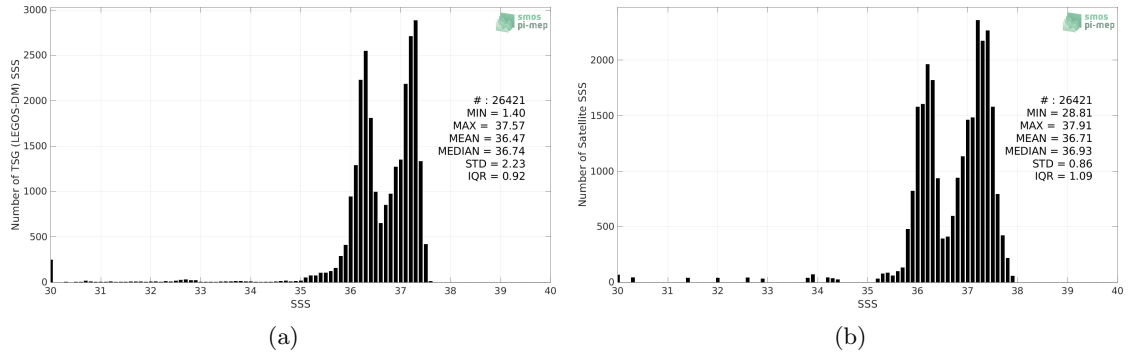
Figure 2: Histograms of SSS from TSG (LEGOS-DM) (a) and Aquarius SSS L3 OR v5 - 7-Day running - Rain mask (NASA-GSFC) (b) considering all match-up pairs per bins of 0.1 over the South Atlantic Ocean Pi-MEP region and for the full satellite product period.
