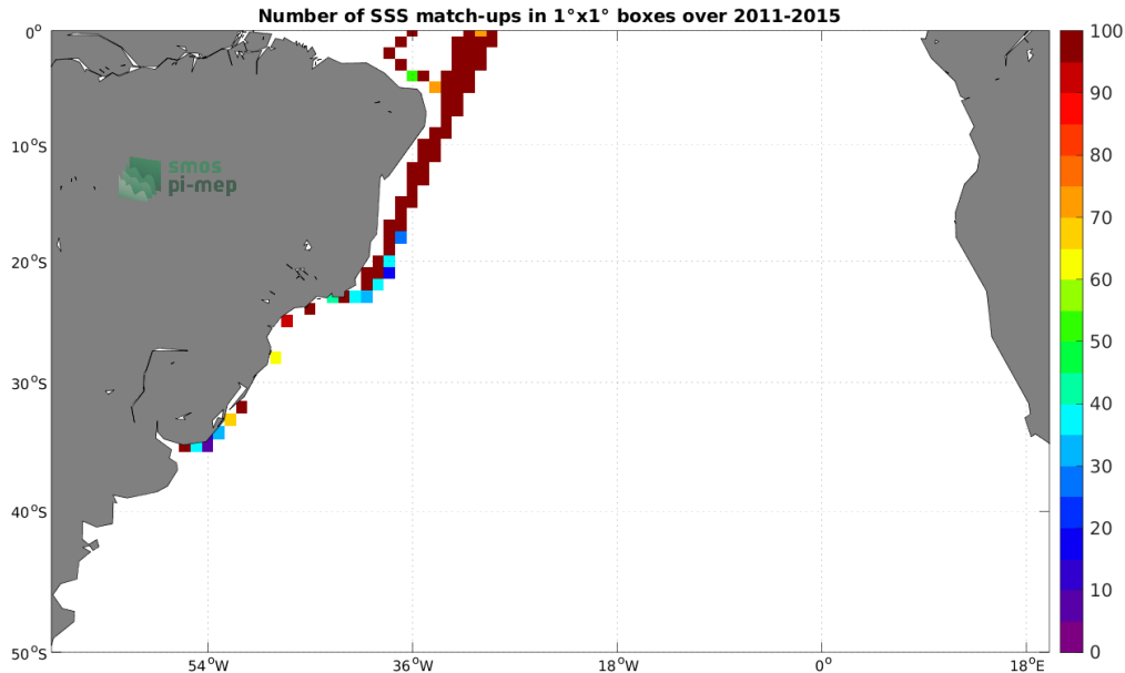
Figure 4: Number of SSS match-ups between TSG (LEGOS-DM) SSS and the Aquarius SSS L3 OR v5 - 7-Day running - Rain mask (NASA-GSFC) SSS product for the South Atlantic Ocean Pi-MEP region over 1^{\circ} \times 1^{\circ} boxes and for the full satellite product period.
