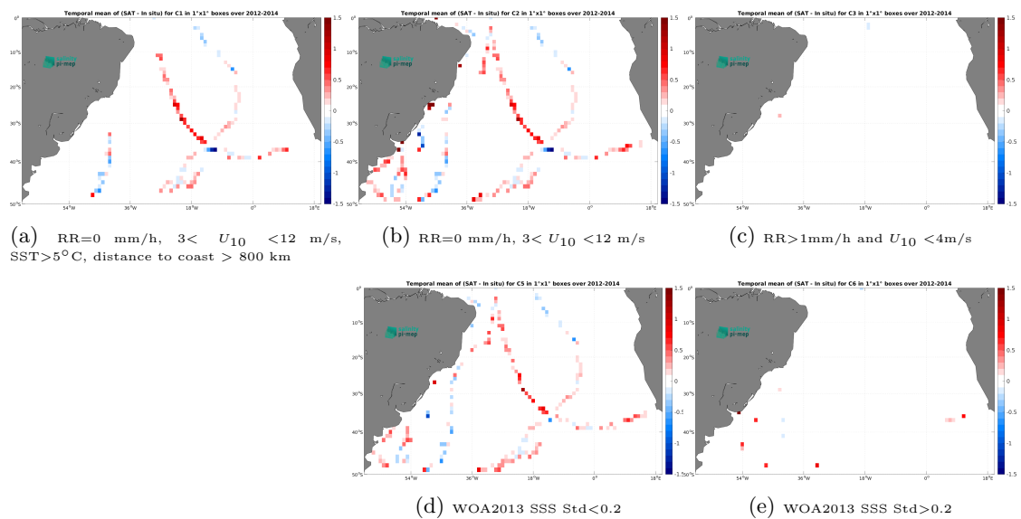
Figure 12: Temporal mean gridded over spatial boxes of size 1^\circ \times 1^\circ of \Delta\text{SSS} (Aquarius SSS L3 OR v5 - 7-Day running - Rain mask (NASA-GSFC) - TSG (GOSUD-Sailing-ship)) for 5 different subdatasets corresponding to:RR=0 mm/h, 3 < U_{10} < 12 m/s, SST >5^\circ\text{C} , distance to coast > 800 km (a), RR=0 mm/h, 3 < U_{10} < 12 m/s (b), RR >1 mm/h and U_{10} < 4 m/s (c), WOA2013 SSS Std <0.2 (d), WOA2013 SSS Std >0.2 (e).
