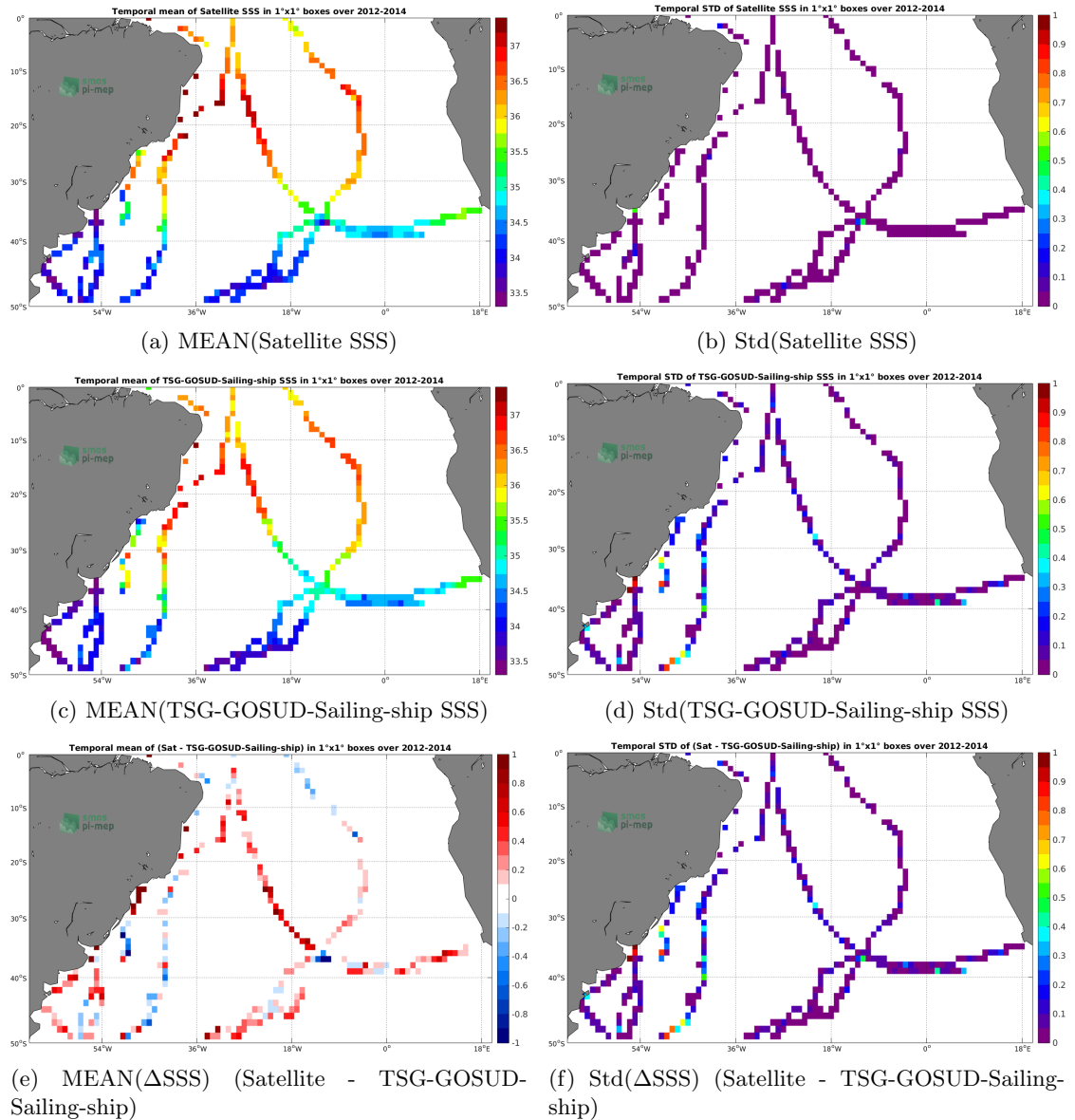
Figure 6: Temporal mean (left) and Std (right) of SSS from Aquarius-L3-OR-V5-7DAY-RUNNING-RAIN-MASK-1DEG (top), TSG-GOSUD-Sailing-ship (middle), and of \Delta SSS (Satellite - TSG-GOSUD-Sailing-ship). Only match-up pairs are used to generate these maps.
