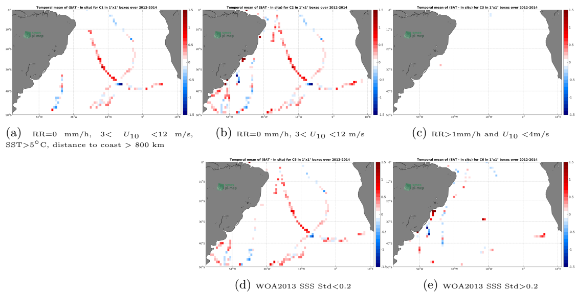
Figure 12: Temporal mean gridded over spatial boxes of size 1^\circ \times 1^\circ of \Delta SSS (Aquarius-L3-OR-V5-7DAY-RUNNING-RAIN-MASK-1DEG - TSG-GOSUD-Sailing-ship) for 5 different subdatasets corresponding to:RR=0 mm/h, 3 < U_{10} < 12 m/s, SST >5^\circ\text{C} , distance to coast > 800 km (a), RR=0 mm/h, 3 < U_{10} < 12 m/s (b), RR >1 mm/h and U_{10} < 4 m/s (c), WOA2013 SSS Std <0.2 (d), WOA2013 SSS Std >0.2 (e).
