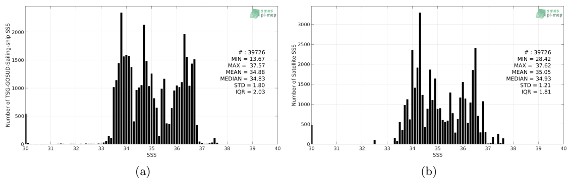
Figure 2: Histograms of SSS from TSG-GOSUD-Sailing-ship (a) and Aquarius-L3-OR-V5-7DAY-RUNNING-RAIN-MASK-1DEG (b) considering all match-up pairs per bins of 0.1 over the South Atlantic Ocean Pi-MEP region and for the full satellite product period.
