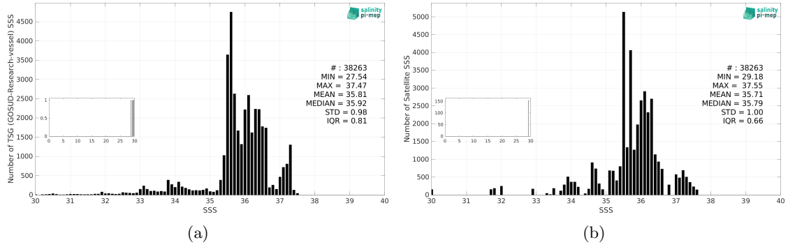
Figure 3: Histograms of SSS from TSG (GOSUD-Research-vessel) (a) and Aquarius SSS L3 OR v5 - 7-Day running - Rain mask (NASA-GSFC) (b) considering all match-up pairs per bins of 0.1 over the South Atlantic Ocean Pi-MEP region and for the full satellite product period.
