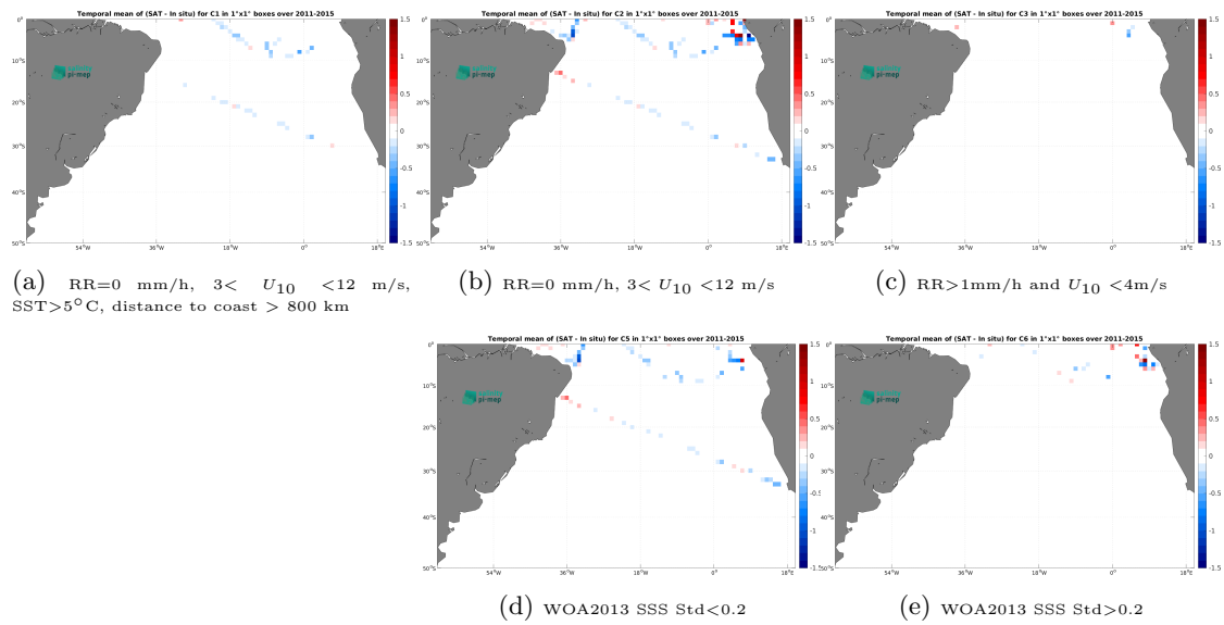
Figure 14: Temporal mean gridded over spatial boxes of size 1^\circ \times 1^\circ of \Delta SSS (Aquarius SSS L3 OR v5 - 7-Day running - Rain mask (NASA-GSFC) - TSG (GOSUD-Research-vessel)) for 5 different subdatasets corresponding to:RR=0 mm/h, 3 < U_{10} < 12 m/s, SST >5^\circ\text{C} , distance to coast > 800 km (a), RR=0 mm/h, 3 < U_{10} < 12 m/s (b), RR >1 mm/h and U_{10} < 4 m/s (c), WOA2013 SSS Std <0.2 (d), WOA2013 SSS Std >0.2 (e).
