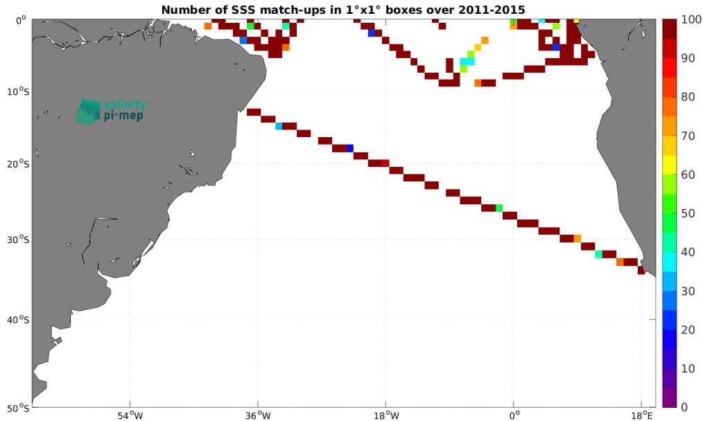
Figure 5: Number of SSS match-ups between TSG (GOSUD-Research-vessel) SSS and the Aquarius SSS L3 OR v5 - 7-Day running - Rain mask (NASA-GSFC) SSS product for the South Atlantic Ocean Pi-MEP region over 1^\circ \times 1^\circ boxes and for the full satellite product period.
