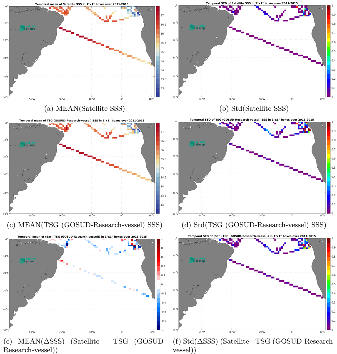
Figure 7: Temporal mean (left) and Std (right) of SSS from Aquarius SSS L3 OR v5 - 7-Day running - Rain mask (NASA-GSFC) (top), TSG (GOSUD-Research-vessel) (middle), and of \Delta SSS (Satellite - TSG (GOSUD-Research-vessel)). Only match-up pairs are used to generate these maps.
