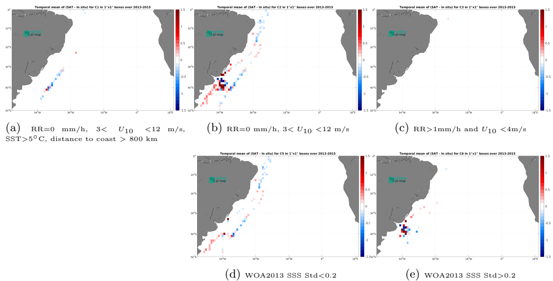
Figure 14: Temporal mean gridded over spatial boxes of size 1^\circ \times 1^\circ of \Delta SSS (Aquarius SSS L3 OR v5 - 7-Day running - Rain mask (NASA-GSFC) - TSG (CSIC-UTM)) for 5 different subdatasets corresponding to:RR=0 mm/h, 3 < U_{10} < 12 m/s, SST >5^\circ\text{C} , distance to coast > 800 km (a), RR=0 mm/h, 3 < U_{10} < 12 m/s (b), RR >1 mm/h and U_{10} < 4 m/s (c), WOA2013 SSS Std <0.2 (d), WOA2013 SSS Std >0.2 (e).
