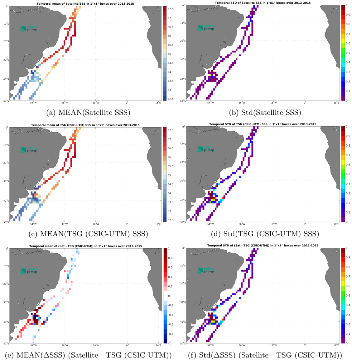
Figure 7: Temporal mean (left) and Std (right) of SSS from Aquarius SSS L3 OR v5 - 7-Day running - Rain mask (NASA-GSFC) (top), TSG (CSIC-UTM) (middle), and of \Delta SSS (Satellite - TSG (CSIC-UTM)). Only match-up pairs are used to generate these maps.
