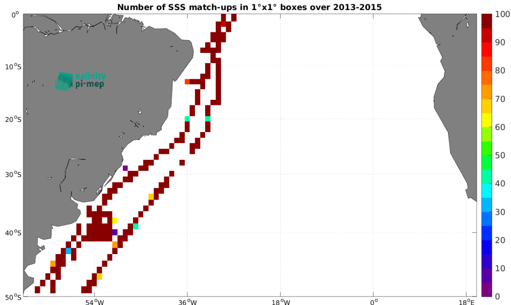
Figure 5: Number of SSS match-ups between TSG (CSIC-UTM) SSS and the Aquarius SSS L3 OR v5 - 7-Day running - Rain mask (NASA-GSFC) SSS product for the South Atlantic Ocean Pi-MEP region over 1^{\circ} \times 1^{\circ} boxes and for the full satellite product period.
