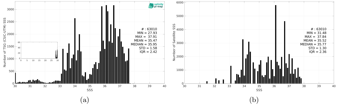
Figure 3: Histograms of SSS from TSG (CSIC-UTM) (a) and Aquarius SSS L3 OR v5 - 7-Day running - Rain mask (NASA-GSFC) (b) considering all match-up pairs per bins of 0.1 over the South Atlantic Ocean Pi-MEP region and for the full satellite product period.
