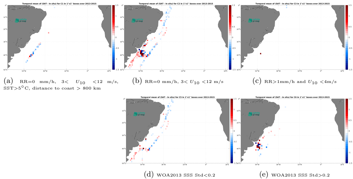
Figure 12: Temporal mean gridded over spatial boxes of size 1^\circ \times 1^\circ of \Delta SSS (Aquarius SSS L3 OR v5 - 7-Day running - Rain mask (NASA-GSFC) - TSG (CSIC-UTM)) for 5 different subdatasets corresponding to:RR=0 mm/h, 3 < U_{10} < 12 m/s, SST >5^\circ\text{C} , distance to coast > 800 km (a), RR=0 mm/h, 3 < U_{10} < 12 m/s (b), RR >1 mm/h and U_{10} < 4 m/s (c), WOA2013 SSS Std <0.2 (d), WOA2013 SSS Std >0.2 (e).
