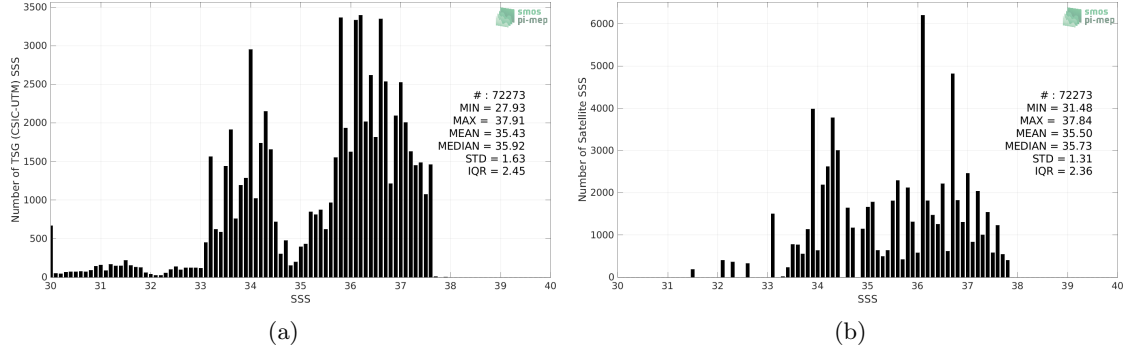
Figure 2: Histograms of SSS from TSG (CSIC-UTM) (a) and Aquarius SSS L3 OR v5 - 7-Day running - Rain mask (NASA-GSFC) (b) considering all match-up pairs per bins of 0.1 over the South Atlantic Ocean Pi-MEP region and for the full satellite product period.
