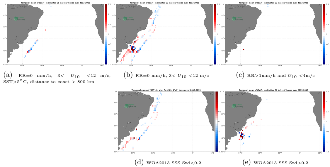
Figure 12: Temporal mean gridded over spatial boxes of size 1^\circ \times 1^\circ of \Delta\text{SSS} (Aquarius SSS L3 OR v5 - 7-Day running - Rain mask (NASA-GSFC) - TSG (CSIC-UTM)) for 5 different subdatasets corresponding to: \text{RR}=0 mm/h, 3 < U_{10} < 12 m/s, \text{SST} > 5^\circ\text{C} , distance to coast > 800 km (a), \text{RR}=0 mm/h, 3 < U_{10} < 12 m/s (b), \text{RR} > 1\text{mm/h} and U_{10} < 4\text{m/s} (c), WOA2013 SSS Std < 0.2 (d), WOA2013 SSS Std > 0.2 (e).
