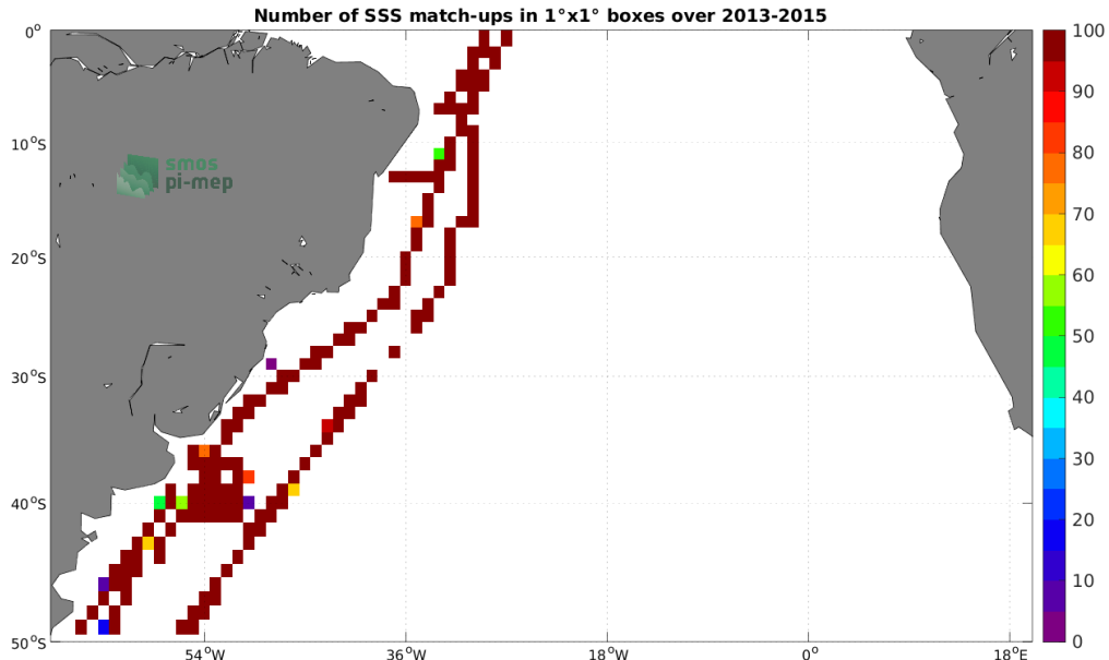
Figure 4: Number of SSS match-ups between TSG (CSIC-UTM) SSS and the Aquarius SSS L3 OR v5 - 7-Day running - Rain mask (NASA-GSFC) SSS product for the South Atlantic Ocean Pi-MEP region over 1^\circ \times 1^\circ boxes and for the full satellite product period.
