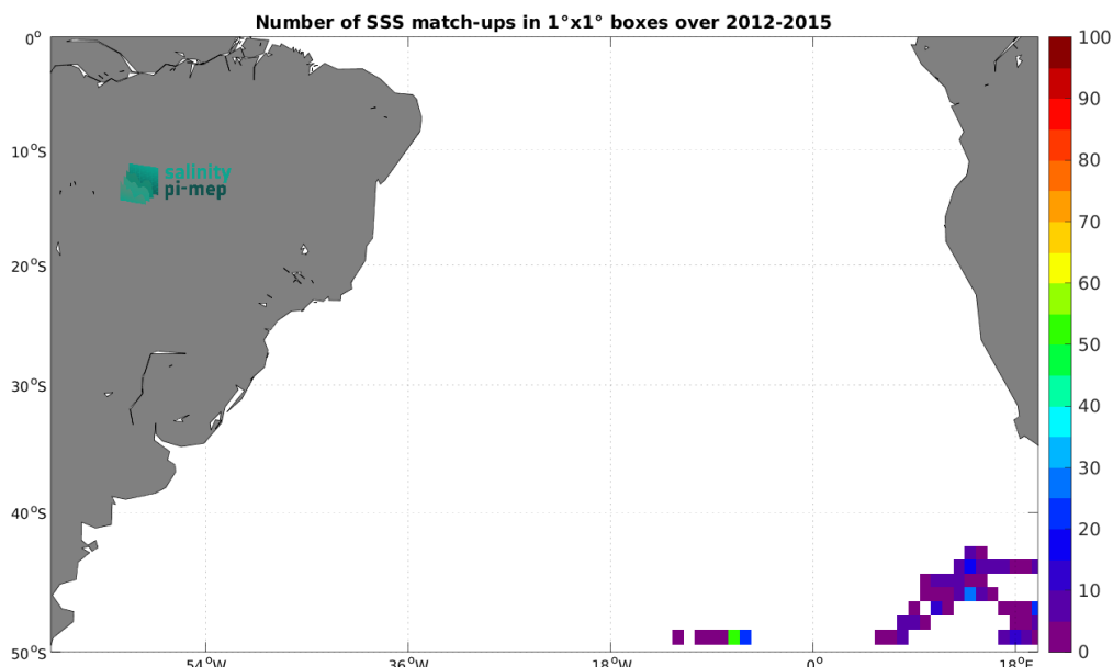
Figure 5: Number of SSS match-ups between Marine mammals SSS and the Aquarius SSS L3 OR v5 - 7-Day running - Rain mask (NASA-GSFC) SSS product for the South Atlantic Ocean Pi-MEP region over 1^\circ \times 1^\circ boxes and for the full satellite product period.
