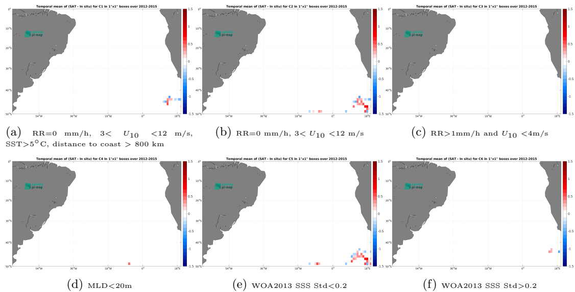
Figure 14: Temporal mean gridded over spatial boxes of size 1^\circ \times 1^\circ of \Delta SSS (Aquarius SSS L3 OR v5 - 7-Day running - Rain mask (NASA-GSFC) - Marine mammals) for 6 different subdatasets corresponding to:RR=0 mm/h, 3 < U_{10} < 12 m/s, SST > 5^\circ\text{C} , distance to coast > 800 km (a), RR=0 mm/h, 3 < U_{10} < 12 m/s (b), RR > 1 mm/h and U_{10} < 4 m/s (c),MLD < 20 m (d),WOA2013 SSS Std < 0.2 (e),WOA2013 SSS Std > 0.2 (f).
