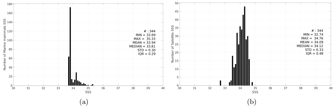
Figure 3: Histograms of SSS from Marine mammals (a) and Aquarius SSS L3 OR v5 - 7-Day running - Rain mask (NASA-GSFC) (b) considering all match-up pairs per bins of 0.1 over the South Atlantic Ocean Pi-MEP region and for the full satellite product period.
