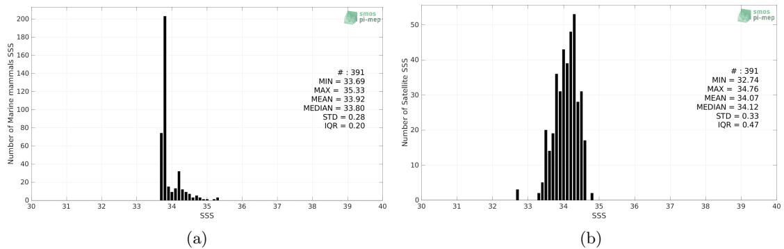
Figure 2: Histograms of SSS from Marine mammals (a) and Aquarius SSS L3 OR v5 - 7-Day running - Rain mask (NASA-GSFC) (b) considering all match-up pairs per bins of 0.1 over the South Atlantic Ocean Pi-MEP region and for the full satellite product period.
