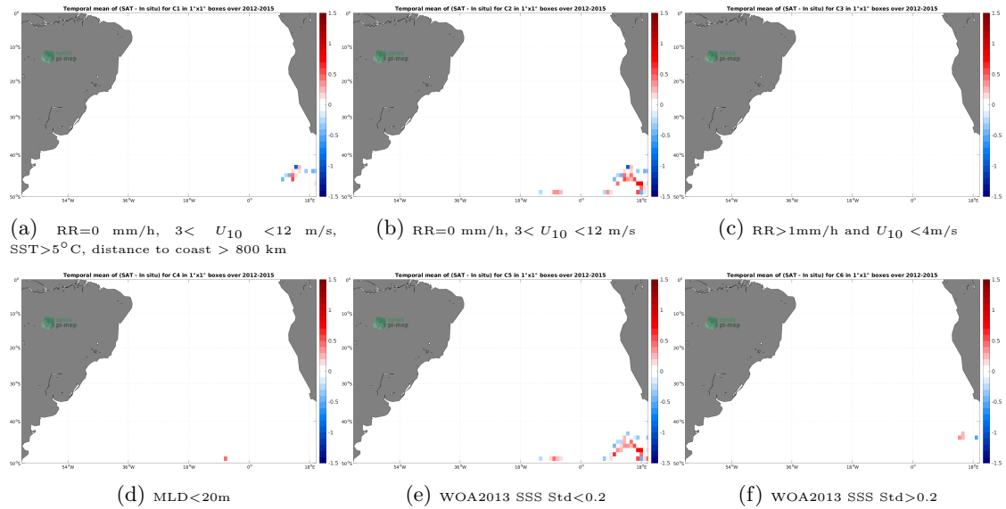
Figure 12: Temporal mean gridded over spatial boxes of size 1^{\circ}\times 1^{\circ} of \Delta\text{SSS} (Aquarius SSS L3 OR v5 - 7-Day running - Rain mask (NASA-GSFC) - Marine mammals) for 6 different subdatasets corresponding to:RR=0 mm/h, 3 < U_{10} < 12 m/s, SST >5^{\circ}\text{C} , distance to coast > 800 km (a), RR=0 mm/h, 3 < U_{10} < 12 m/s (b), RR >1 mm/h and U_{10} < 4 m/s (c),MLD <20 m (d),WOA2013 SSS Std <0.2 (e),WOA2013 SSS Std >0.2 (f).
