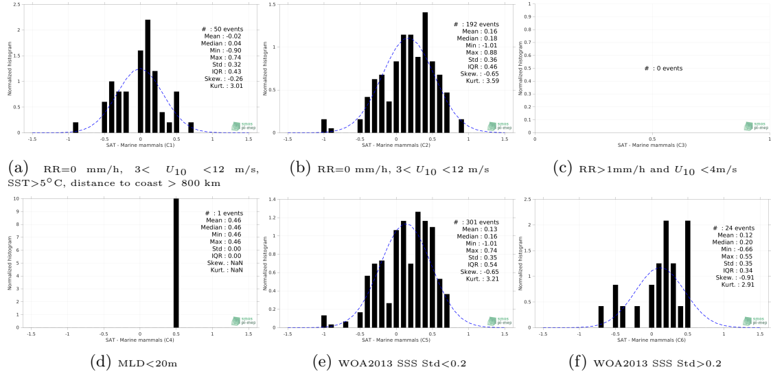
Figure 13: Normalized histogram of \Delta SSS (Aquarius SSS L3 OR v5 - 7-Day running - Rain mask (NASA-GSFC) - Marine mammals) for 6 different subdatasets corresponding to: RR=0 mm/h, 3 < U_{10} < 12 m/s, SST>5°C, distance to coast > 800 km (a), RR=0 mm/h, 3 < U_{10} < 12 m/s (b), RR>1mm/h and U_{10} < 4 m/s (c), MLD<20m (d), WOA2013 SSS Std<0.2 (e), WOA2013 SSS Std>0.2 (f).
