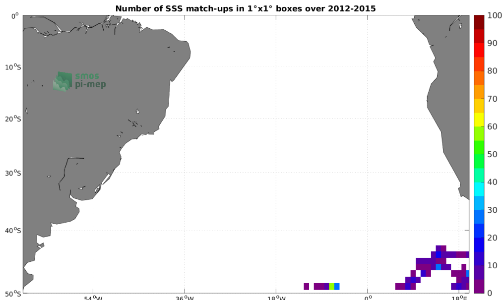
Figure 4: Number of SSS match-ups between Marine mammals SSS and the Aquarius SSS L3 OR v5 - 7-Day running - Rain mask (NASA-GSFC) SSS product for the South Atlantic Ocean Pi-MEP region over 1^\circ \times 1^\circ boxes and for the full satellite product period.
