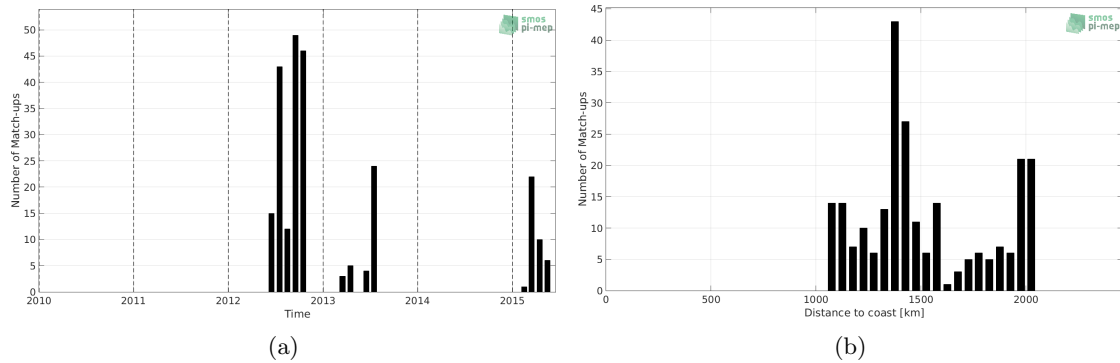
Figure 1: Number of match-ups between Sea mammals and Aquarius-L3-OR-V5-7DAY-RUNNING-RAIN-MASK-1DEG SSS as a function of time (a) and as function of the distance to coast (b) over the South Atlantic Ocean Pi-MEP region and for the full satellite product period.
