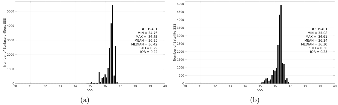
Figure 3: Histograms of SSS from Surface drifters (a) and Aquarius SSS L3 OR v5 - 7-Day running - Rain mask (NASA-GSFC) (b) considering all match-up pairs per bins of 0.1 over the South Atlantic Ocean Pi-MEP region and for the full satellite product period.
