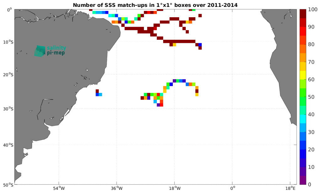
Figure 4: Number of SSS match-ups between Surface drifters SSS and the Aquarius SSS L3 OR v5 - 7-Day running - Rain mask (NASA-GSFC) SSS product for the South Atlantic Ocean Pi-MEP region over 1^\circ \times 1^\circ boxes and for the full satellite product period.
