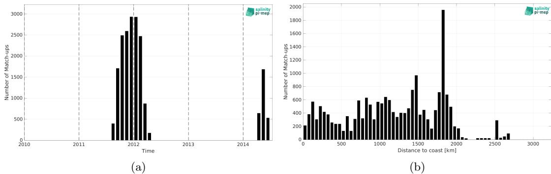
Figure 2: Number of match-ups between Surface drifters and Aquarius SSS L3 OR v5 - 7-Day running - Rain mask (NASA-GSFC) SSS as a function of time (a) and as function of the distance to coast (b) over the South Atlantic Ocean Pi-MEP region and for the full satellite product period.
