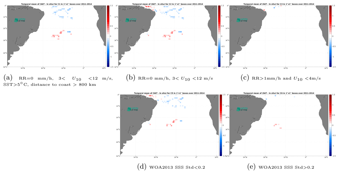
Figure 13: Temporal mean gridded over spatial boxes of size 1^\circ \times 1^\circ of \Delta SSS (Aquarius SSS L3 OR v5 - 7-Day running - Rain mask (NASA-GSFC) - Surface drifters) for 5 different subdatasets corresponding to:RR=0 mm/h, 3 < U_{10} < 12 m/s, SST >5^\circ\text{C} , distance to coast > 800 km (a), RR=0 mm/h, 3 < U_{10} < 12 m/s (b), RR >1 mm/h and U_{10} < 4 m/s (c), WOA2013 SSS Std <0.2 (d), WOA2013 SSS Std >0.2 (e).
