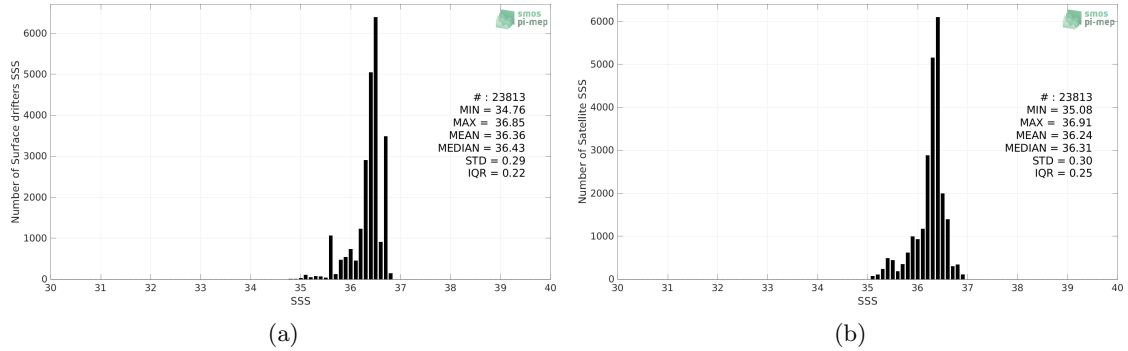
Figure 2: Histograms of SSS from Surface drifters (a) and Aquarius SSS L3 OR v5 - 7-Day running - Rain mask (NASA-GSFC) (b) considering all match-up pairs per bins of 0.1 over the South Atlantic Ocean Pi-MEP region and for the full satellite product period.
