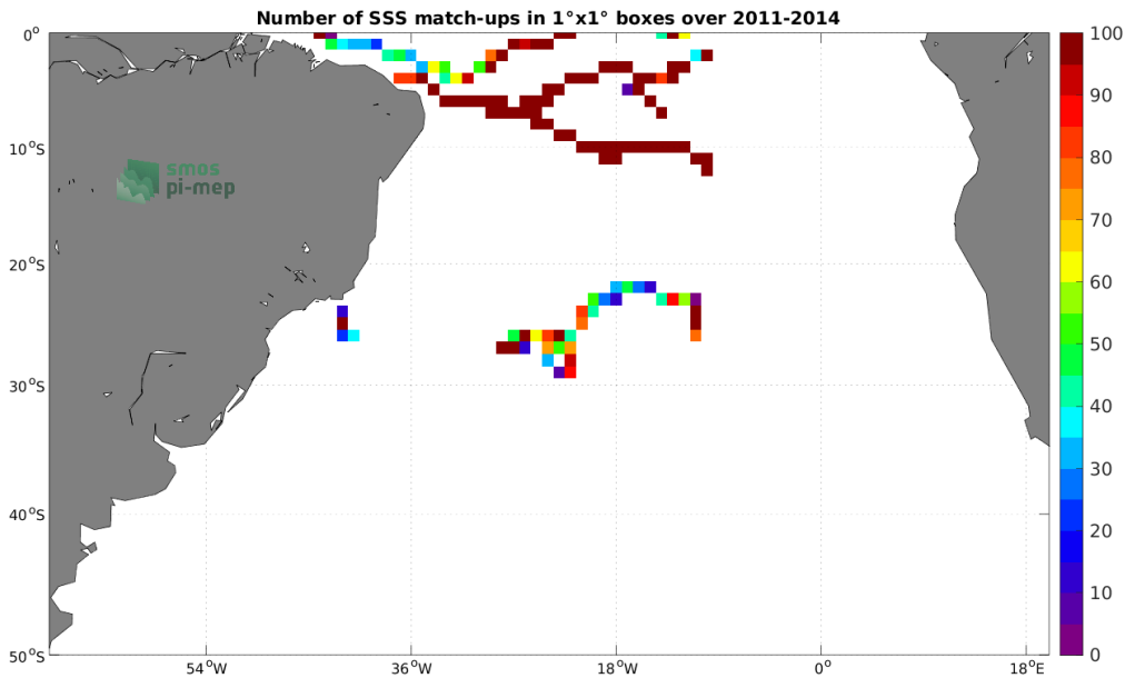
Figure 3: Number of SSS match-ups between Surface drifters SSS and the Aquarius SSS L3 OR v5 - 7-Day running - Rain mask (NASA-GSFC) SSS product for the South Atlantic Ocean Pi-MEP region over 1^\circ \times 1^\circ boxes and for the full satellite product period.
