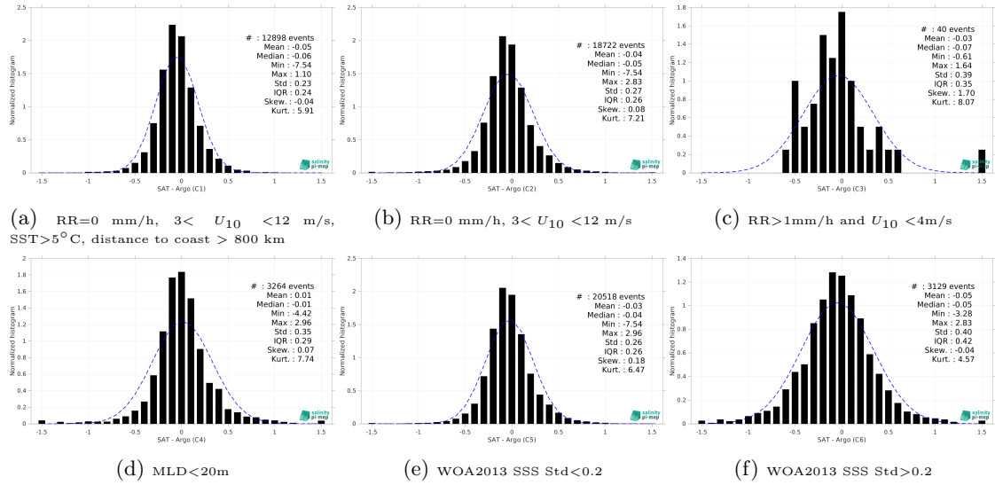
Figure 15: Normalized histogram of \Delta SSS (Aquarius SSS L3 OR v5 - 7-Day running - Rain mask (NASA-GSFC) - Argo) for 6 different subdatasets corresponding to: RR=0 mm/h, 3 < U_{10} < 12 m/s, SST > 5°C, distance to coast > 800 km (a), RR=0 mm/h, 3 < U_{10} < 12 m/s (b), RR > 1mm/h and U_{10} < 4 m/s (c), MLD < 20m (d), WOA2013 SSS Std < 0.2 (e), WOA2013 SSS Std > 0.2 (f).
