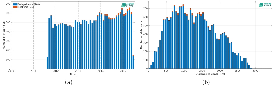
Figure 2: Number of match-ups between Argo and Aquarius SSS L3 OR v5 - 7-Day running - Rain mask (NASA-GSFC) SSS as a function of time (a) and as function of the distance to coast (b) over the South Atlantic Ocean Pi-MEP region and for the full satellite product period.
