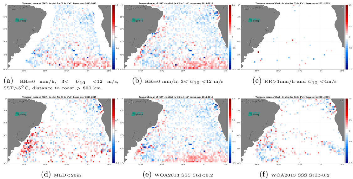
Figure 14: Temporal mean gridded over spatial boxes of size 1^\circ \times 1^\circ of \Delta SSS (Aquarius SSS L3 OR v5 - 7-Day running - Rain mask (NASA-GSFC) - Argo) for 6 different subdatasets corresponding to:RR=0 mm/h, 3 < U_{10} < 12 m/s, SST >5^\circ C, distance to coast > 800 km (a), RR=0 mm/h, 3 < U_{10} < 12 m/s (b), RR >1 mm/h and U_{10} < 4 m/s (c),MLD <20 m (d),WOA2013 SSS Std <0.2 (e),WOA2013 SSS Std >0.2 (f).
