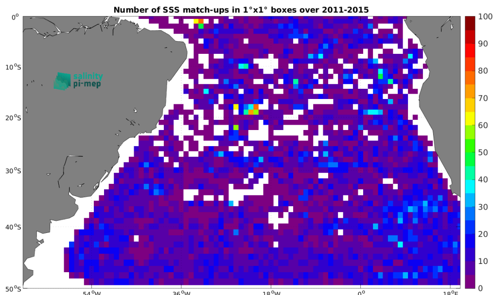
Figure 5: Number of SSS match-ups between Argo SSS and the Aquarius SSS L3 OR v5 - 7-Day running - Rain mask (NASA-GSFC) SSS product for the South Atlantic Ocean Pi-MEP region over 1^\circ \times 1^\circ boxes and for the full satellite product period.
