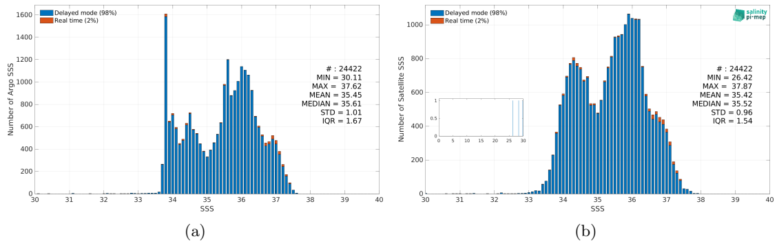
Figure 3: Histograms of SSS from Argo (a) and Aquarius SSS L3 OR v5 - 7-Day running - Rain mask (NASA-GSFC) (b) considering all match-up pairs per bins of 0.1 over the South Atlantic Ocean Pi-MEP region and for the full satellite product period.
