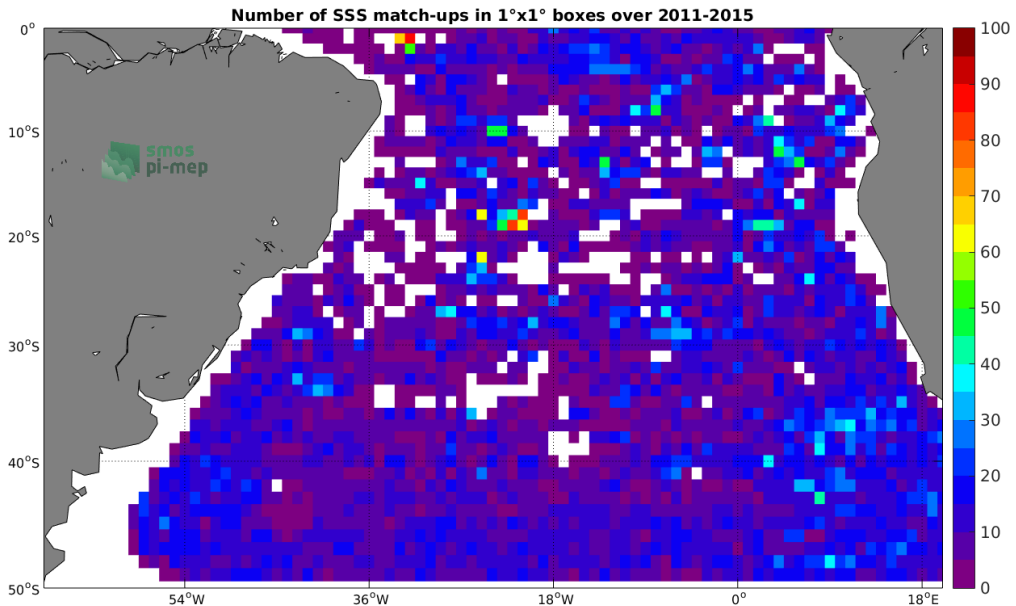
Figure 4: Number of SSS match-ups between Argo SSS and the Aquarius-L3-OR-V5-7DAY-RUNNING-RAIN-MASK-1DEG SSS product for the South Atlantic Ocean Pi-MEP region over 1^\circ \times 1^\circ boxes and for the full satellite product period.
