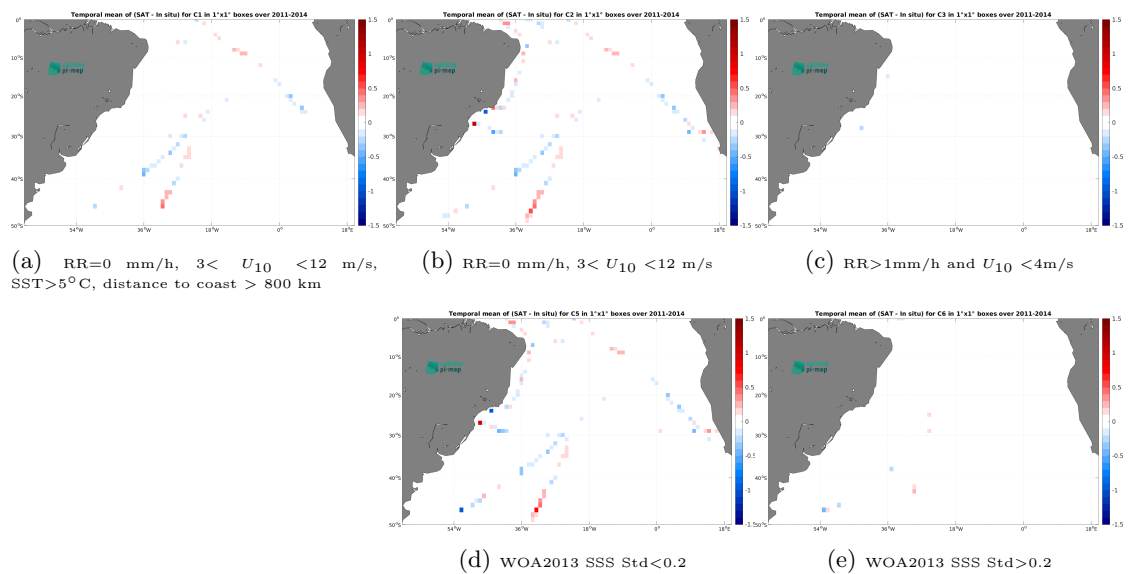
Figure 14: Temporal mean gridded over spatial boxes of size 1^\circ \times 1^\circ of \Delta SSS (Aquarius SSS L3 OR v5 - Monthly (NASA-GSFC) - TSG (SAMOS)) for 5 different subdatasets corresponding to:RR=0 mm/h, 3 < U_{10} < 12 m/s, SST >5^\circ\text{C} , distance to coast > 800 km (a), RR=0 mm/h, 3 < U_{10} < 12 m/s (b), RR >1 mm/h and U_{10} < 4 m/s (c), WOA2013 SSS Std <0.2 (d), WOA2013 SSS Std >0.2 (e).
