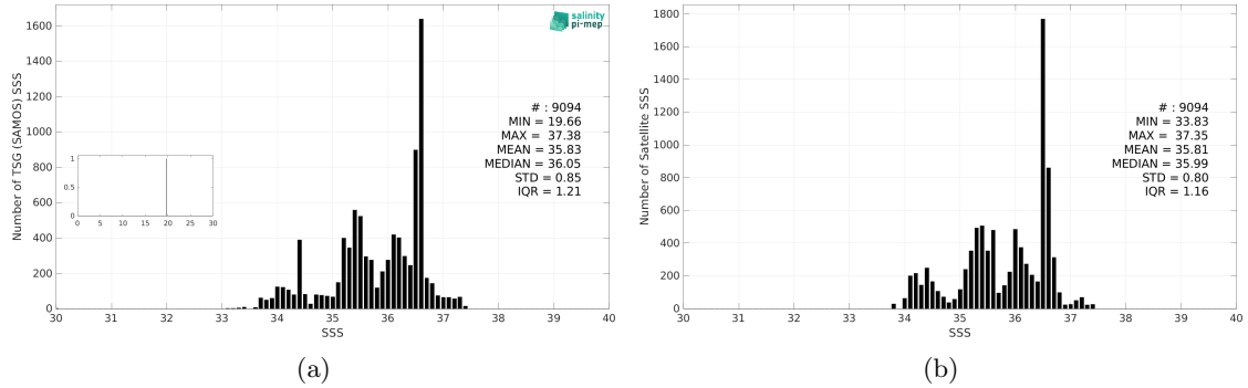
Figure 3: Histograms of SSS from TSG (SAMOS) (a) and Aquarius SSS L3 OR v5 - Monthly (NASA-GSFC) (b) considering all match-up pairs per bins of 0.1 over the South Atlantic Ocean Pi-MEP region and for the full satellite product period.
