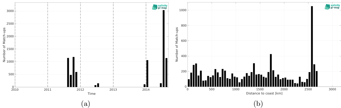
Figure 2: Number of match-ups between TSG (SAMOS) and Aquarius SSS L3 OR v5 - Monthly (NASA-GSFC) SSS as a function of time (a) and as function of the distance to coast (b) over the South Atlantic Ocean Pi-MEP region and for the full satellite product period.
