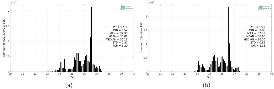
Figure 2: Histograms of SSS from TSG (SAMOS) (a) and Aquarius SSS L3 OR v5 - Monthly (NASA-GSFC) (b) considering all match-up pairs per bins of 0.1 over the South Atlantic Ocean Pi-MEP region and for the full satellite product period.
