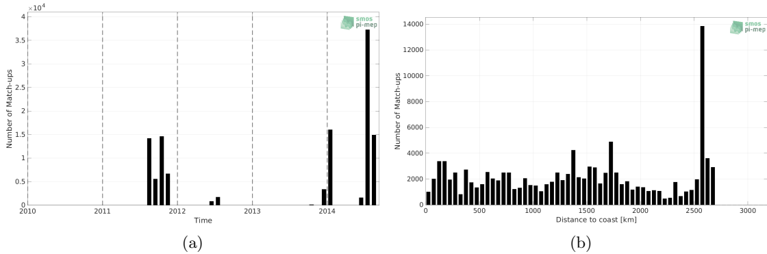
Figure 1: Number of match-ups between TSG (SAMOS) and Aquarius SSS L3 OR v5 - Monthly (NASA-GSFC) SSS as a function of time (a) and as function of the distance to coast (b) over the South Atlantic Ocean Pi-MEP region and for the full satellite product period.
