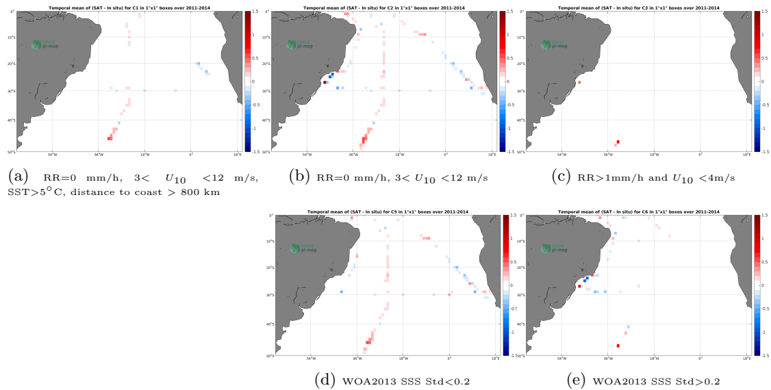
Figure 12: Temporal mean gridded over spatial boxes of size 1^\circ \times 1^\circ of \Delta SSS (Aquarius-L3-OR-V5-MONTHLY-1DEG - TSG-SAMOS) for 5 different subdatasets corresponding to:RR=0 mm/h, 3 < U_{10} < 12 m/s, SST >5^\circ\text{C} , distance to coast > 800 km (a), RR=0 mm/h, 3 < U_{10} < 12 m/s (b), RR >1 mm/h and U_{10} < 4 m/s (c), WOA2013 SSS Std <0.2 (d), WOA2013 SSS Std >0.2 (e).
