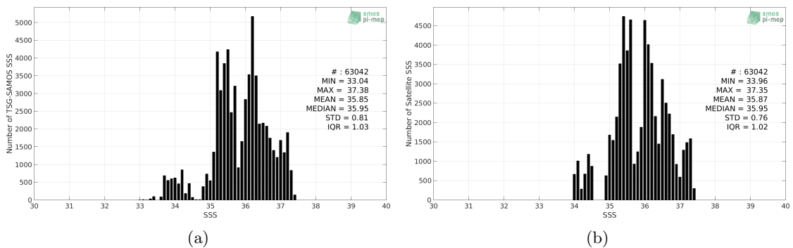
Figure 2: Histograms of SSS from TSG-SAMOS (a) and Aquarius-L3-OR-V5-MONTHLY-1DEG (b) considering all match-up pairs per bins of 0.1 over the South Atlantic Ocean Pi-MEP region and for the full satellite product period.
