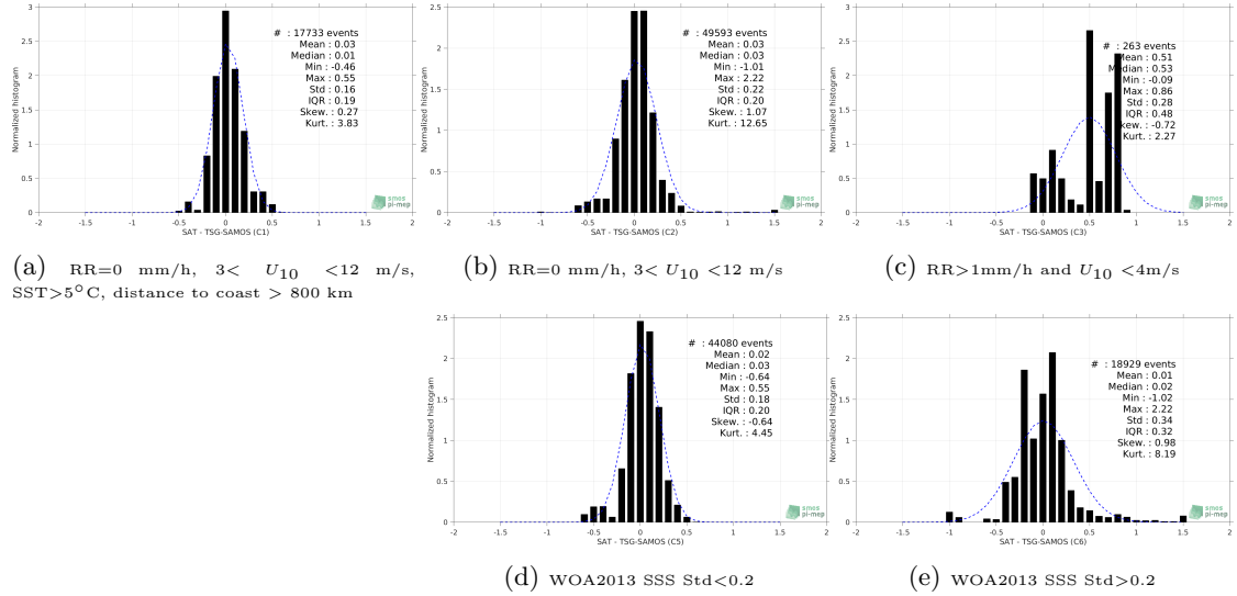
Figure 13: Normalized histogram of \Delta SSS (Aquarius-L3-OR-V5-MONTHLY-1DEG - TSG-SAMOS) for 5 different subdatasets corresponding to: RR=0 mm/h, 3 < U_{10} < 12 m/s, SST > 5°C, distance to coast > 800 km (a), RR=0 mm/h, 3 < U_{10} < 12 m/s (b), RR > 1mm/h and U_{10} < 4 m/s (c), WOA2013 SSS Std < 0.2 (d), WOA2013 SSS Std > 0.2 (e).
