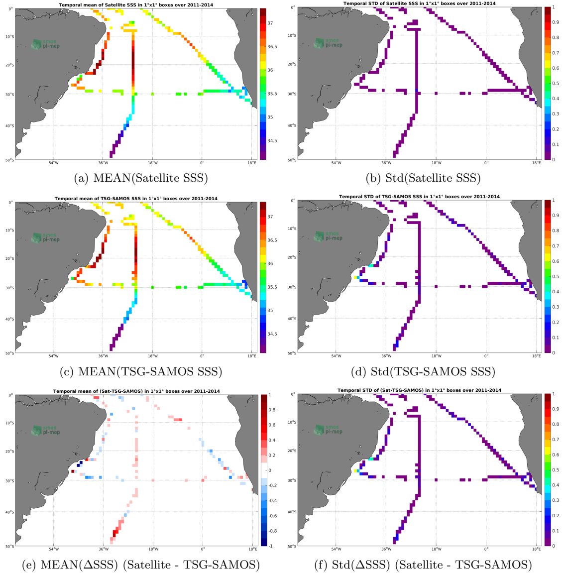
Figure 6: Temporal mean (left) and Std (right) of SSS from Aquarius-L3-OR-V5-MONTHLY-1DEG (top), TSG-SAMOS (middle), and of \Delta SSS (Satellite - TSG-SAMOS). Only match-up pairs are used to generate these maps.
