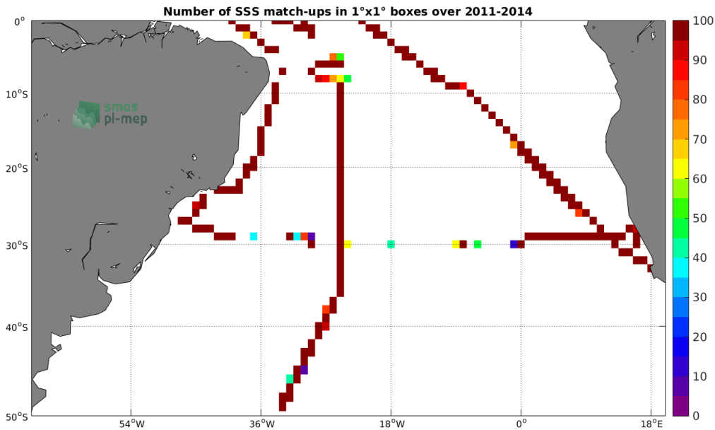
Figure 4: Number of SSS match-ups between TSG-SAMOS SSS and the Aquarius-L3-OR-V5-MONTHLY-1DEG SSS product for the South Atlantic Ocean Pi-MEP region over 1^{\circ} \times 1^{\circ} boxes and for the full satellite product period.
