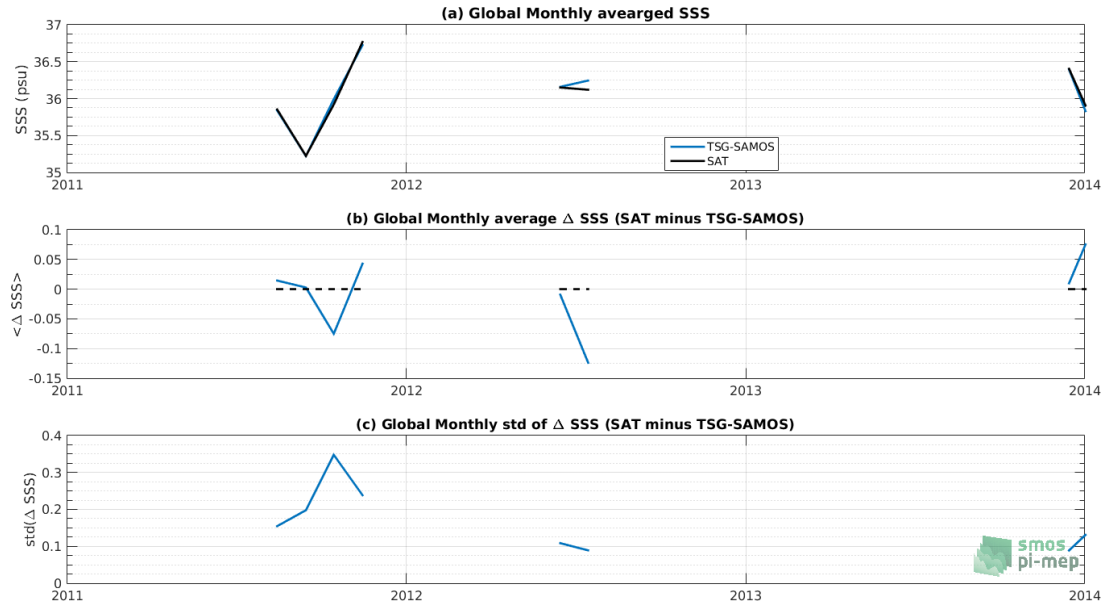
Figure 7: Time series of the monthly averaged mean SSS (top), mean \Delta SSS (Satellite - TSG-SAMOS) and Std of \Delta SSS (Satellite - TSG-SAMOS) over the South Atlantic Ocean Pi-MEP region considering all match-ups collected by the Pi-MEP platform.
