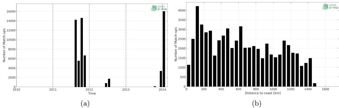
Figure 1: Number of match-ups between TSG-SAMOS and Aquarius-L3-OR-V5-MONTHLY-1DEG SSS as a function of time (a) and as function of the distance to coast (b) over the South Atlantic Ocean Pi-MEP region and for the full satellite product period.
