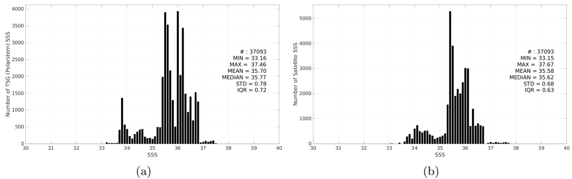
Figure 3: Histograms of SSS from TSG (Polarstern) (a) and Aquarius SSS L3 OR v5 - Monthly (NASA-GSFC) (b) considering all match-up pairs per bins of 0.1 over the South Atlantic Ocean Pi-MEP region and for the full satellite product period.
