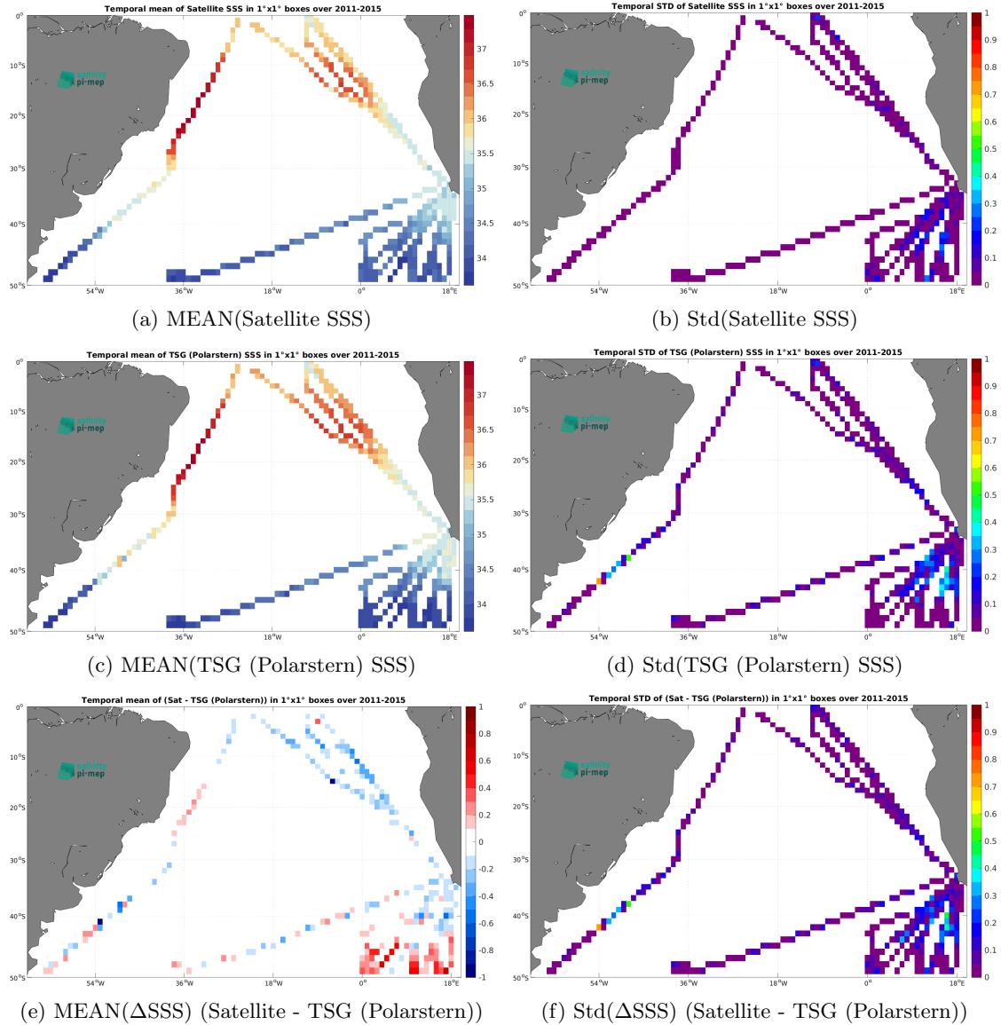
Figure 7: Temporal mean (left) and Std (right) of SSS from Aquarius SSS L3 OR v5 - Monthly (NASA-GSFC) (top), TSG (Polarstern) (middle), and of \Delta SSS (Satellite - TSG (Polarstern)). Only match-up pairs are used to generate these maps.
