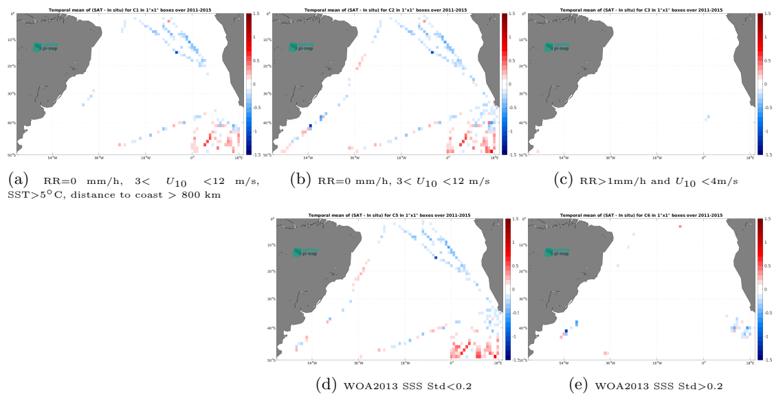
Figure 14: Temporal mean gridded over spatial boxes of size 1^\circ \times 1^\circ of \Delta SSS (Aquarius SSS L3 OR v5 - Monthly (NASA-GSFC) - TSG (Polarstern)) for 5 different subdatasets corresponding to:RR=0 mm/h, 3 < U_{10} < 12 m/s, SST >5^\circ\text{C} , distance to coast > 800 km (a), RR=0 mm/h, 3 < U_{10} < 12 m/s (b), RR >1 mm/h and U_{10} < 4 m/s (c), WOA2013 SSS Std <0.2 (d), WOA2013 SSS Std >0.2 (e).
