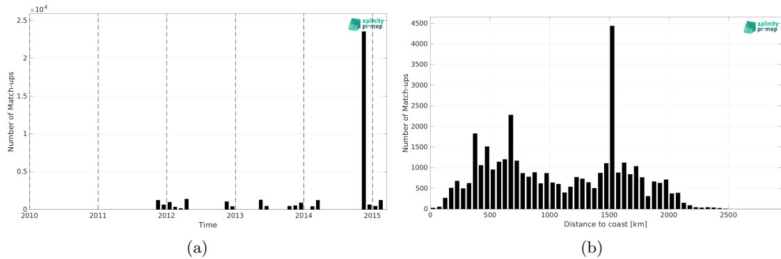
Figure 2: Number of match-ups between TSG (Polarstern) and Aquarius SSS L3 OR v5 - Monthly (NASA-GSFC) SSS as a function of time (a) and as function of the distance to coast (b) over the South Atlantic Ocean Pi-MEP region and for the full satellite product period.
