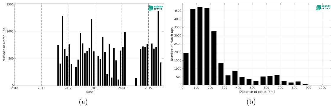
Figure 2: Number of match-ups between TSG (LEGOS-DM) and Aquarius SSS L3 OR v5 - Monthly (NASA-GSFC) SSS as a function of time (a) and as function of the distance to coast (b) over the South Atlantic Ocean Pi-MEP region and for the full satellite product period.
