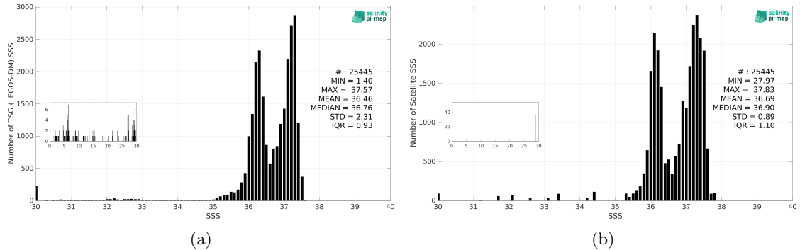
Figure 3: Histograms of SSS from TSG (LEGOS-DM) (a) and Aquarius SSS L3 OR v5 - Monthly (NASA-GSFC) (b) considering all match-up pairs per bins of 0.1 over the South Atlantic Ocean Pi-MEP region and for the full satellite product period.
