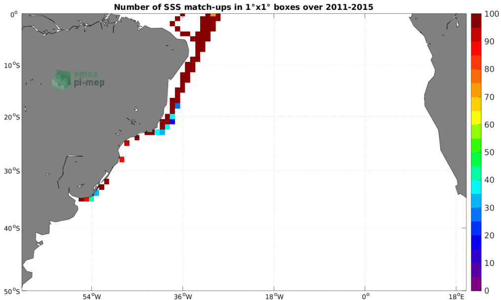
Figure 4: Number of SSS match-ups between TSG (LEGOS-DM) SSS and the Aquarius SSS L3 OR v5 - Monthly (NASA-GSFC) SSS product for the South Atlantic Ocean Pi-MEP region over 1^\circ \times 1^\circ boxes and for the full satellite product period.
