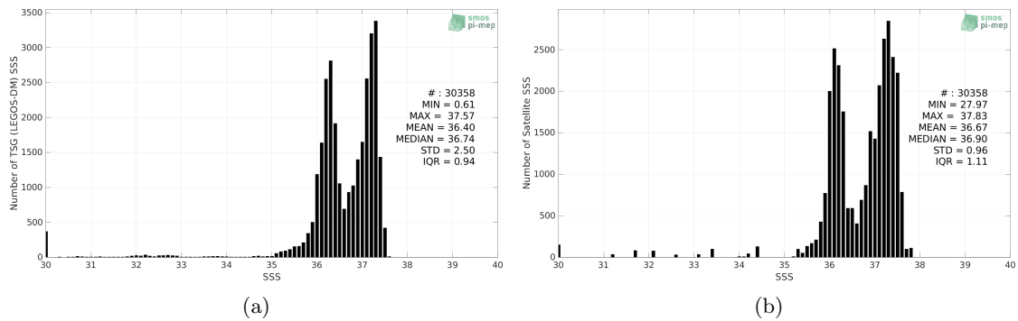
Figure 2: Histograms of SSS from TSG (LEGOS-DM) (a) and Aquarius SSS L3 OR v5 - Monthly (NASA-GSFC) (b) considering all match-up pairs per bins of 0.1 over the South Atlantic Ocean Pi-MEP region and for the full satellite product period.
