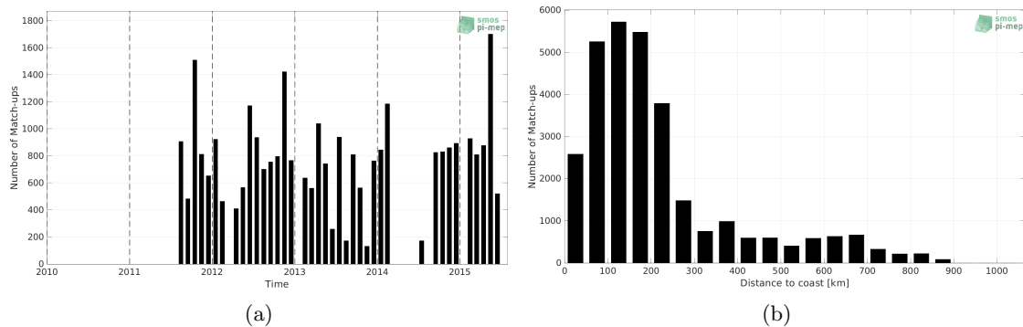
Figure 1: Number of match-ups between TSG (LEGOS-DM) and Aquarius SSS L3 OR v5 - Monthly (NASA-GSFC) SSS as a function of time (a) and as function of the distance to coast (b) over the South Atlantic Ocean Pi-MEP region and for the full satellite product period.
