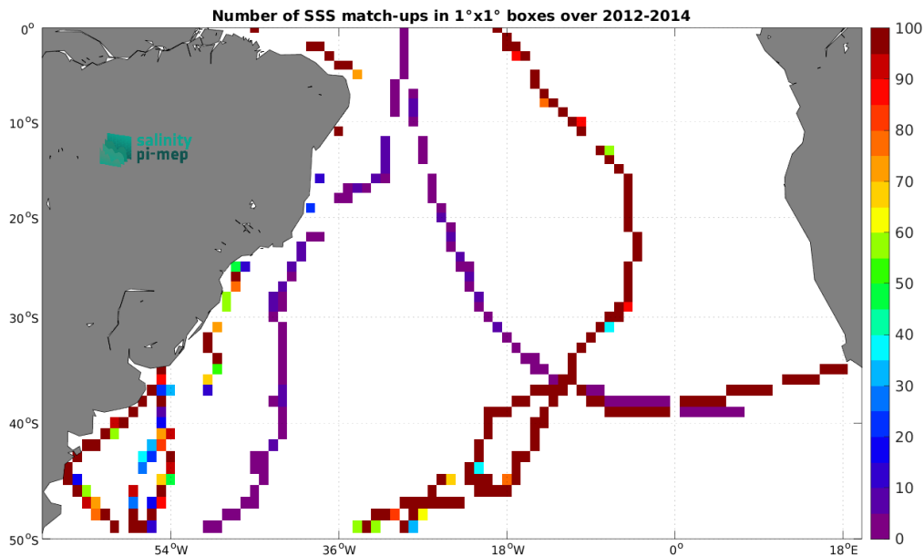
Figure 5: Number of SSS match-ups between TSG (GOSUD-Sailing-ship) SSS and the Aquarius SSS L3 OR v5 - Monthly (NASA-GSFC) SSS product for the South Atlantic Ocean Pi-MEP region over 1^\circ \times 1^\circ boxes and for the full satellite product period.
