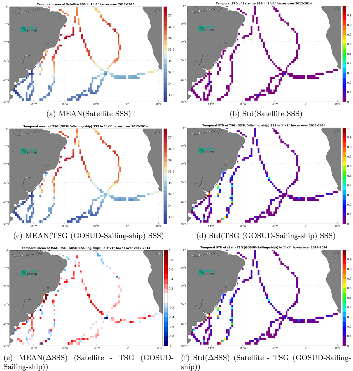
Figure 7: Temporal mean (left) and Std (right) of SSS from Aquarius SSS L3 OR v5 - Monthly (NASA-GSFC) (top), TSG (GOSUD-Sailing-ship) (middle), and of \Delta SSS (Satellite - TSG (GOSUD-Sailing-ship)). Only match-up pairs are used to generate these maps.
