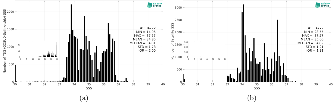
Figure 3: Histograms of SSS from TSG (GOSUD-Sailing-ship) (a) and Aquarius SSS L3 OR v5 - Monthly (NASA-GSFC) (b) considering all match-up pairs per bins of 0.1 over the South Atlantic Ocean Pi-MEP region and for the full satellite product period.
