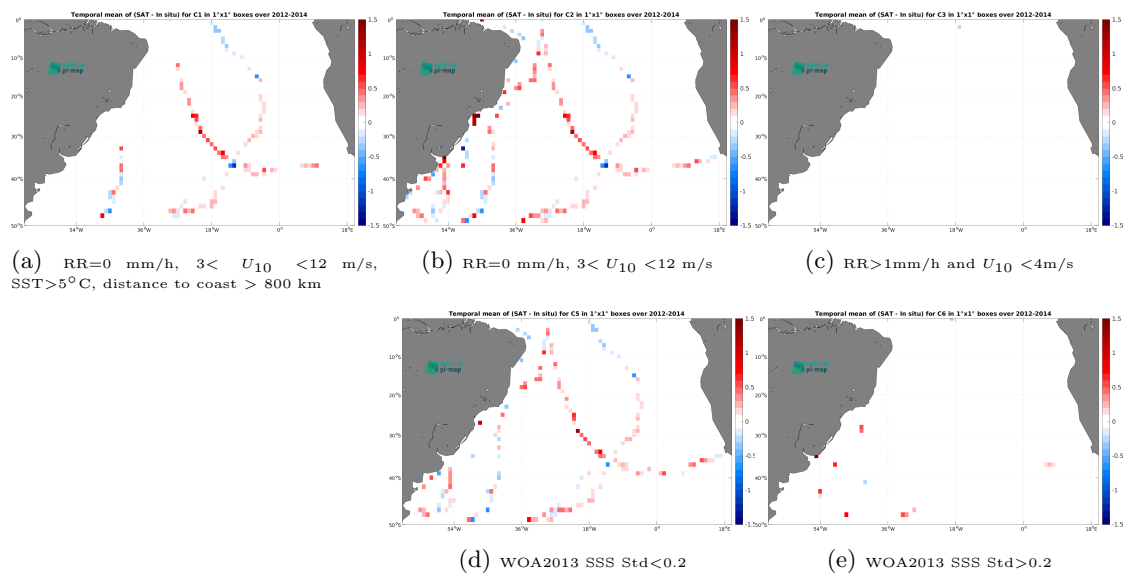
Figure 14: Temporal mean gridded over spatial boxes of size 1^\circ \times 1^\circ of \Delta\text{SSS} (Aquarius SSS L3 OR v5 - Monthly (NASA-GSFC) - TSG (GOSUD-Sailing-ship)) for 5 different subdatasets corresponding to:RR=0 mm/h, 3 < U_{10} < 12 m/s, SST >5^\circ\text{C} , distance to coast > 800 km (a), RR=0 mm/h, 3 < U_{10} < 12 m/s (b), RR >1 mm/h and U_{10} < 4 m/s (c), WOA2013 SSS Std <0.2 (d), WOA2013 SSS Std >0.2 (e).
