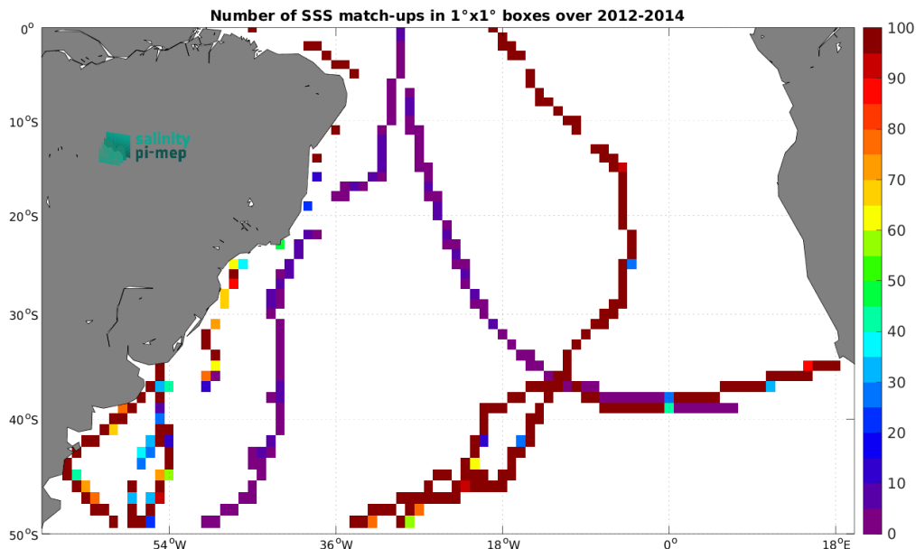
Figure 4: Number of SSS match-ups between TSG (GOSUD-Sailing-ship) SSS and the Aquarius SSS L3 OR v5 - Monthly (NASA-GSFC) SSS product for the South Atlantic Ocean Pi-MEP region over 1^\circ \times 1^\circ boxes and for the full satellite product period.
