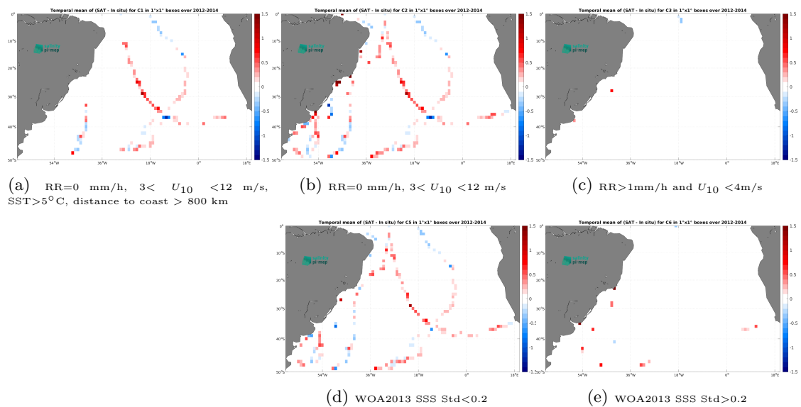
Figure 12: Temporal mean gridded over spatial boxes of size 1^\circ \times 1^\circ of \Delta SSS (Aquarius SSS L3 OR v5 - Monthly (NASA-GSFC) - TSG (GOSUD-Sailing-ship)) for 5 different subdatasets corresponding to:RR=0 mm/h, 3 < U_{10} < 12 m/s, SST >5^\circ\text{C} , distance to coast > 800 km (a), RR=0 mm/h, 3 < U_{10} < 12 m/s (b), RR >1 mm/h and U_{10} < 4 m/s (c), WOA2013 SSS Std <0.2 (d), WOA2013 SSS Std >0.2 (e).
