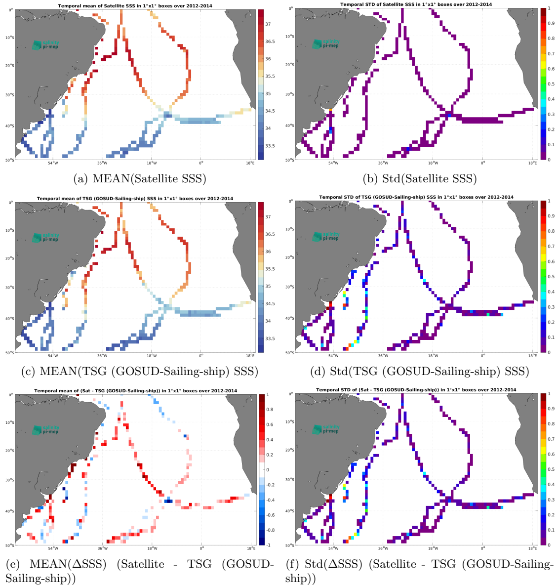
Figure 6: Temporal mean (left) and Std (right) of SSS from Aquarius SSS L3 OR v5 - Monthly (NASA-GSFC) (top), TSG (GOSUD-Sailing-ship) (middle), and of \Delta SSS (Satellite - TSG (GOSUD-Sailing-ship)). Only match-up pairs are used to generate these maps.
