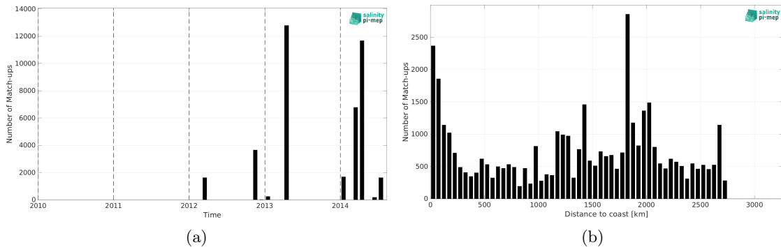
Figure 1: Number of match-ups between TSG (GOSUD-Sailing-ship) and Aquarius SSS L3 OR v5 - Monthly (NASA-GSFC) SSS as a function of time (a) and as function of the distance to coast (b) over the South Atlantic Ocean Pi-MEP region and for the full satellite product period.
