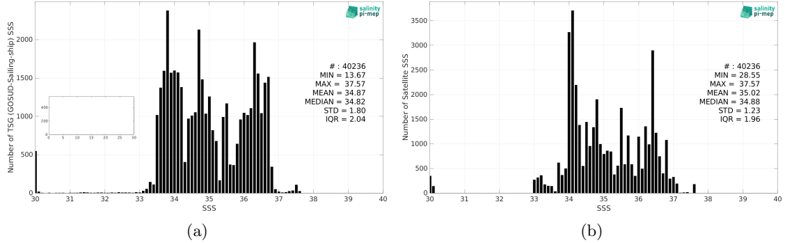
Figure 2: Histograms of SSS from TSG (GOSUD-Sailing-ship) (a) and Aquarius SSS L3 OR v5 - Monthly (NASA-GSFC) (b) considering all match-up pairs per bins of 0.1 over the South Atlantic Ocean Pi-MEP region and for the full satellite product period.
